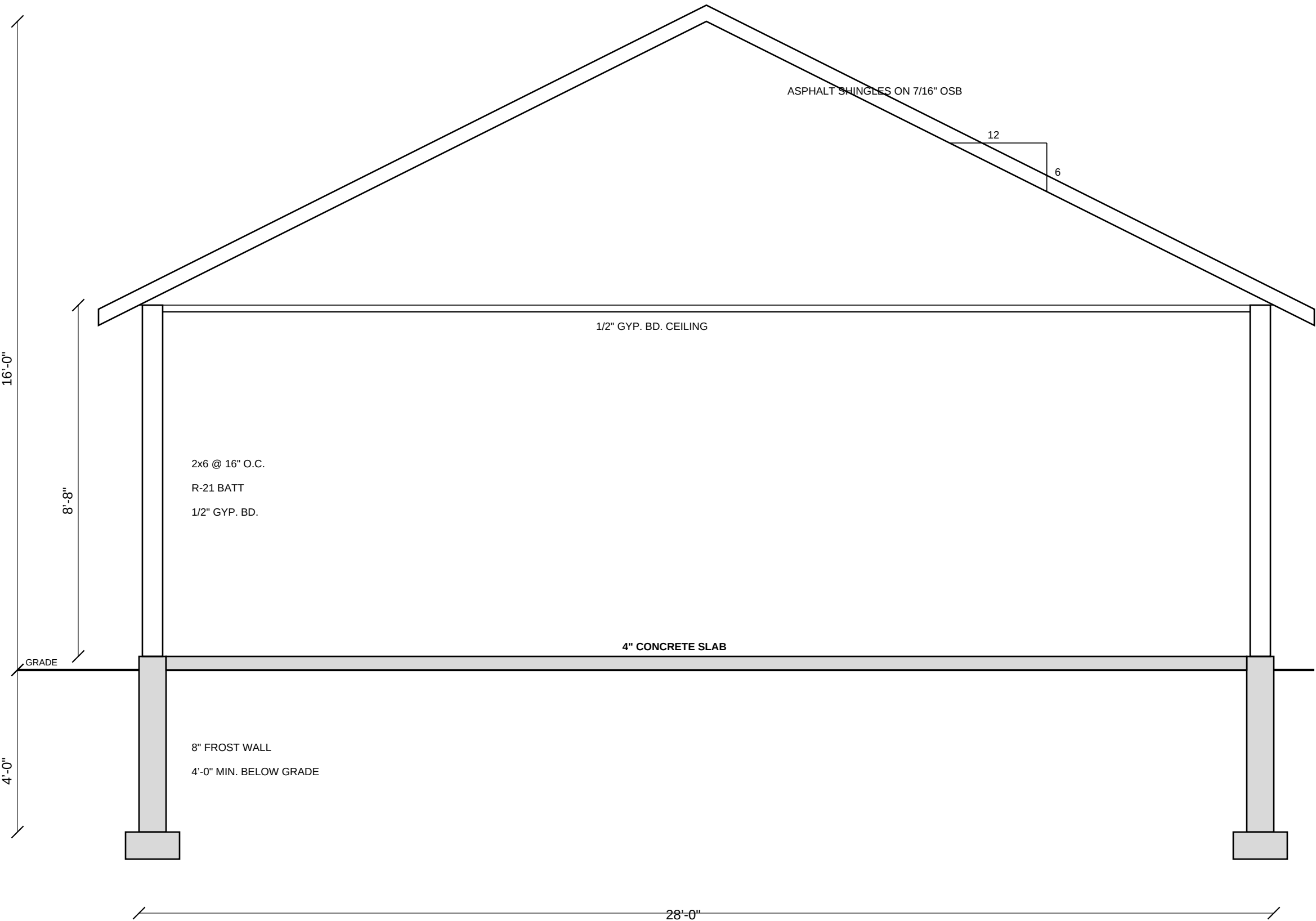
SECTION A 3/8" = 1'-0"
