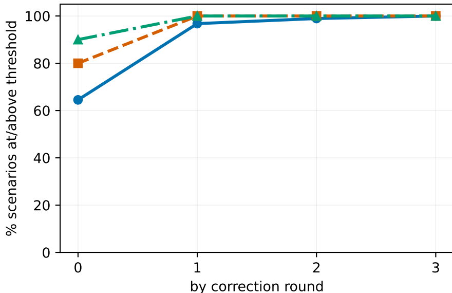
Cumulative convergence
