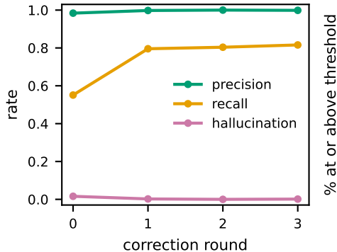
precision / recall / hallucination
