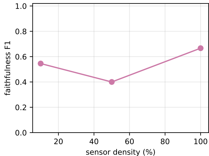
Faithfulness (condition A)
