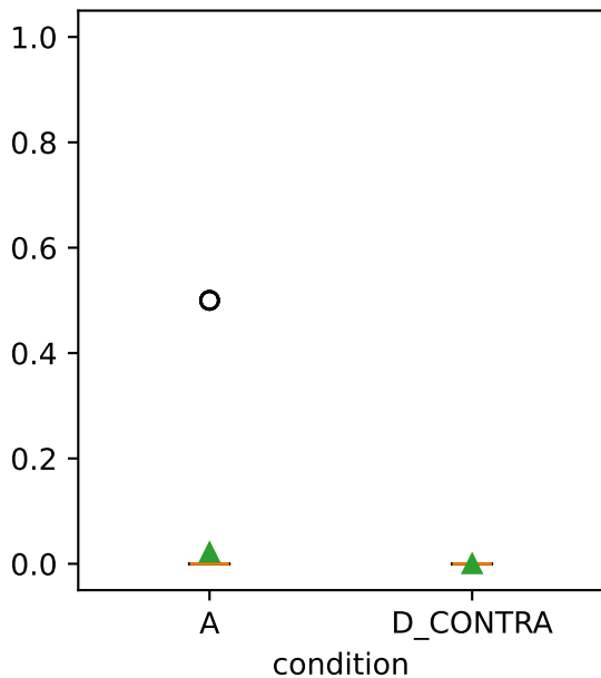
Hallucination rate
