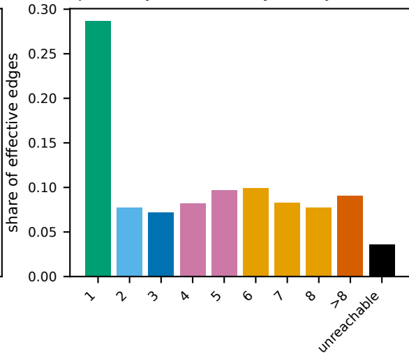
free flow split-half J=0.2256 (beyond-K J=0.1241 )
