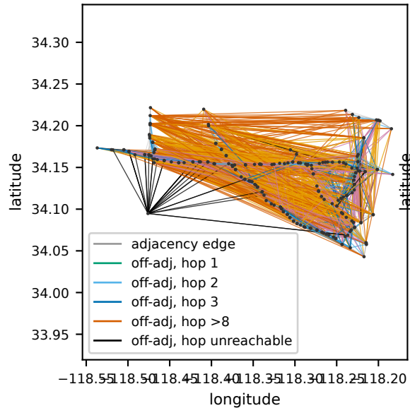
metr la best (1465 off-adjacency of 1656) metr la best epoch34 ARCHIVE (1530 off-adjacency of 1656) metr la fusion best (1423 off-adjacency of 1656)
