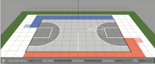
FIGURE V: GAZEBO SIMULATION
