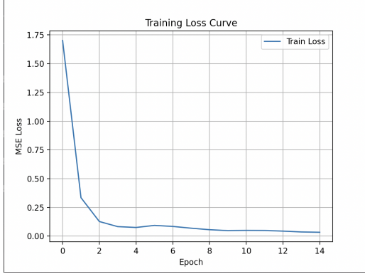
FIGURE VIII: LOSS CURVE
