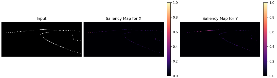
FIGURE X: SALIENCY MAPS
