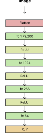
FIGURE II: FLOW DIAGRAM
