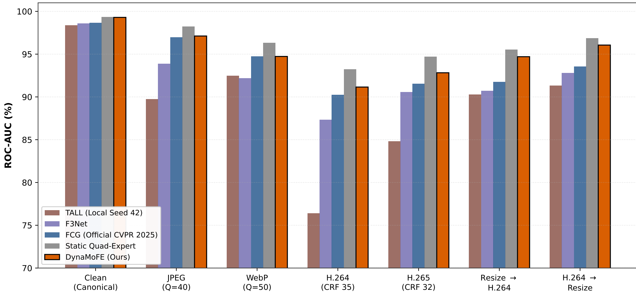
Matched Deepfake Detection Performance Across 7 Transmission Codec Environments
