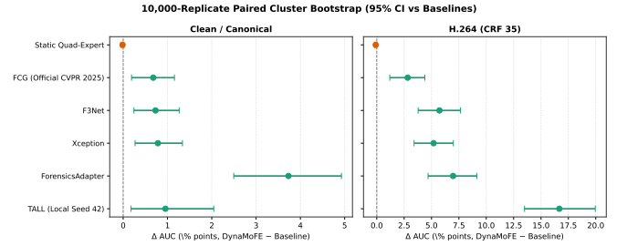
Fig. 3. 10,000-Replicate Paired Cluster Bootstrap Results (95% CI). Difference in AUC points (DynaMoFE residual minus baseline) across 70 source clusters on canonical clean video and H.264 CRF-35.
