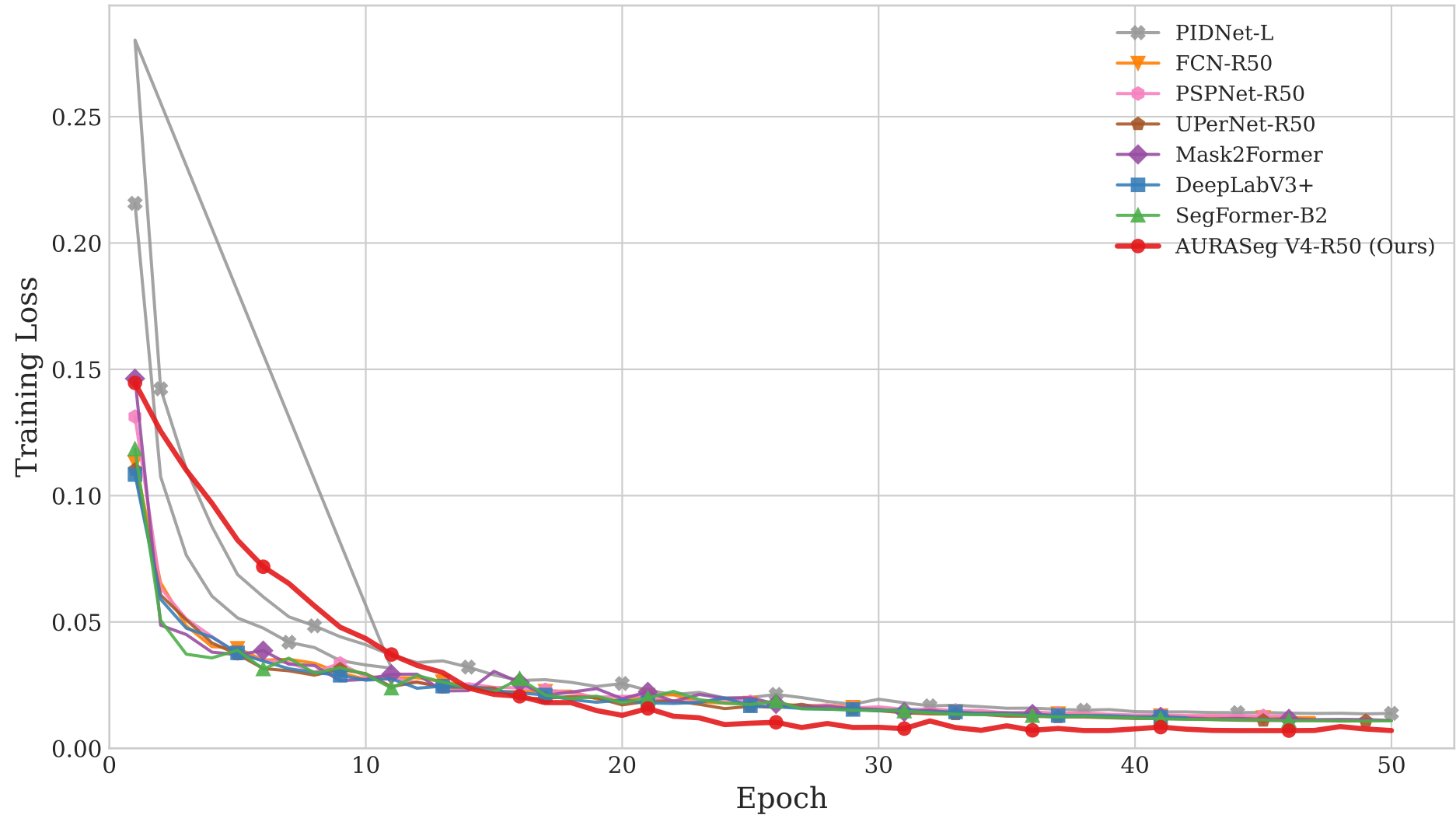
Training Loss Convergence
