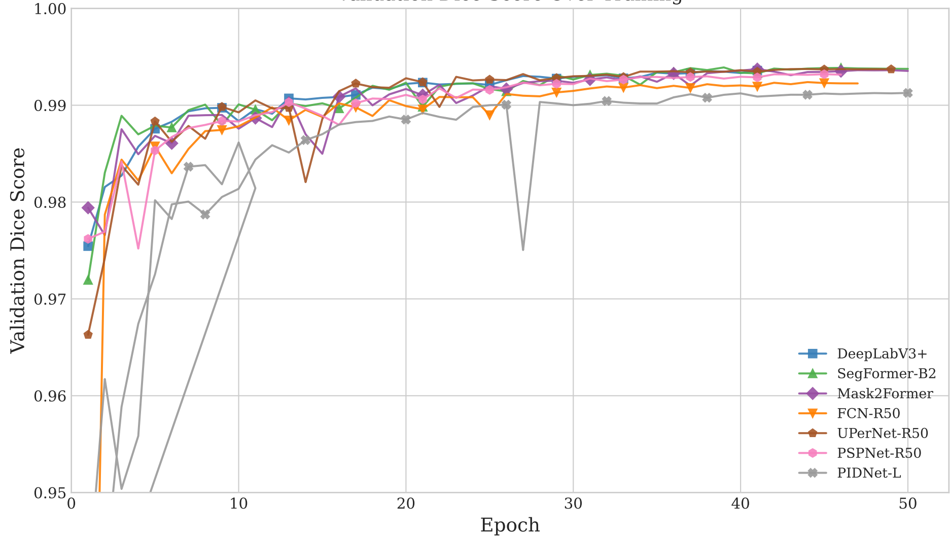
Validation Dice Score Over Training
