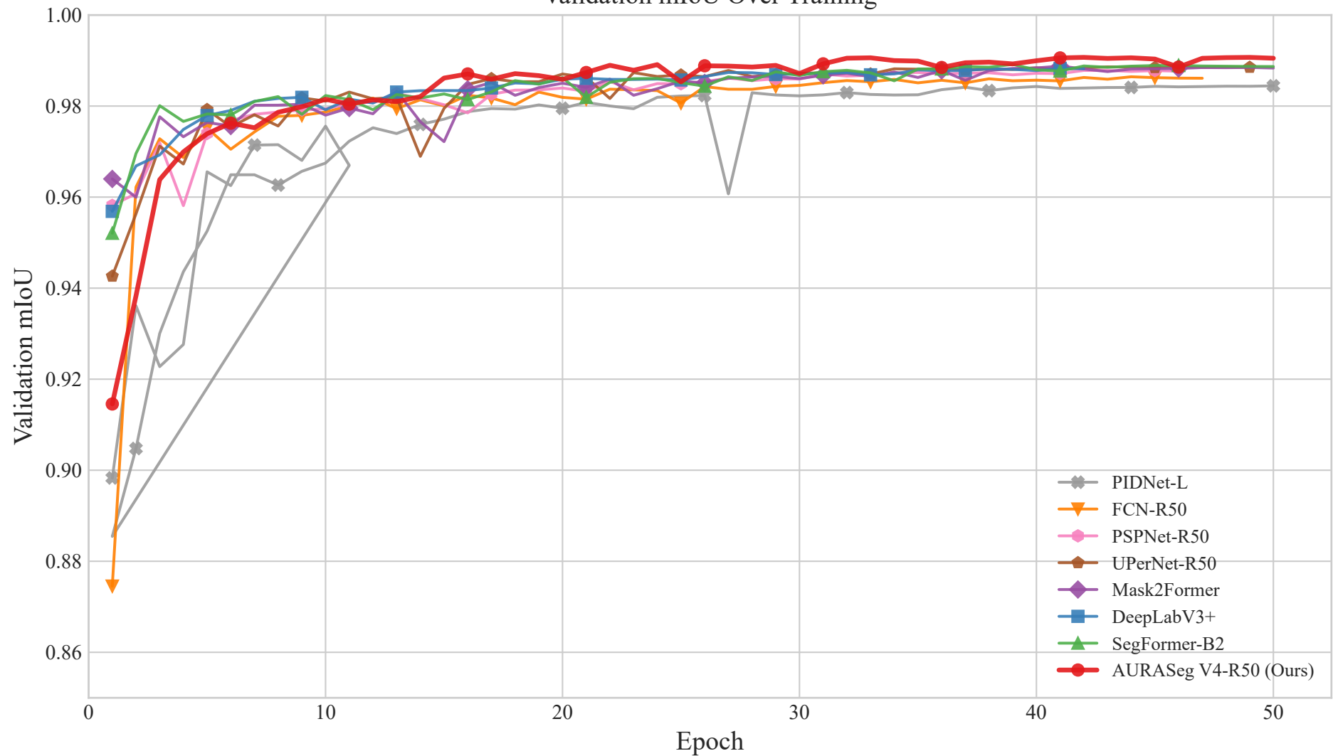
Validation mIoU Over Training
