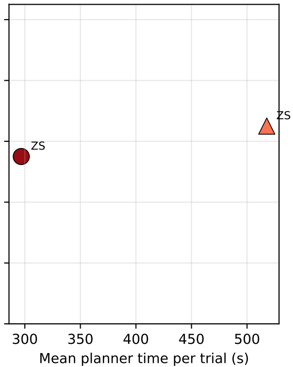
8B
