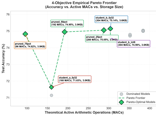
Fig. 4. Multi-objective Pareto projection mapping test accuracy, active MACs, and serialized binary size.
