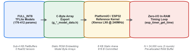
Fig. 1. The physical deployment and zero-I/O in-RAM benchmarking pipeline connecting verified FULL_INT8 TFLite FlatBuffers to bare-metal ESP32 silicon.
