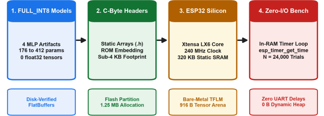
Fig. 1. The physical deployment and zero-I/O in-RAM benchmarking pipeline connecting verified FULL_INT8 TFLite FlatBuffers to bare-metal ESP32 silicon.
