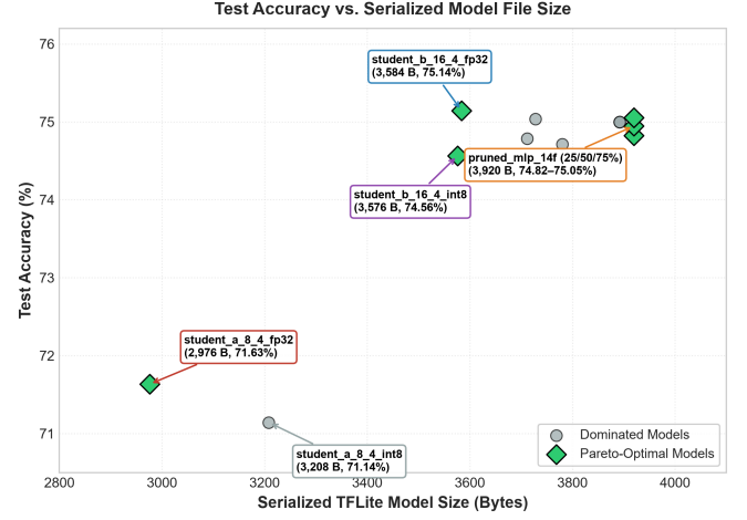
Fig. 2. Test Accuracy vs. Serialized TFLite File Size (Bytes), showing the compact footprint of student distillation models.
