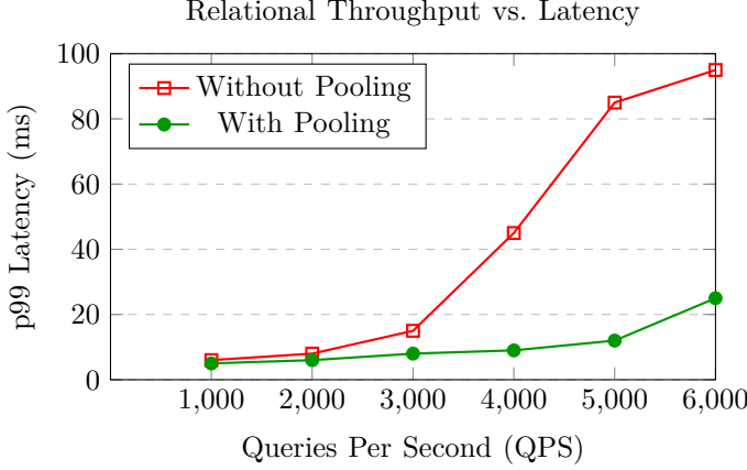
Fig. 2. Throughput Stress Test. Without pooling (Red): connection exhaustion causes p99 latency spikes beyond 3,000 QPS. With connection pooling (Green): 5,000 QPS is sustained with p99 latency below 15 ms.
