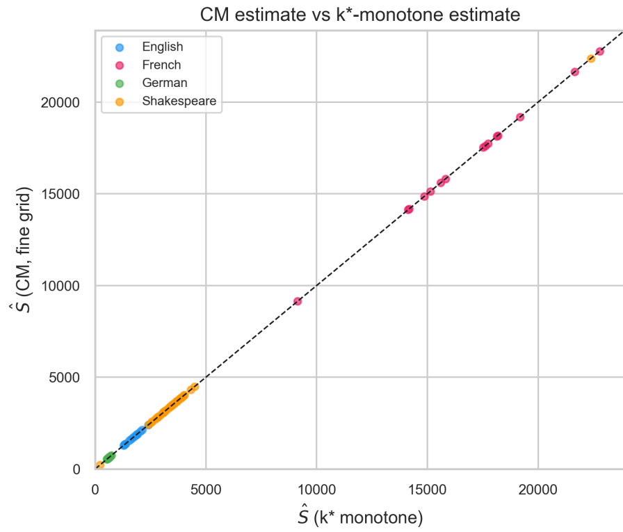
Figure 15: Comparison between completely monotone estimates and selected finite- k monotone estimates.
