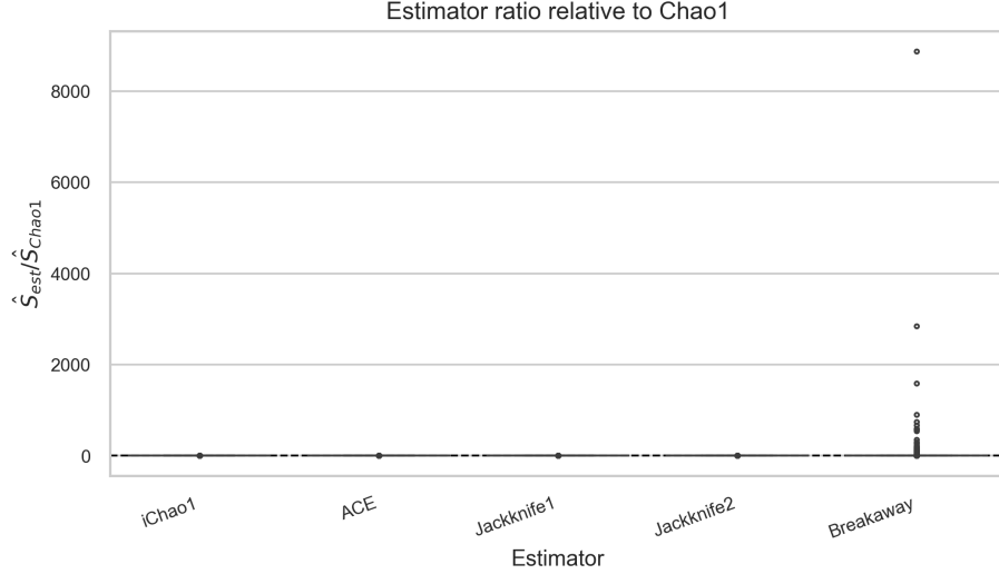
Figure 21: Ratio between each estimator and Chao1 across the spoken/dialogue corpora.
