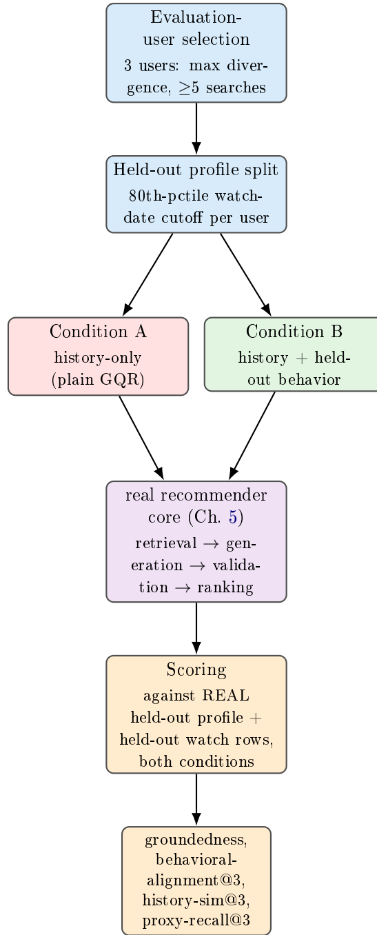
Figure 6.1: The evaluation’s ablation flow. Both conditions run the identical, real recommender-core functions; the only difference is whether the behavioral profile is passed. Scoring is decoupled from what each condition was allowed to see — both are graded against the same real held-out ground truth.
