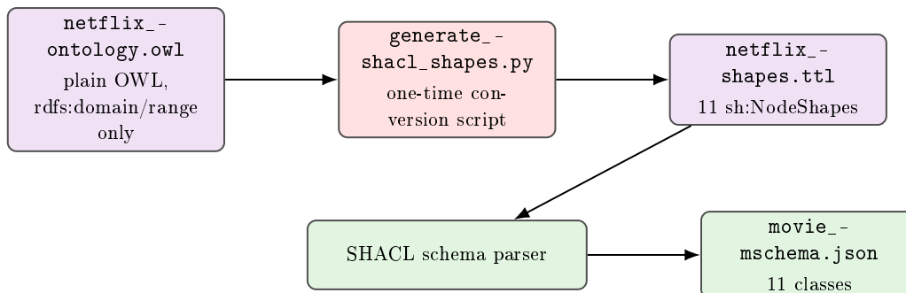
Figure 3.2: The Movie ontology has no native SHACL shapes, so a one-time script generates them from its existing rdfs:domain/rdfs:range declarations before the schema parser can consume it. This m-schema JSON is the same artifact Section 5.4’s schema-grounding check embeds and thresholds against.
