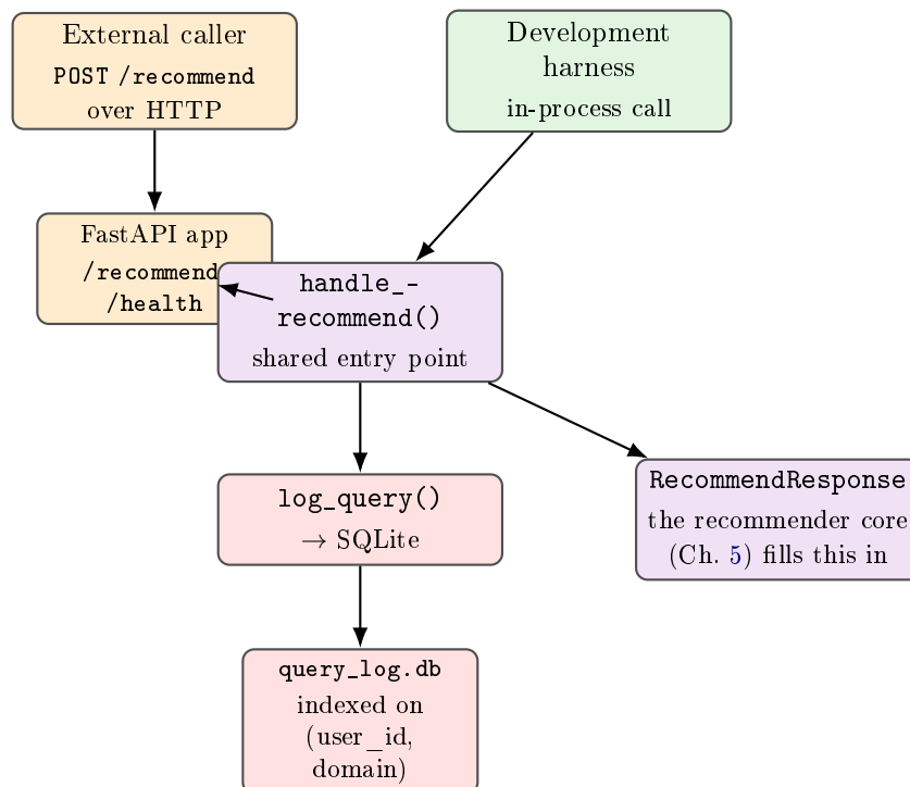
Figure 3.3: Both the real HTTP endpoint and the internal development harness converge on handle_recommend() , which validates the request, persists it, and returns a response. This is the extension point the recommender core (Chapter 5) is built inside, without any further change to the contract, the log store, or the harness.
