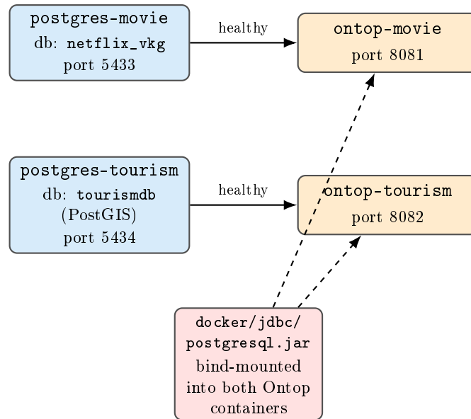
Figure 3.1: Docker Compose topology for the two Virtual Knowledge Graphs. Each Ontop container waits for its database’s healthcheck before starting, and both mount the same JDBC driver directory (dashed arrows) — a workaround for a missing-driver defect in the base Ontop image.
