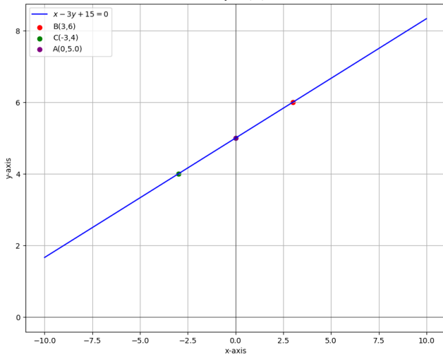
Collinearity of A, B, and C
