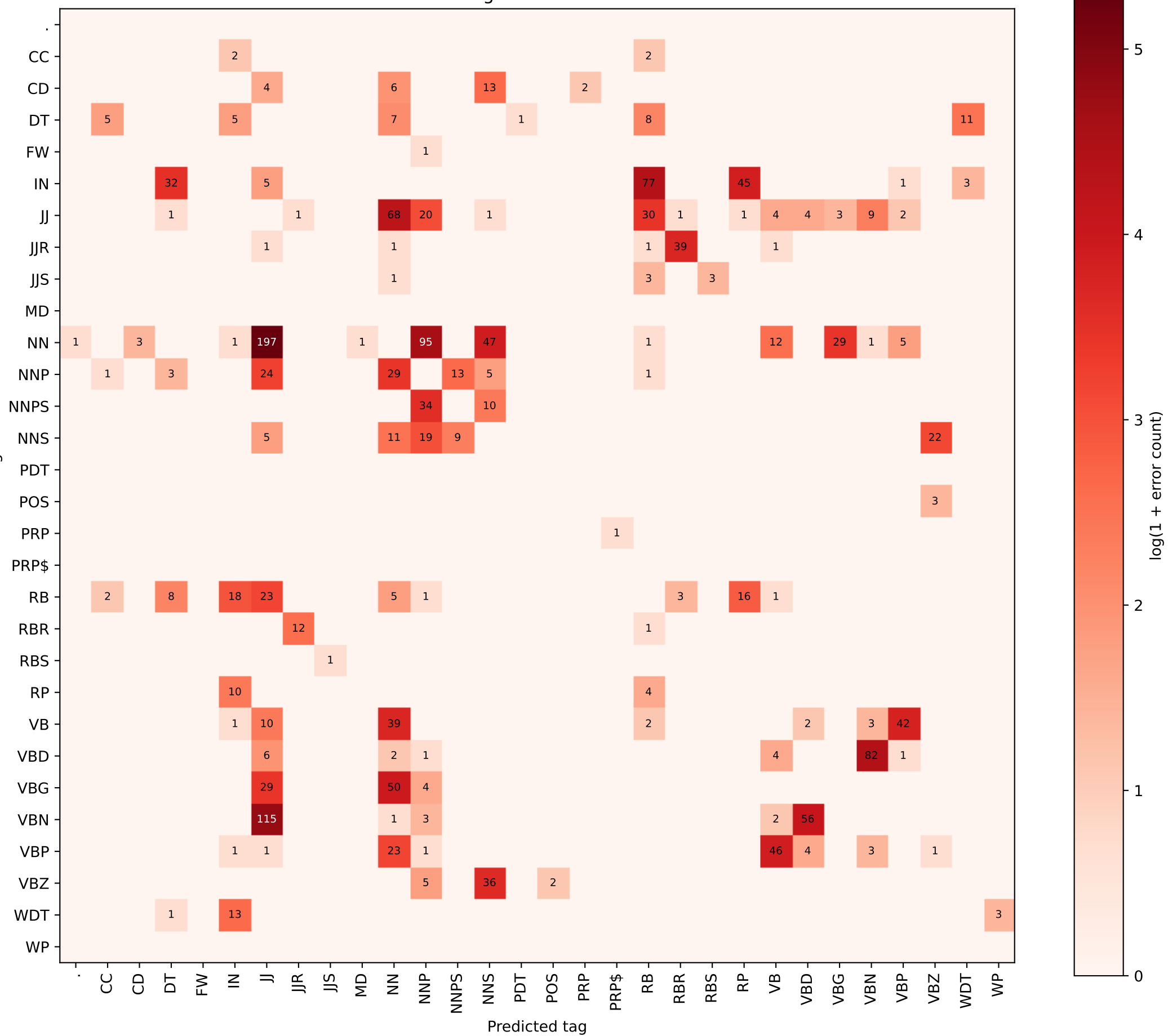
POS-Tag Confusion Matrix
