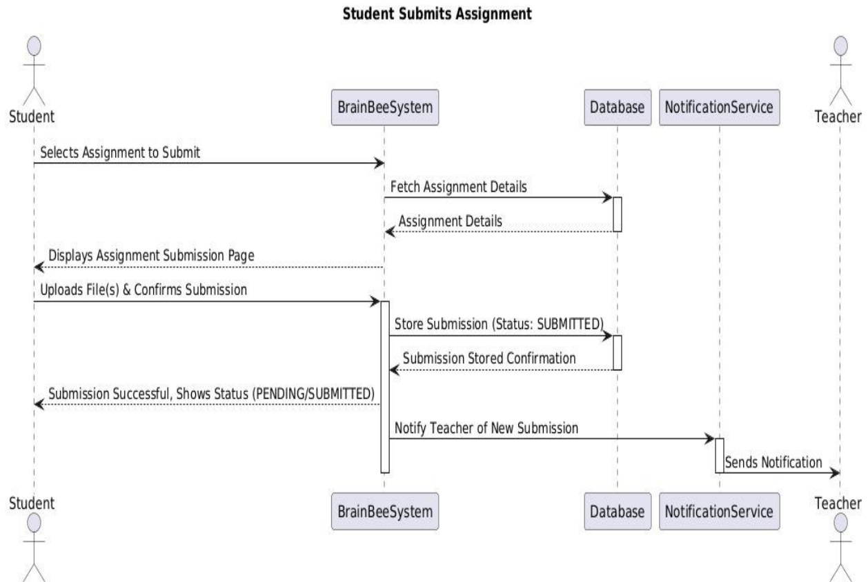
Figure 17 Sequence Diagram for Assessment Module
