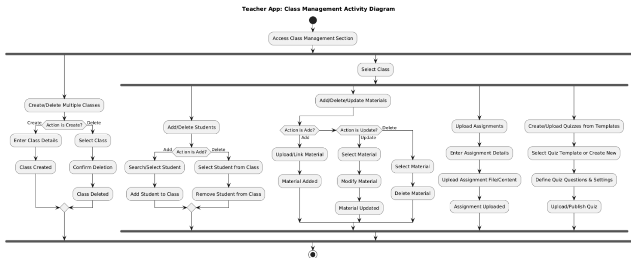
Figure 12 Activity Diagram for Class Management
