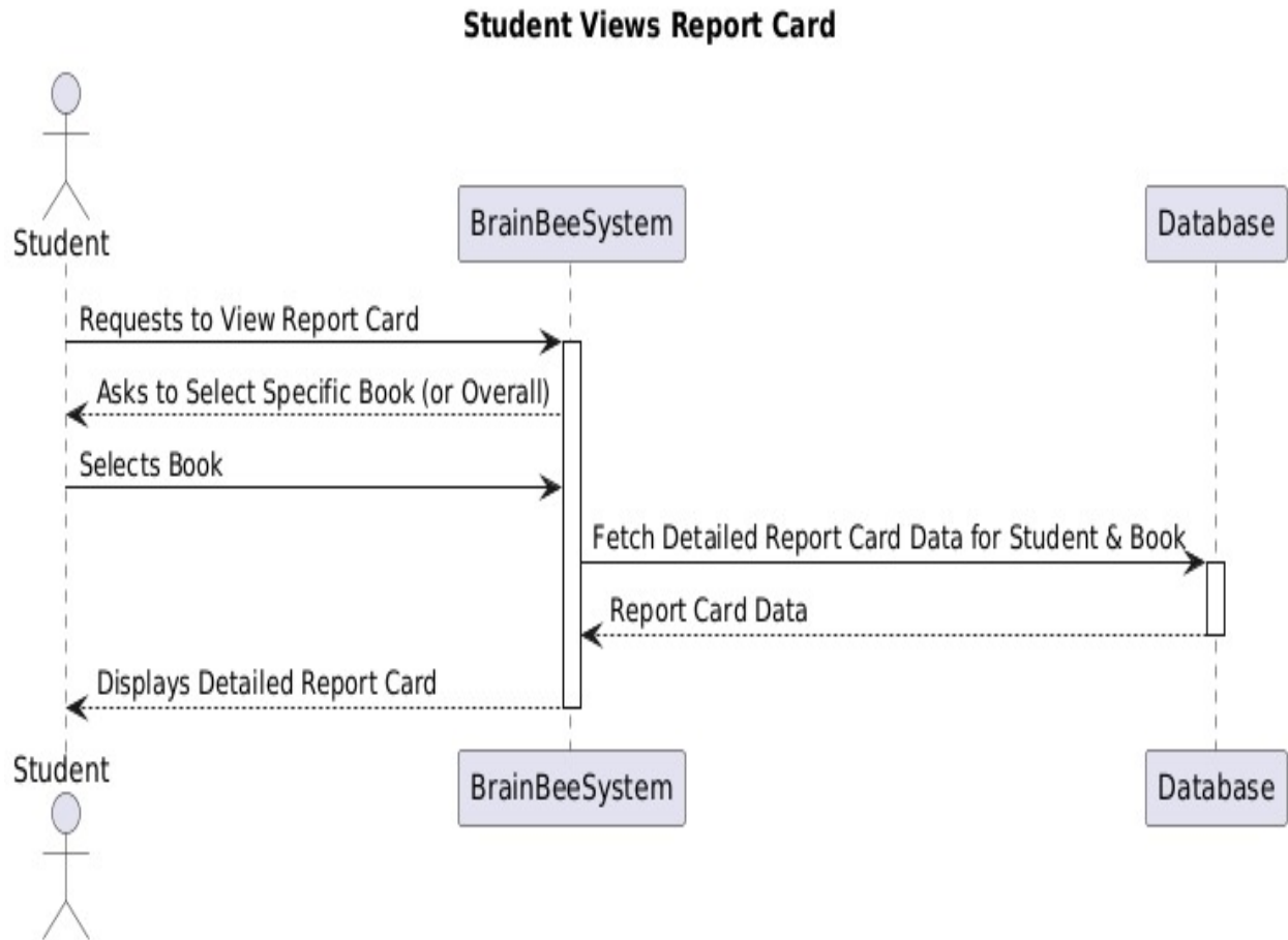
Figure 18 Sequence Diagram for Performance Analytics
