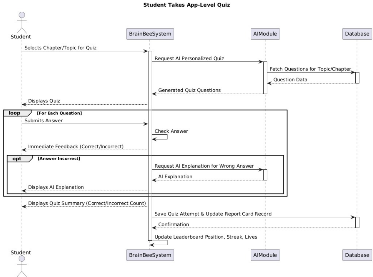
Figure 16 Sequence Diagram for Quiz
