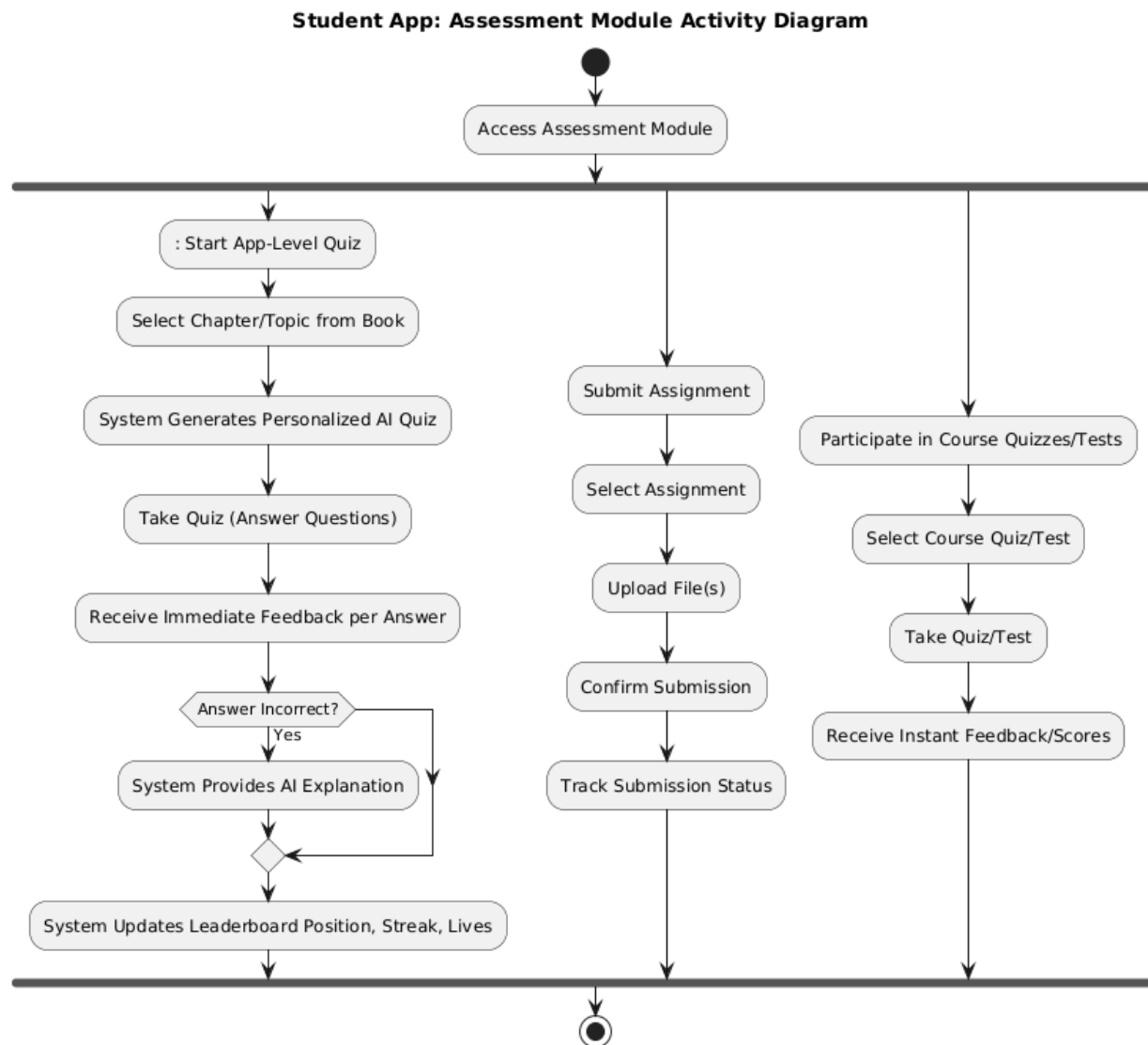
Figure 13 Activity Diagram for Assessment Module
