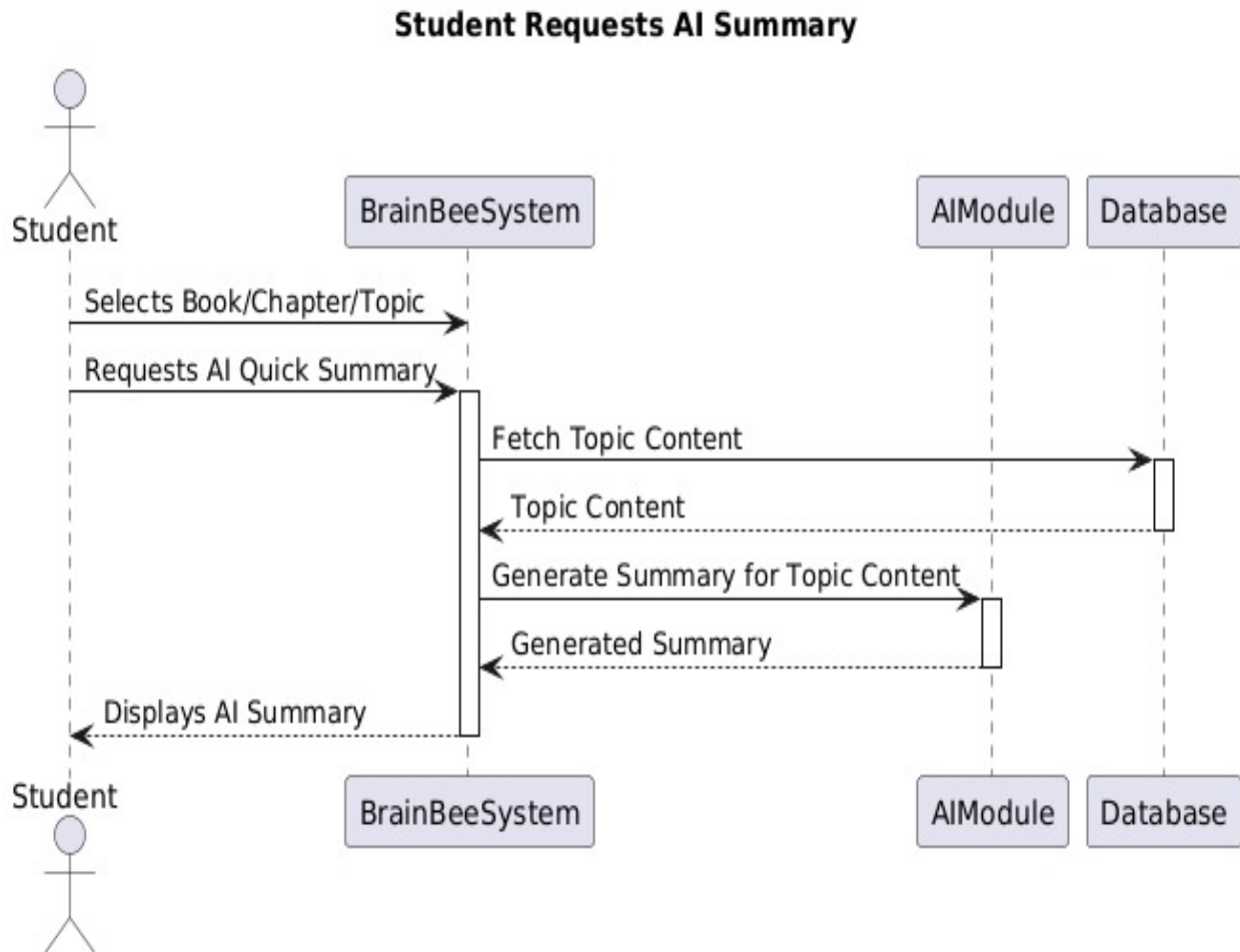
Figure 19 Sequence Diagram for AI Powered Assistant
