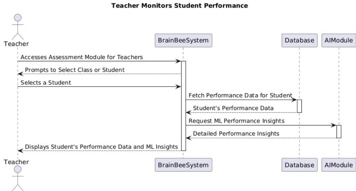
Figure 23 Sequence Diagram for Monitor Student Performance
