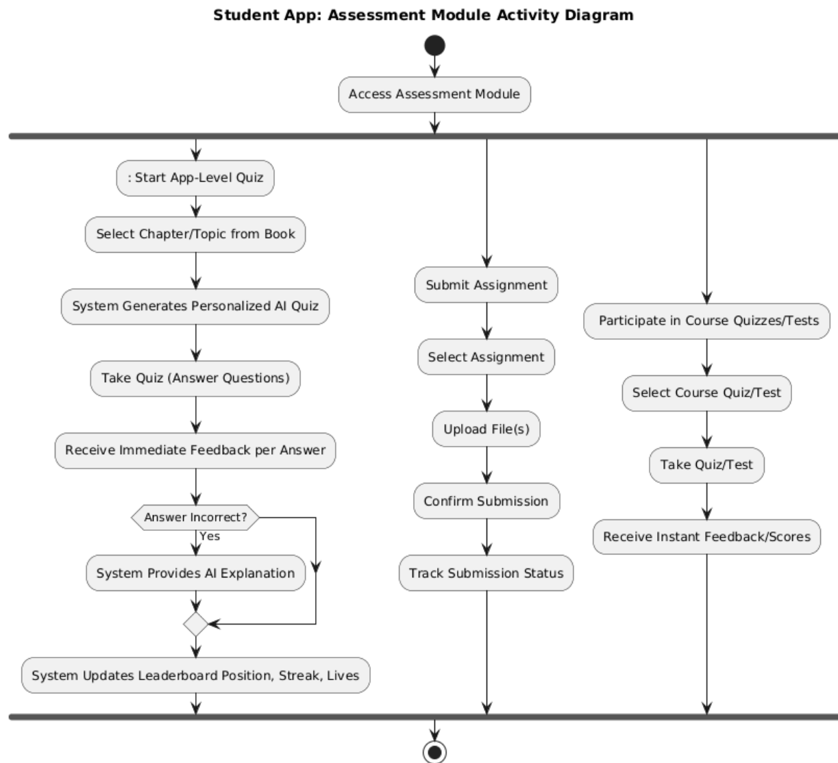
Figure 6 Activity Diagram for Assessment Module
