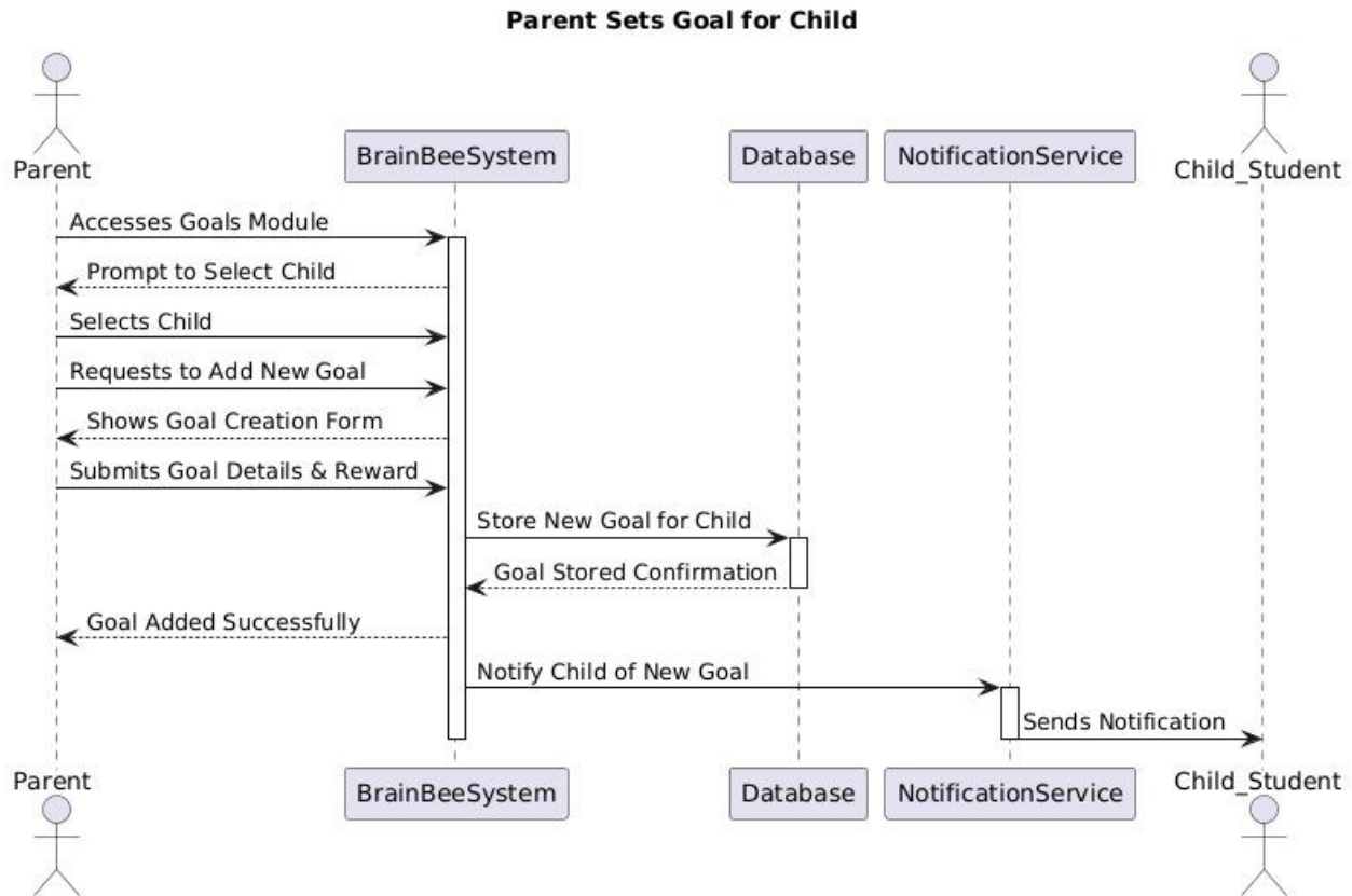
Figure 21 Sequence Diagram for Goals Module
