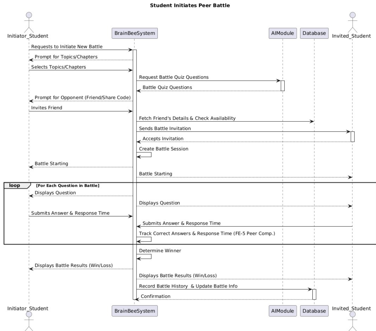
Figure 15 Sequence Diagram for Peer Competition Module
