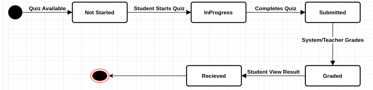
Figure 26 State Transition Diagram for Quiz Attempt
