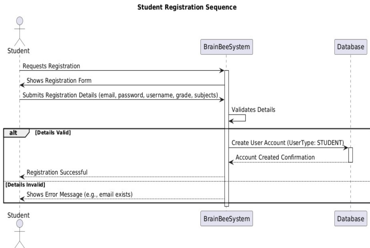
Figure 14 Sequence Diagram for User Management
