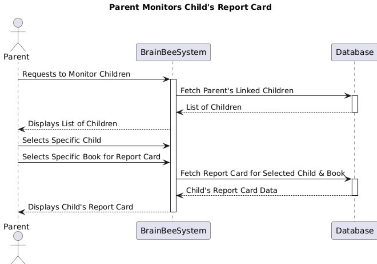
Figure 20 Sequence Diagram for Monitor Children
