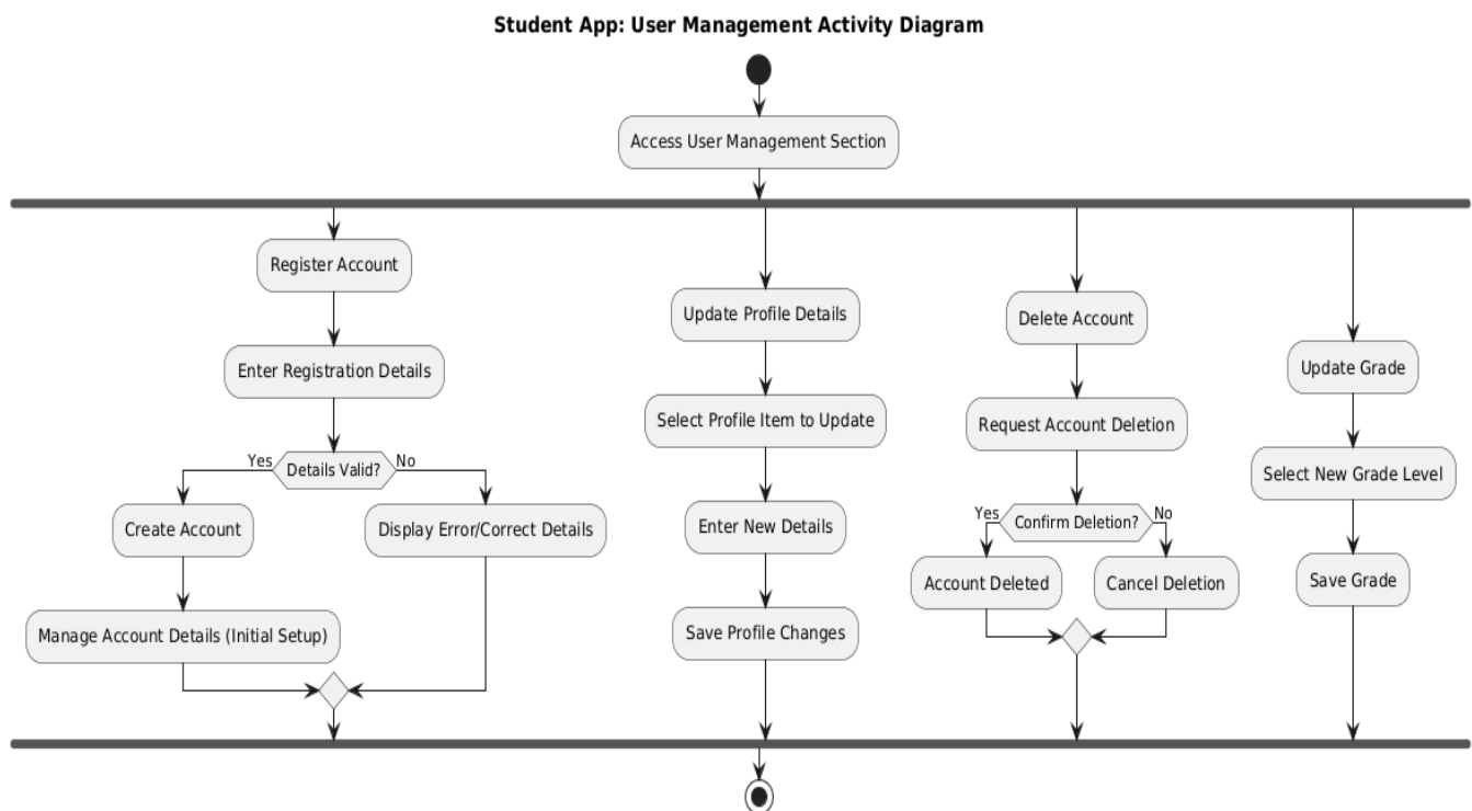
Figure 4 Activity Diagram for User Management
