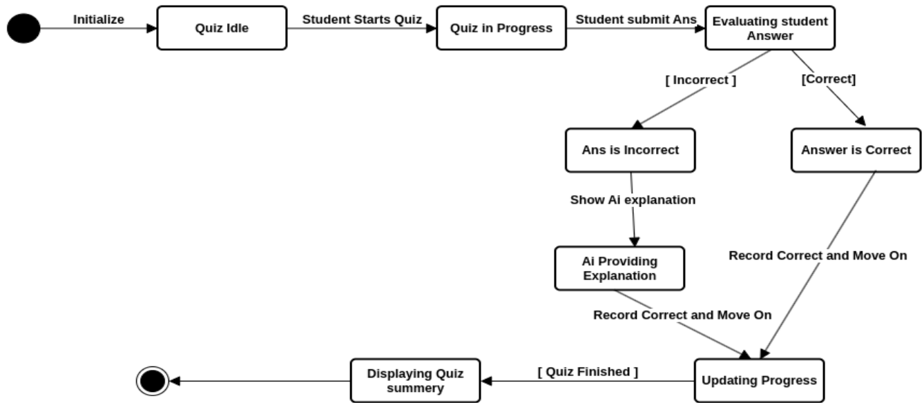
Figure 25 State Transition Diagram for Quiz
