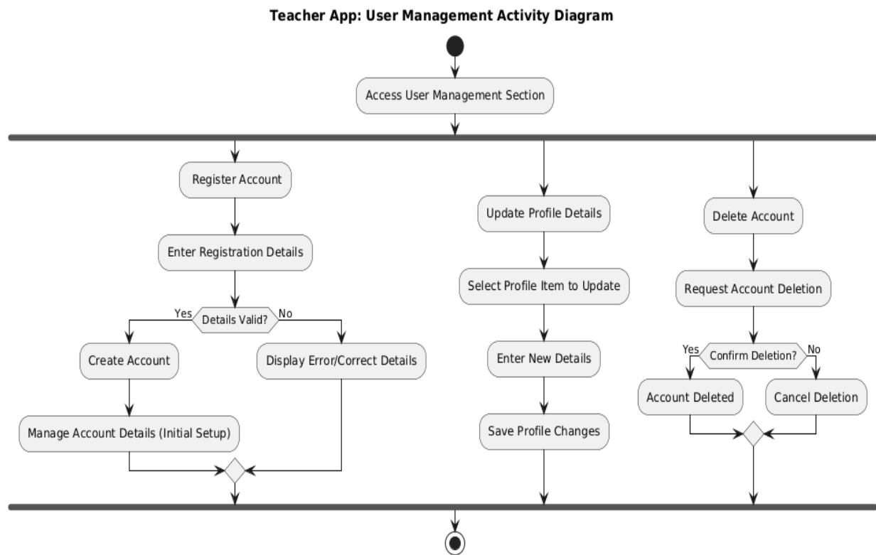
Figure 11 Activity Diagram for User Management
