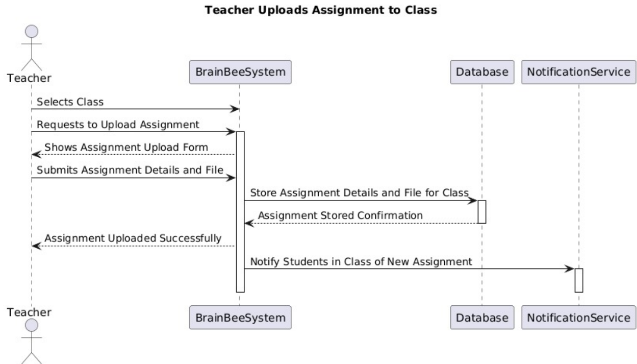
Figure 24 Sequence Diagram for Teacher Uploads assignment
