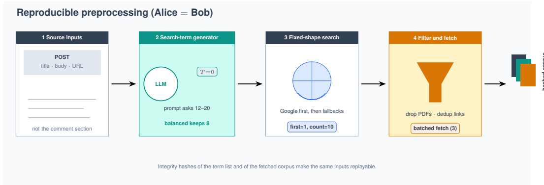
Fig. 3. Research stage: temperature-0 term generation from title, body, and URL; a fixed search request shape; filtering and batched fetching; integrity hashes that detect drift between runs but do not prevent it.
