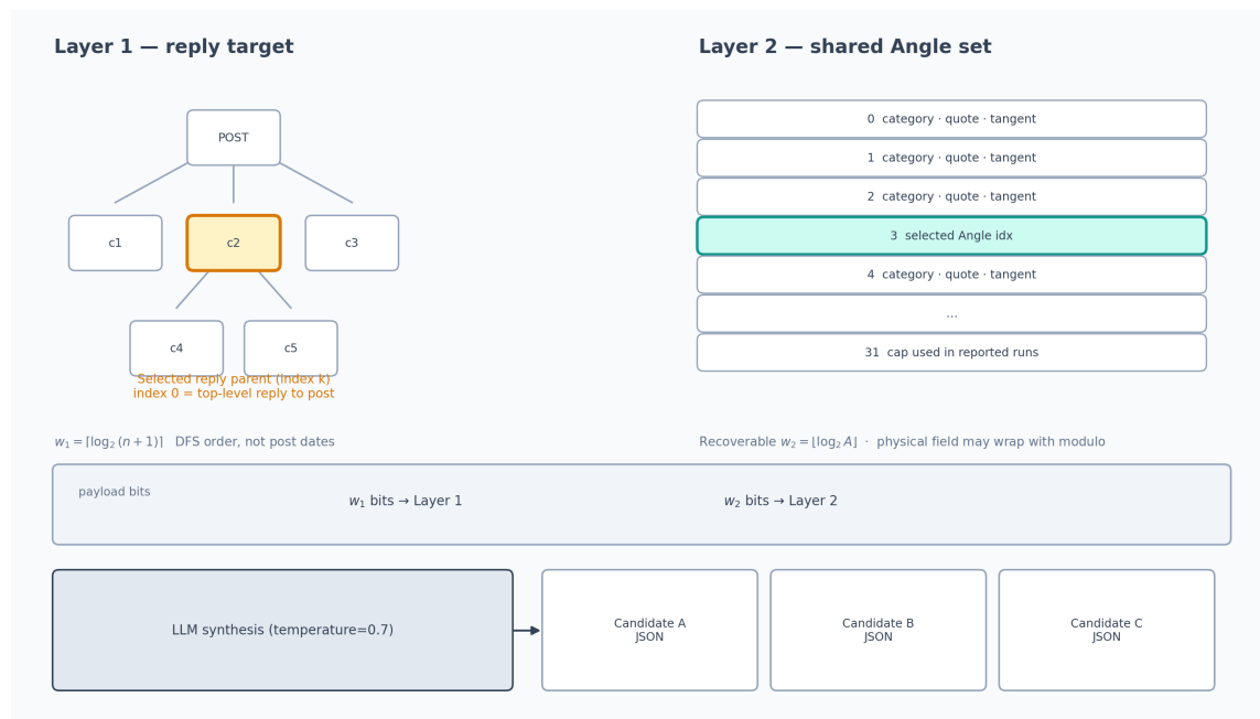
Fig. 5. Two-layer embedding: Layer 1 selects a reply target in a depth-first flattened thread; Layer 2 selects an Angle from a shared list; an LLM then writes a visible reply for that pair.
