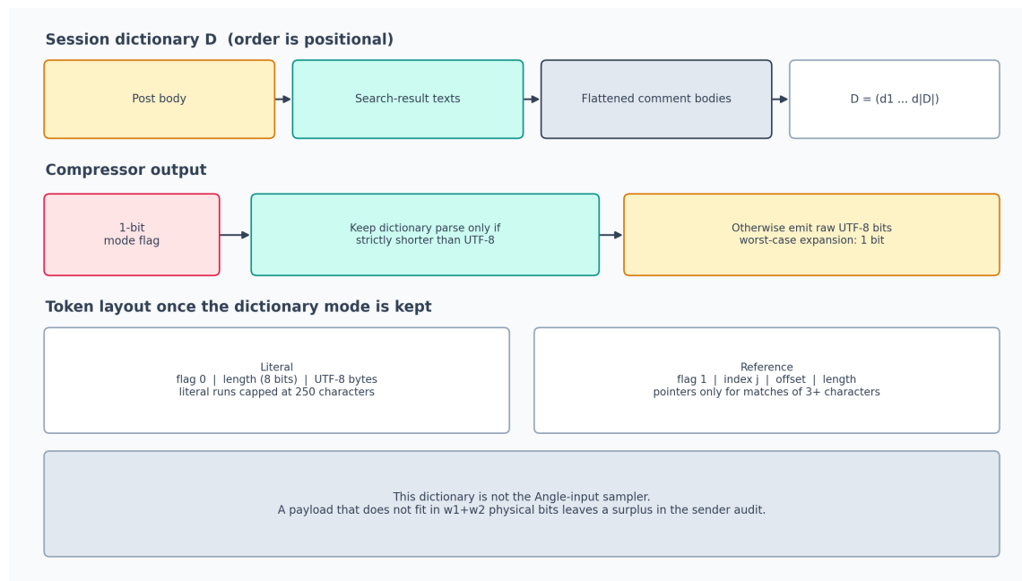
Fig. 7. Payload compression builds a session dictionary from thread and research text, then keeps a dictionary parse only when it is strictly shorter than UTF-8.
