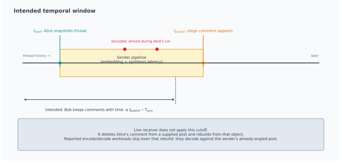
Fig. 4. Intended temporal window: Bob would keep comments dated at most t_{publish} - T_{sync} . The live receiver does not apply this filter; it rebuilds from the supplied post after deleting Alice's comment.
