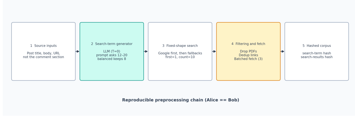
Fig. 3. Research stage: temperature-0 term generation from title, body, and URL; a fixed search request shape; filtering and batched fetching; integrity hashes for replay.
