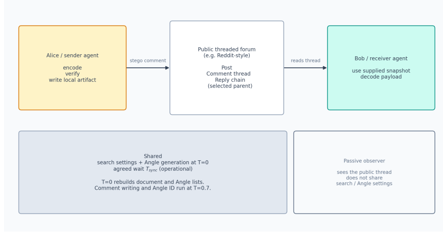
Fig. 2. Covert communication scenario: Alice and Bob use a public threaded channel. They share search and Angle-generation settings, and they agree on a temporal window. The live receiver still needs that snapshot to be supplied; it does not apply the cutoff itself.
