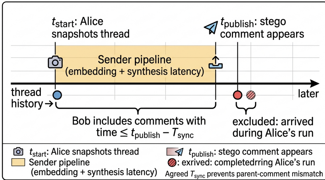
Fig. 4. Temporal synchronization: Bob's reconstructed thread state matches Alice's by agreeing on T_{\text{sync}} and filtering comments relative to t_{\text{publish}} .
