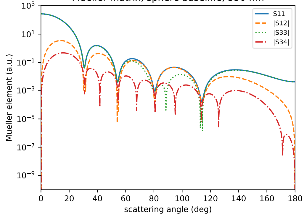
Mueller matrix, sphere baseline, 550 nm
