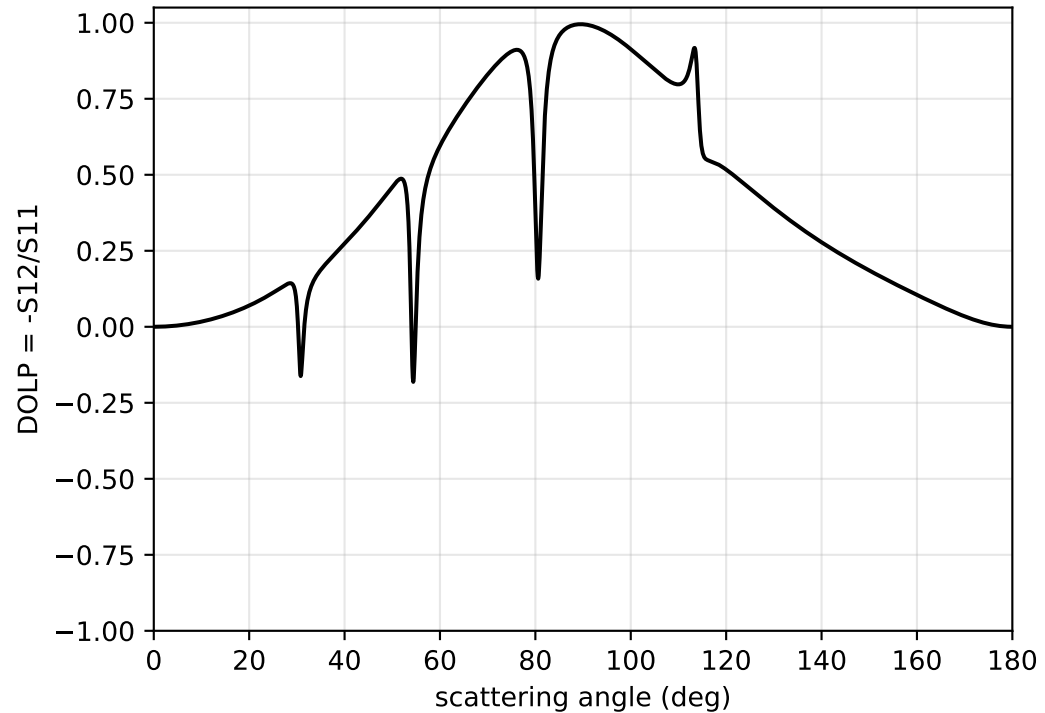
Degree of linear polarization ( \xi=1 )
