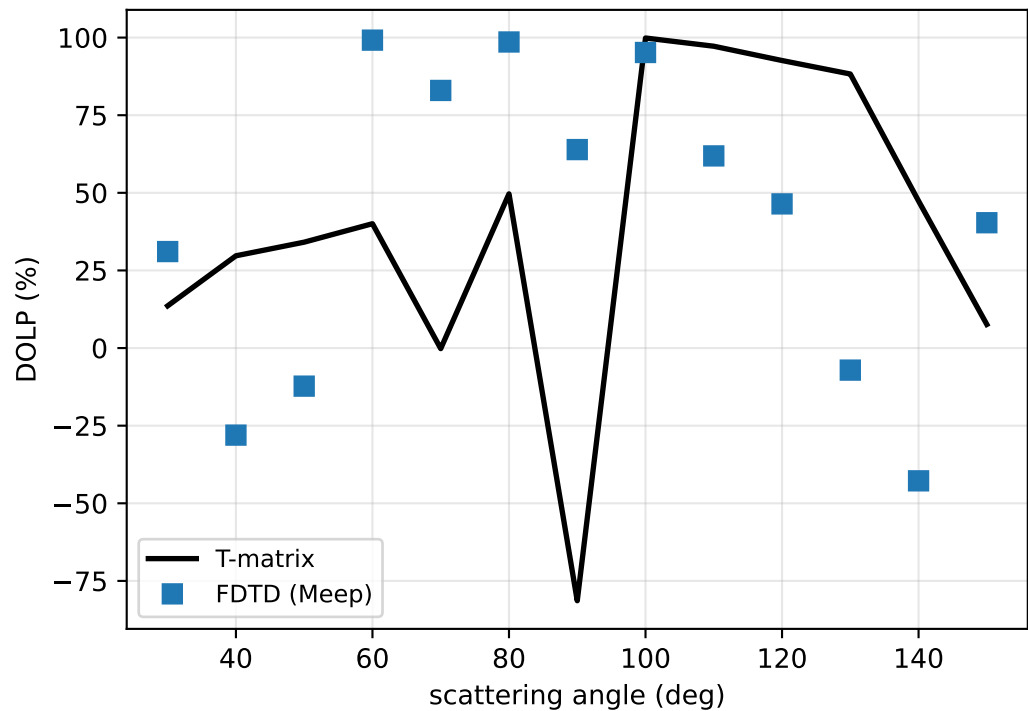
Cross-check: prolate needle \xi=5 broadside, x=8.57
