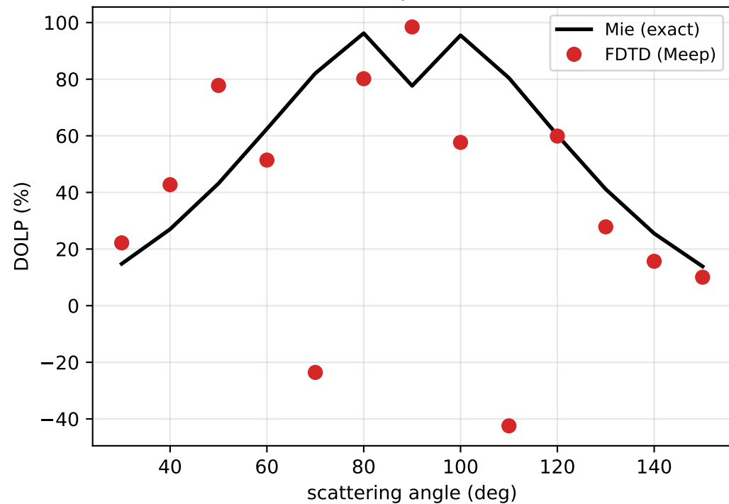
Validation: sphere, x=3.14
