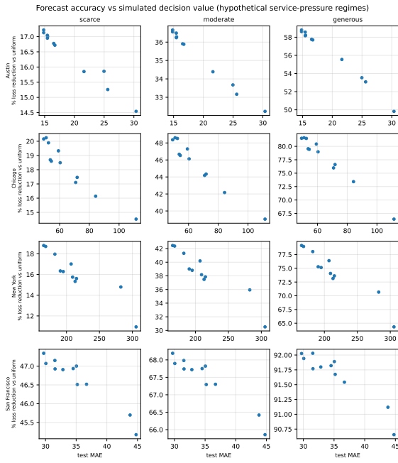
Fig. 4. Test MAE ( x ) versus simulated loss reduction relative to the uniform floor ( y ), point-forecast grid under the greedy policy with the fixed-index tie-break (the non-identified diagnostic view), by city and regime.
