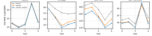
Fig. 3. Rolling-origin fold MAE (LightGBM) by feature set; orderings are stable across folds in all cities.
