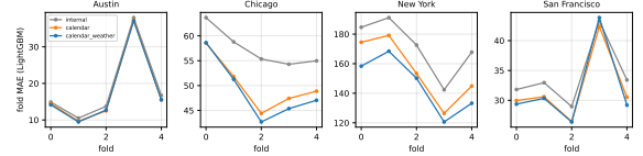
Fig. 3. Rolling-origin fold MAE (LightGBM) by feature set; orderings are stable across folds in all cities.
