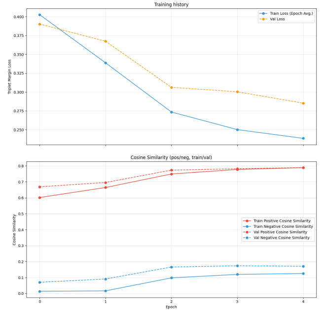
Fig. 3. Fine-tuning result of BERT model aligned to token embeddings.
