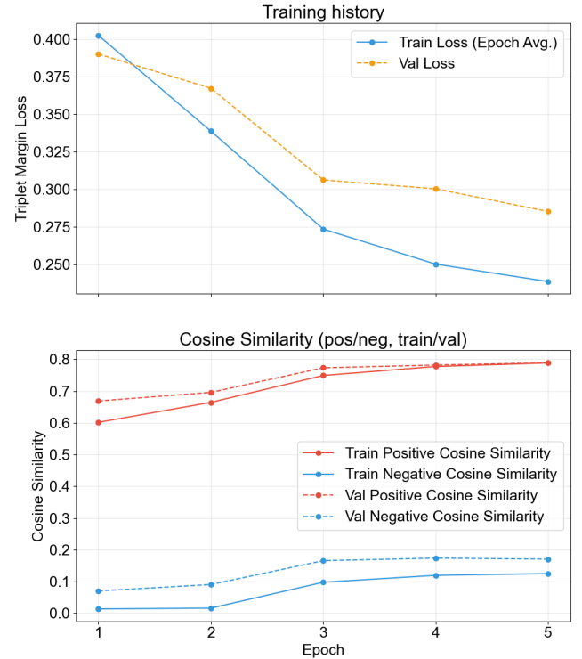
Fig. 3. Fine-tuning result of BERT model aligned to token embeddings.
