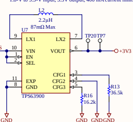
75 nA Iq, 400 mA max, Buck Boost
