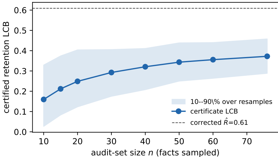
Price of certification shrinks with audit size
