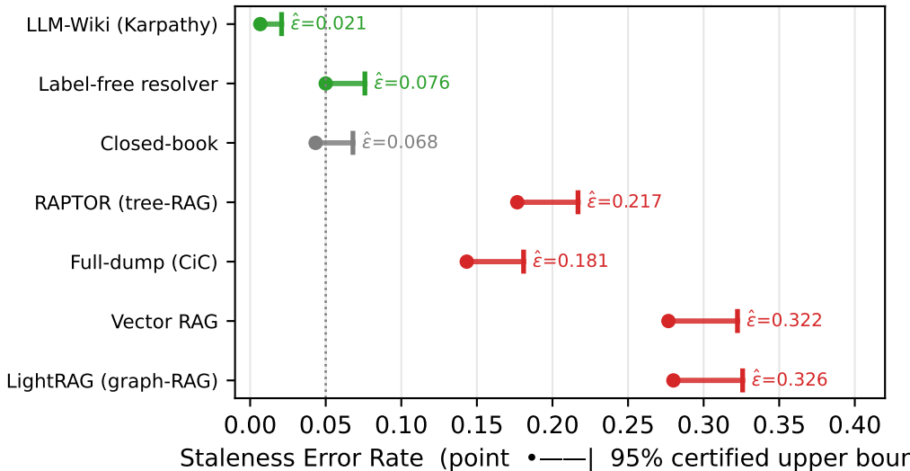
Per-store currency certificate (HoH, n=300, 14B)
