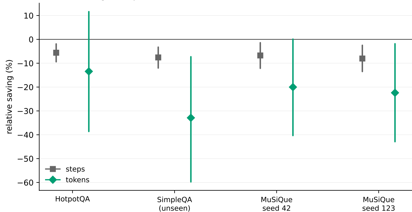
Relative saving in steps vs in tokens, with 95% CIs
