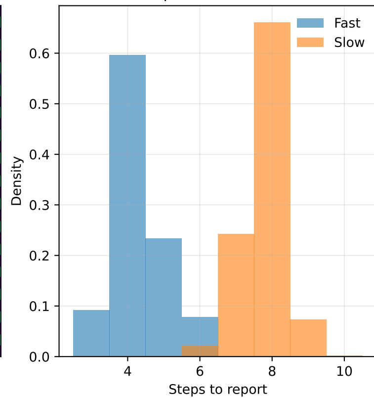
E. Step-count distribution
