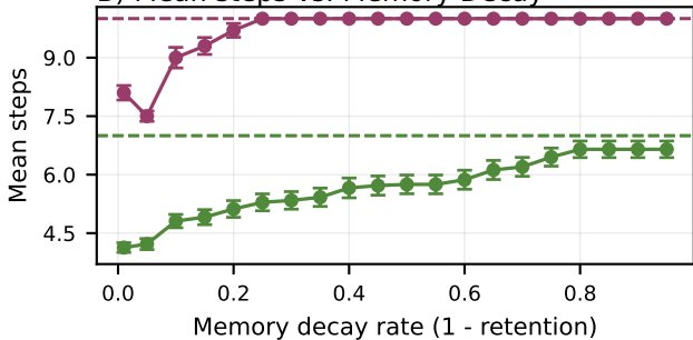
B) Mean steps vs. Memory Decay
