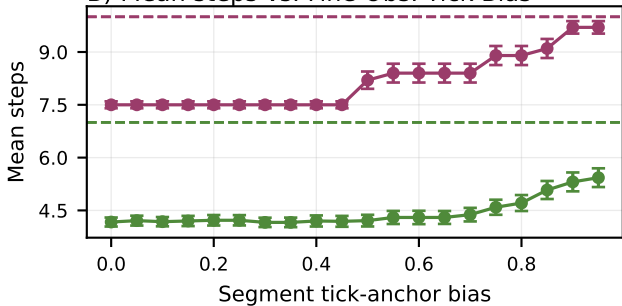
B) Mean steps vs. Fine Obs. Tick Bias
