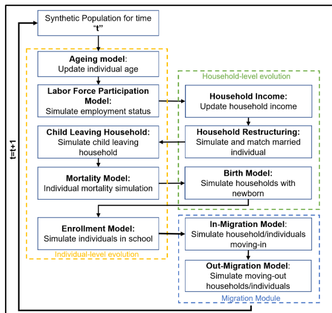
Figure 1. Demographic Microsimulator Sub-Models
