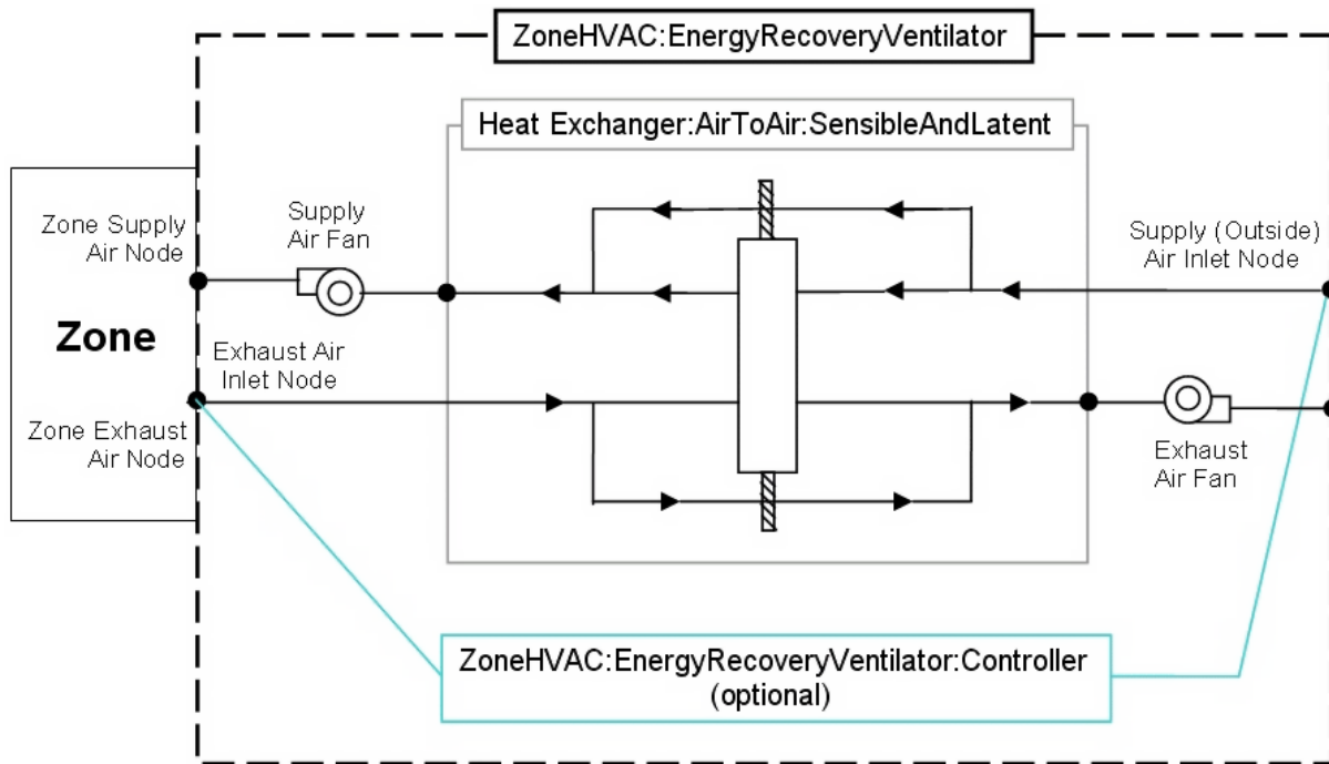
Figure 1.149: ZoneHVAC:EnergyRecoveryVentilator compound object Schematic
