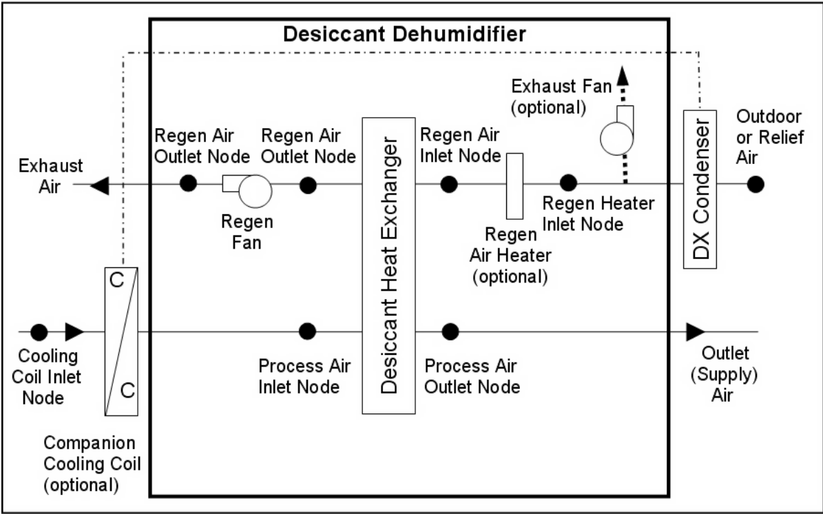
Figure 1.195: Schematic of Dehumidifier:Desiccant:System with Draw Through Regeneration Fan Placement
