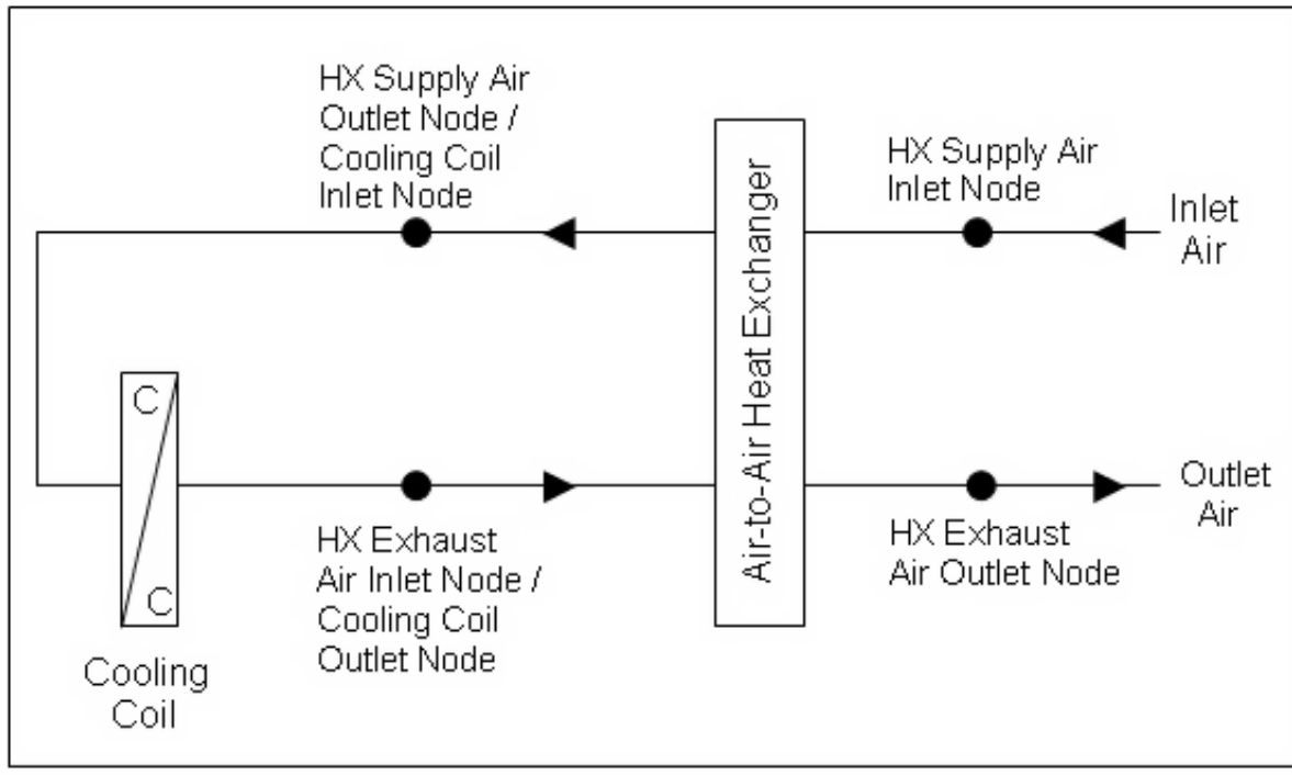
Figure 1.178: Schematic of the CoilSystem:Cooling:Water:HeatExchangerAssisted compound object
