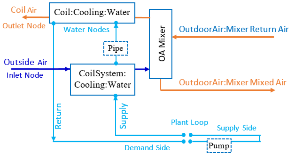
Figure 1.181: Wrap-Around Water Coil Heat Recovery System In Outdoor Air System
