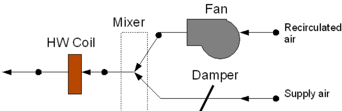
Figure 1.136: Parallel PIU Terminal Unit
