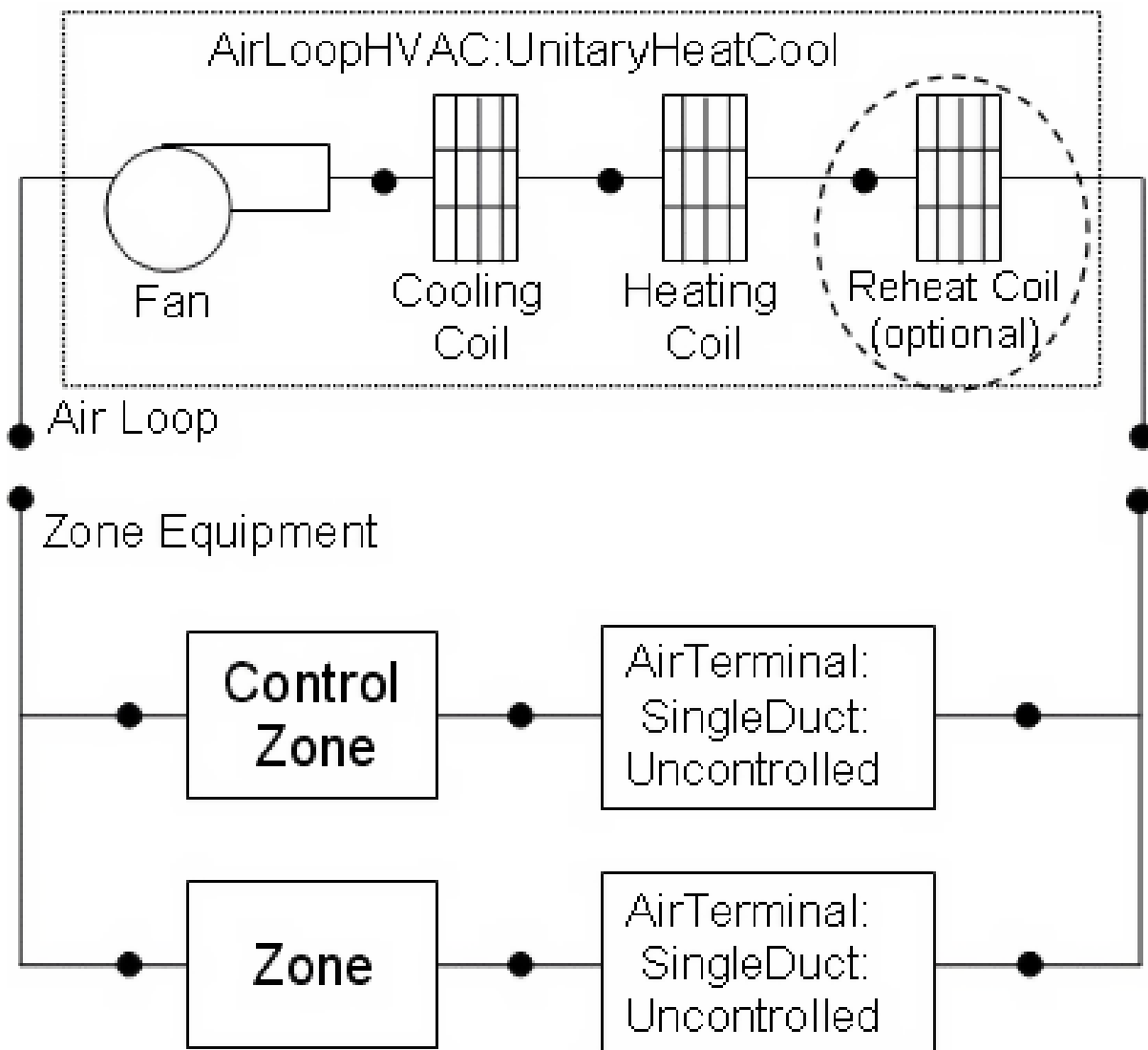
Figure 1.155: Schematic of Blow Through Heat/Cool Unitary System
