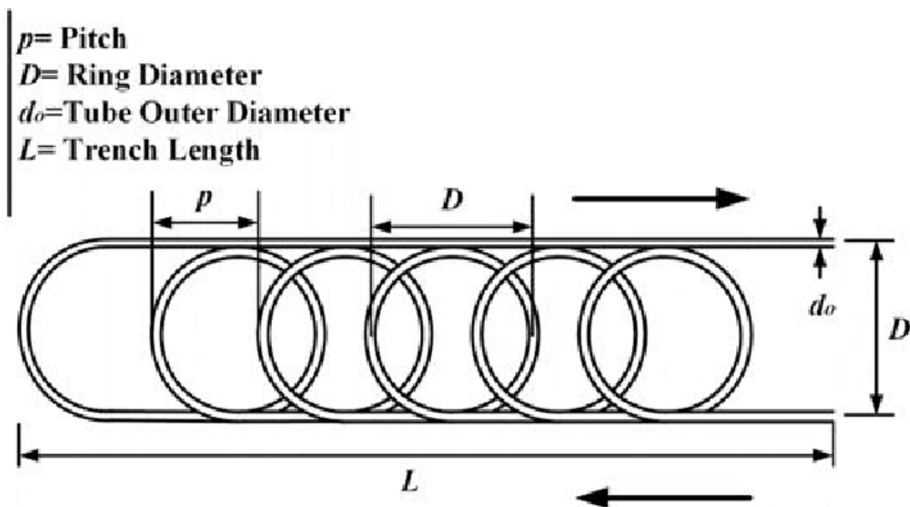
Figure 1.106: slinky heat exchanger
