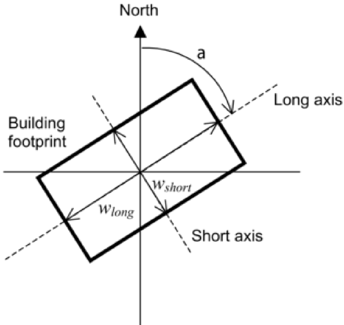
Figure 1.119: Footprint of a rectangular building showing variables used by the program to calculate surface-average wind pressure coefficients. The angle a is the “Azimuth Angle of Long Axis of Building.” w_{short}/w_{long} is the “Ratio of Building Width Along Short Axis to Width Along Long Axis.”
