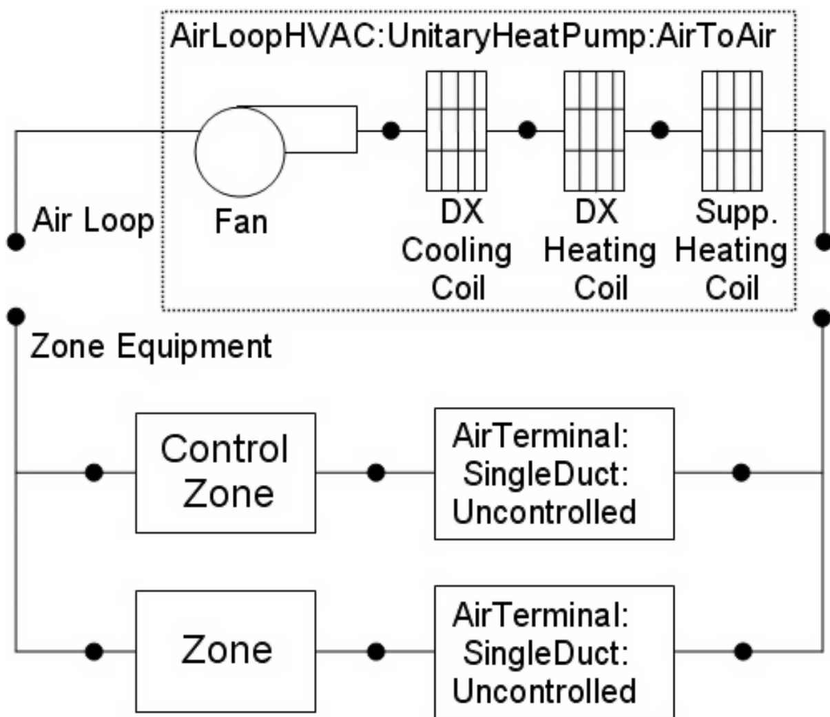
Figure 1.156: Schematic of EnergyPlus Unitary Air-to-Air Heat Pump (Blow Through Configuration)
