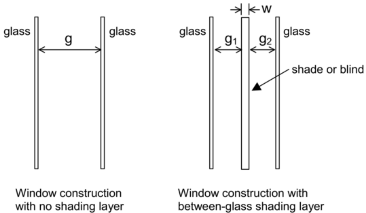
Figure 1.27: Illustration for material ordering in windows.
