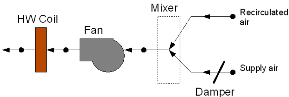
Figure 1.133: Series PIU Terminal Unit
