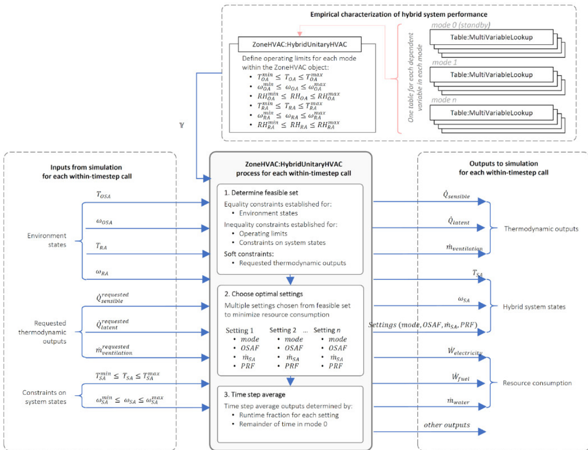
Figure 1.151: Schematic explanation of the architecture and function of ZoneHVAC:HybridUnitaryHVAC
