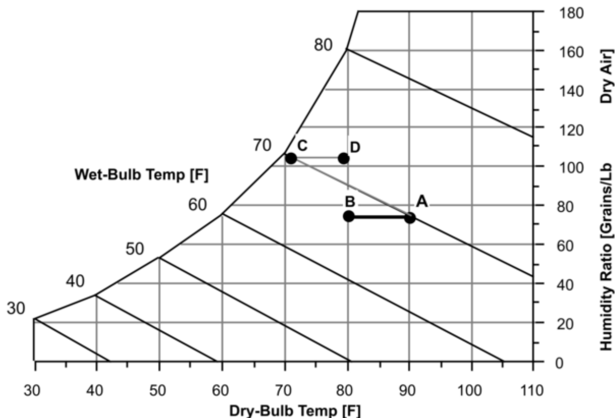
Figure 1.201: Secondary Air Process – Indirect Dry Coil Evap Cooler
