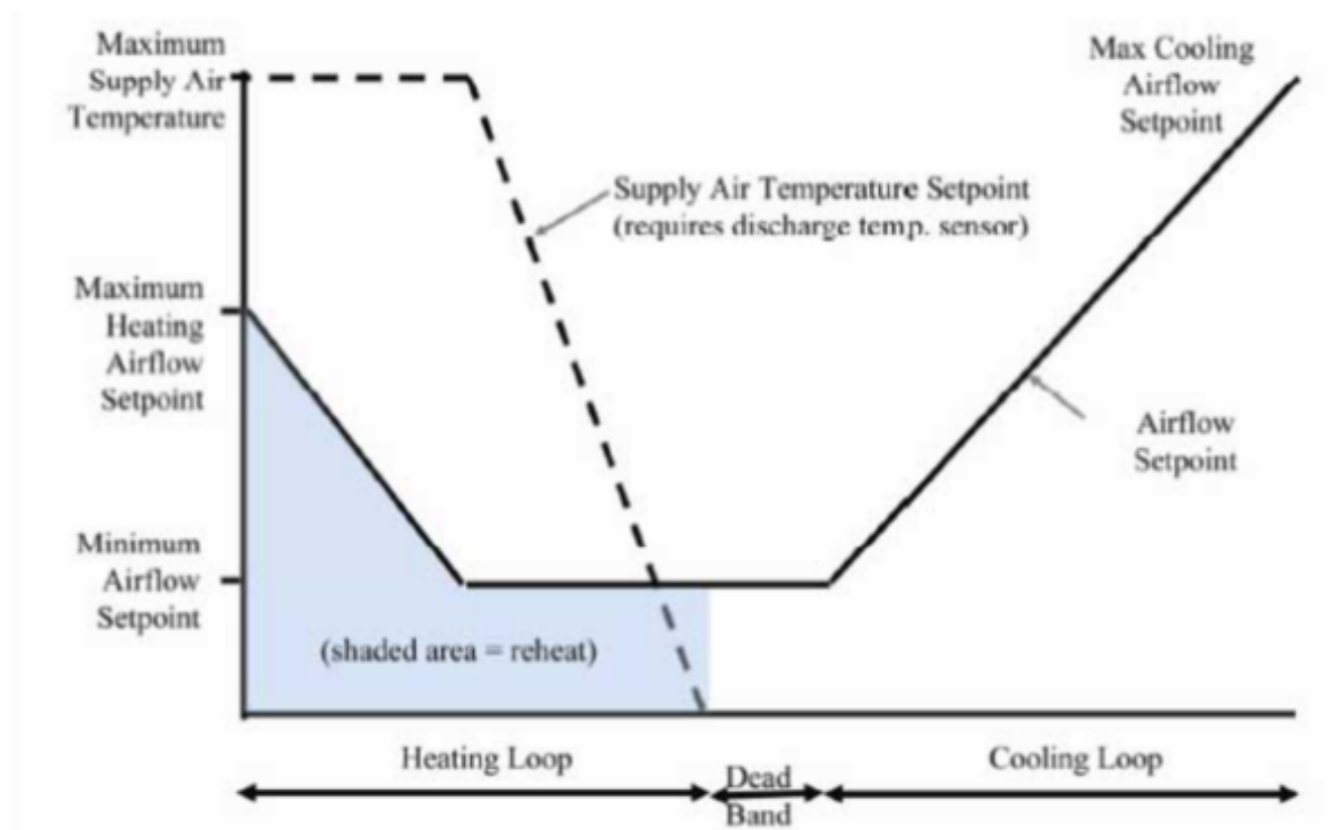
Figure 1.130: The Dual Maximum Control Logic
