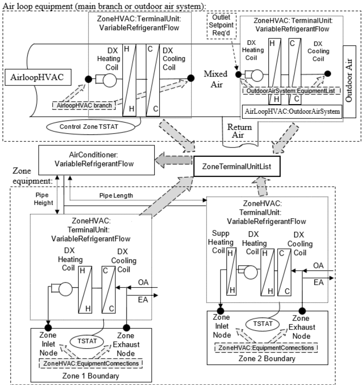
Figure 1.164: Variable Refrigerant Flow Schematic
