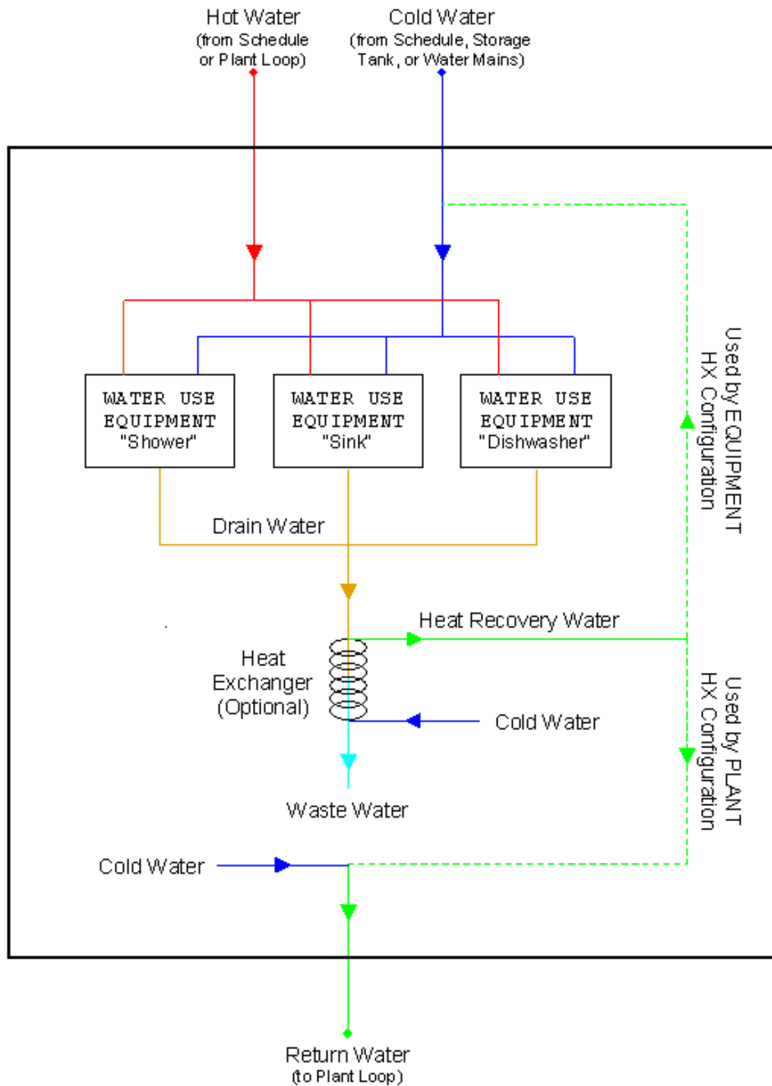
Figure 1.213: Diagram of internal connections for WaterUse:Connections
