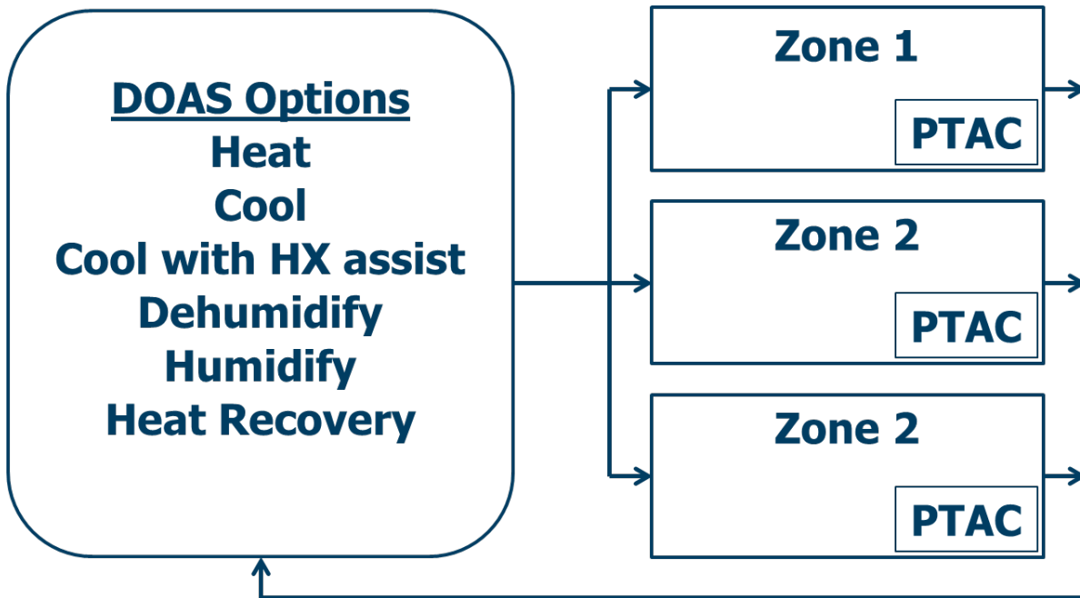
Figure 2.10: DOAS serving three zones with PTACs.
