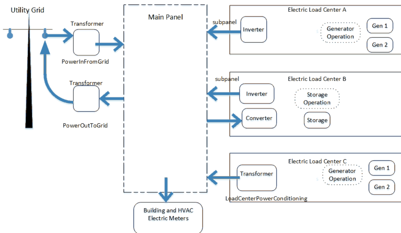
Figure 1.206: PowerServiceOverview
