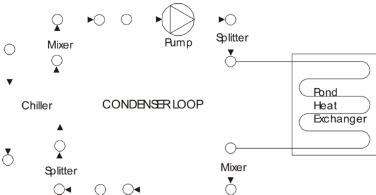
Figure 1.107: Example of Pond Ground Heat Exchanger as only heat exchanger on condenser loop
