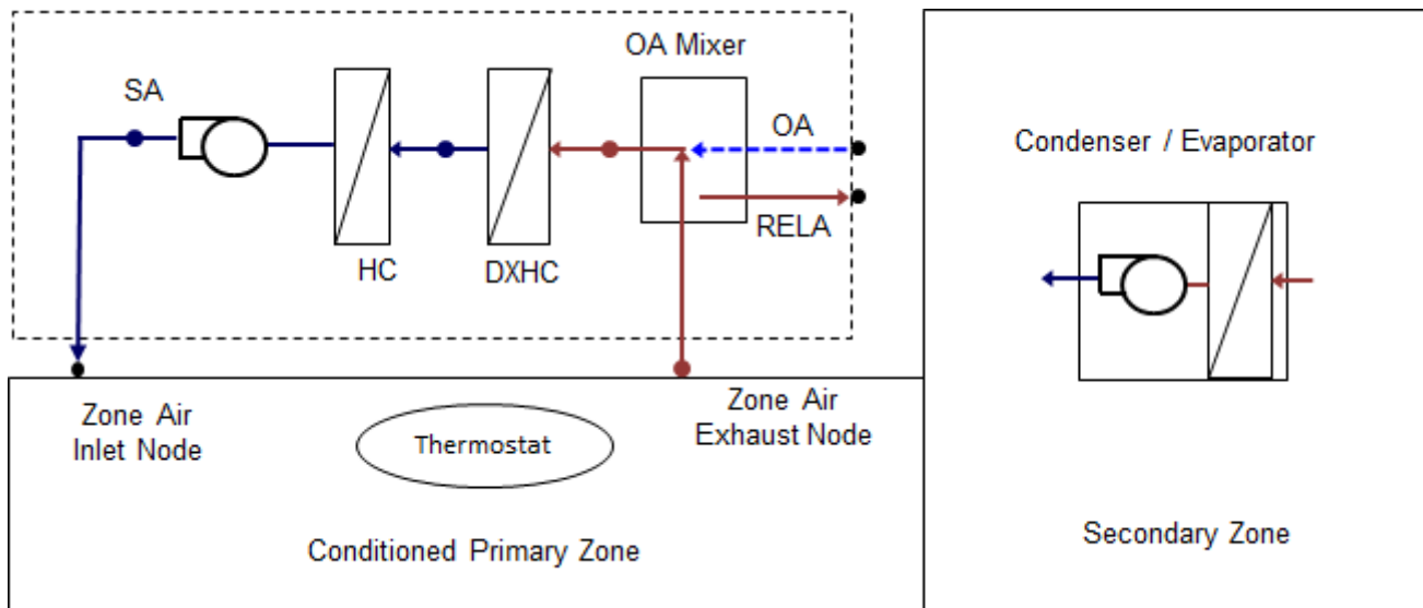
Figure 1.193: Schematic of DX system and secondary coil in cooling mode
