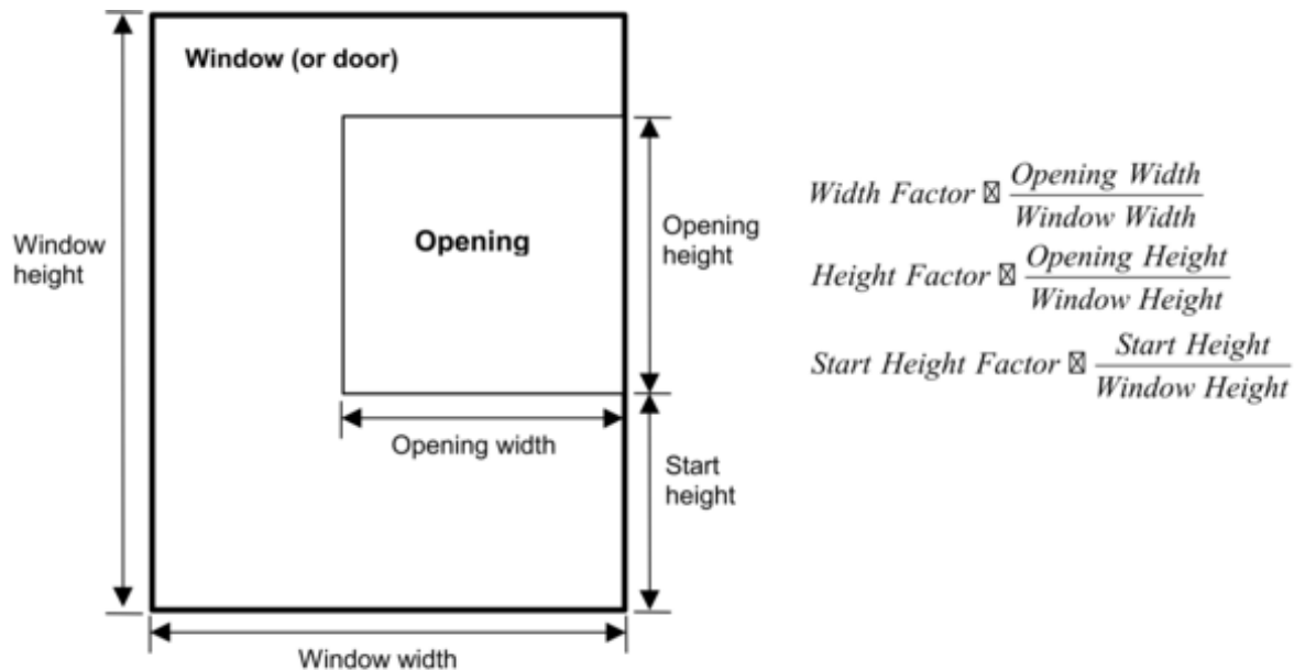
Figure 1.123: Window (or door) showing geometrical factors associated with an opening through which air flows.
