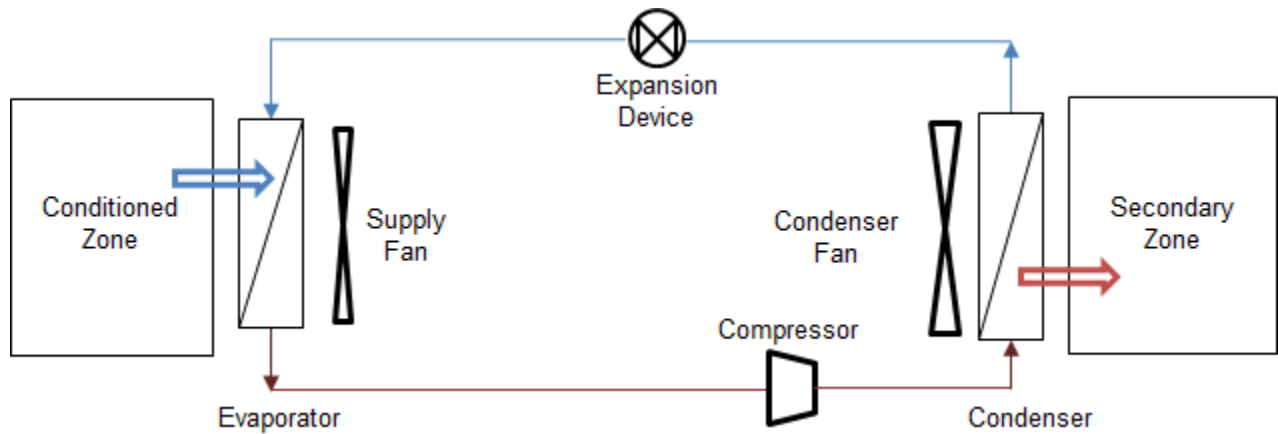
Figure 1.192: Schematic of DX System and heat pump in cooling operating mode
