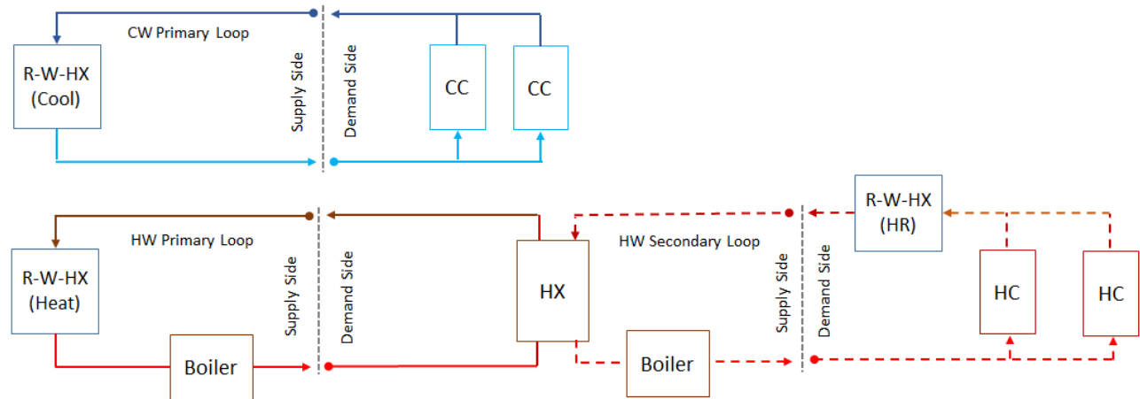
Figure 1.95: Schematic of Six-Pipe Air-to-Water Heat Pump with Heat Recovery
