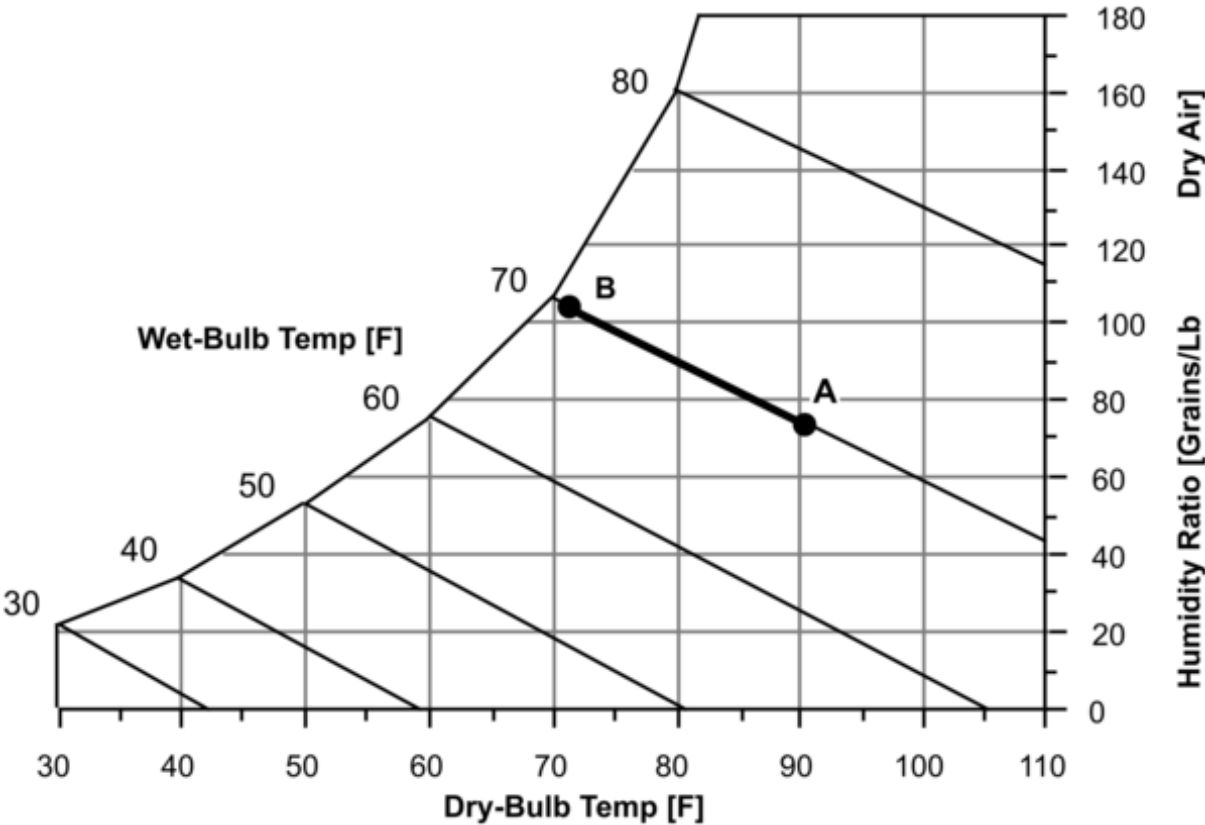
Figure 1.199: Psychrometric Chart – Constant Enthalpy
