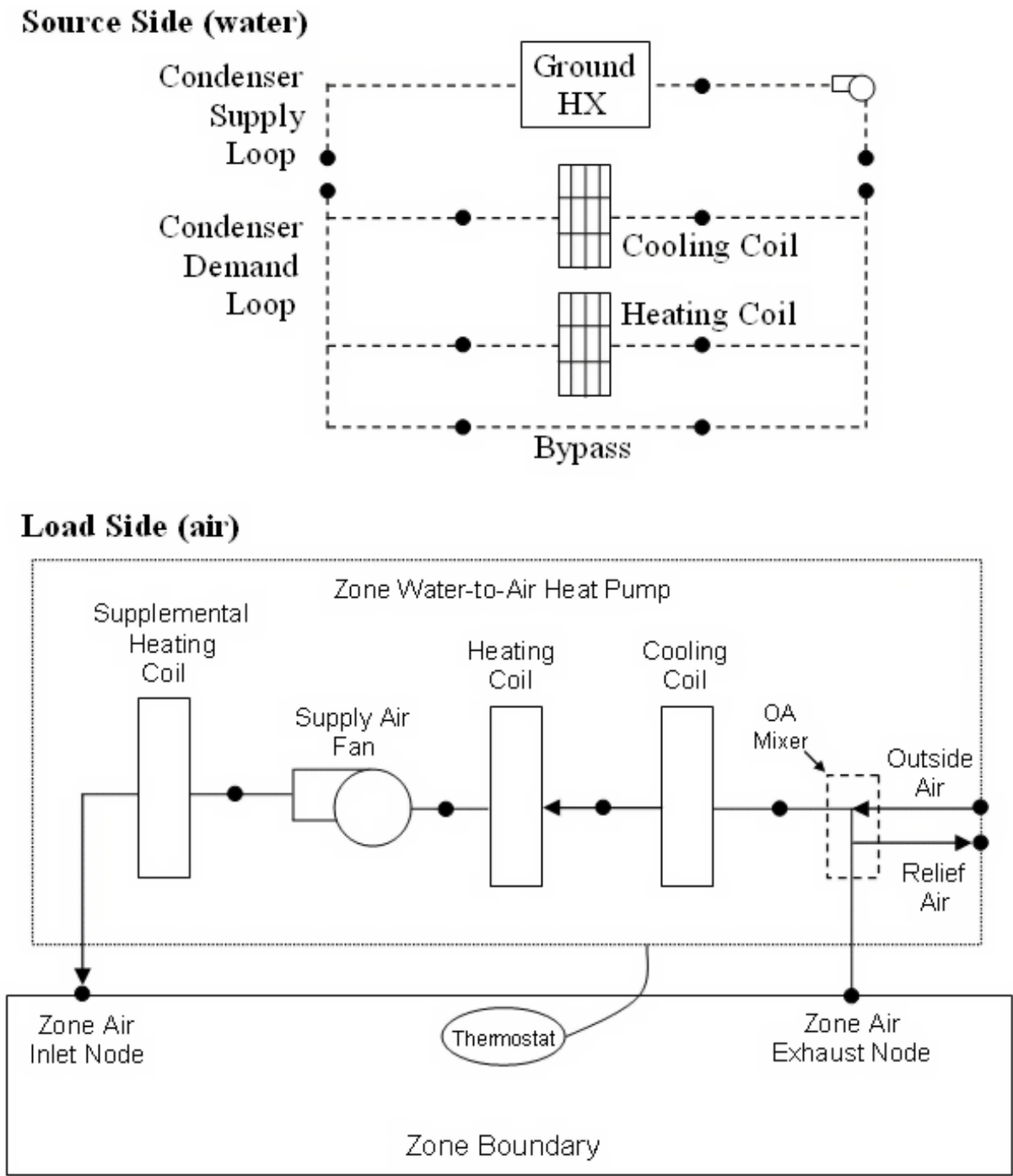
Figure 1.144: Zone Water to Air Heat Pump Schematic for a DrawThrough Configuration with Ground Heat Exchanger
