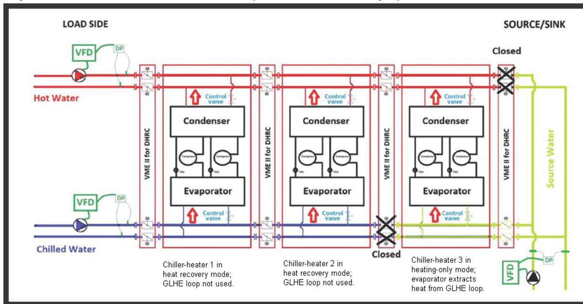
Figure 1.100: Diagram of a central heat pump system with two chiller-heaters in heat recovery mode and one chiller-heater in heating-only mode
