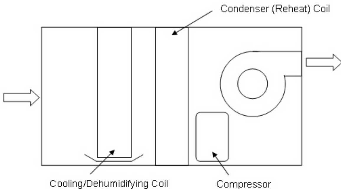
Figure 1.148: Schematic of a mechanical dehumidifier
