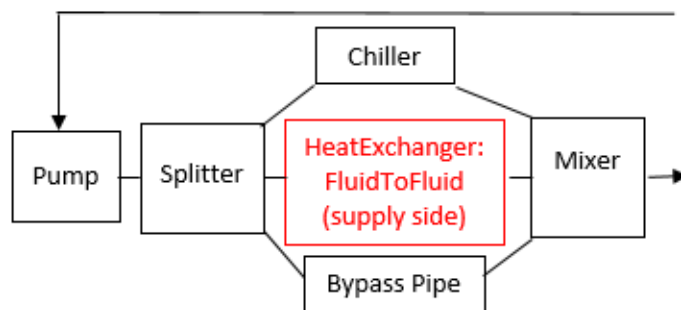
Chilled Water Loop Supply Side Schematic: Parallel HeatExchanger:FluidToFluid Free Cooling Configuration using Control Type = CoolingSetpointOnOffWithComponentOverride (HX demand side connected to condenser loop)
