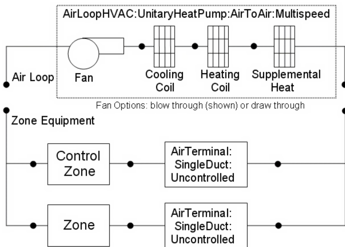
Figure 1.157: Schematic of EnergyPlus Unitary Air-to-Air Multi Speed Heat Pump
