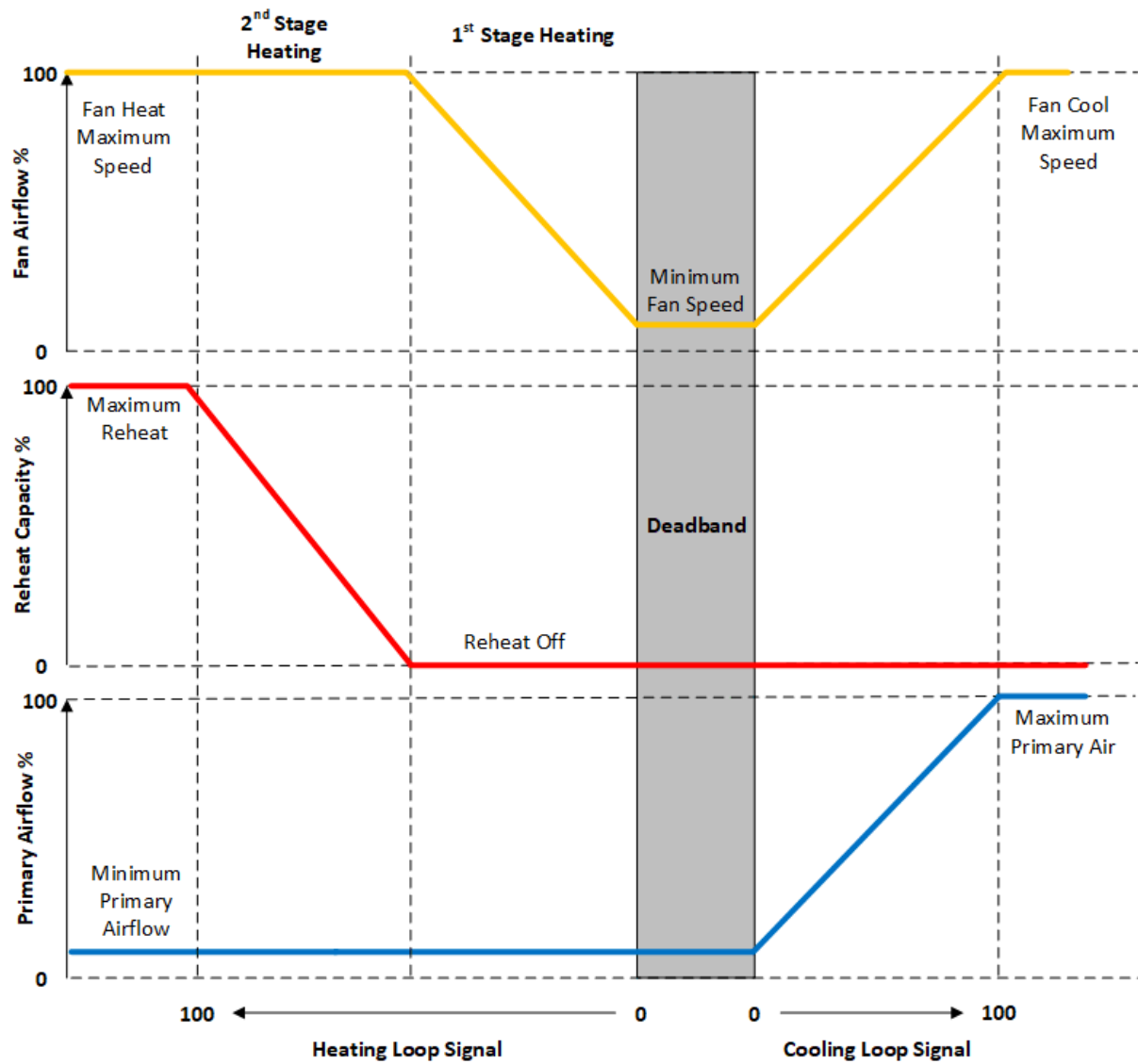
Figure 1.134: Variable Speed Fan with Staged Heat Control
