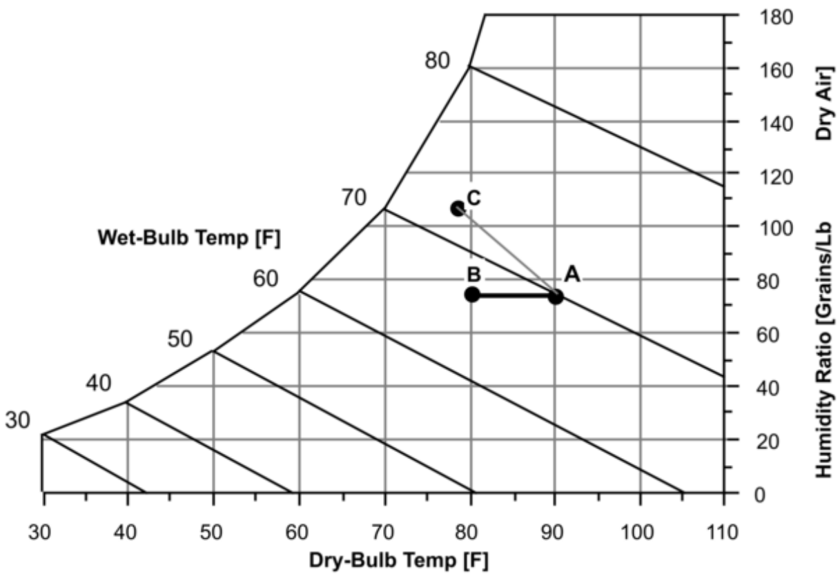
Figure 1.203: Secondary Air Process Indirect Wet Coil Evap Cooler
