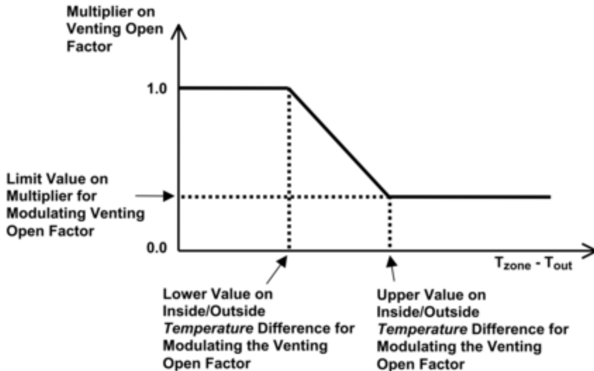
Figure 1.121: Modulation of venting area according to inside-outside temperature difference.
