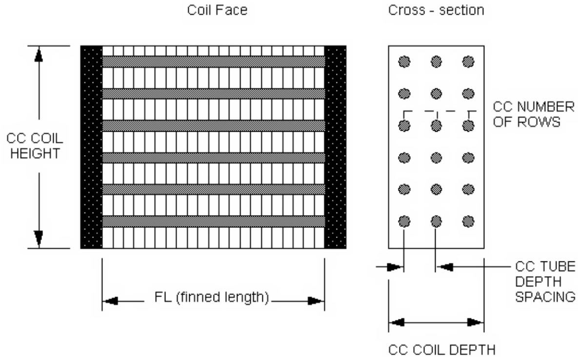
Figure 1.176: Geometry of a Cooling Coil (CC)
