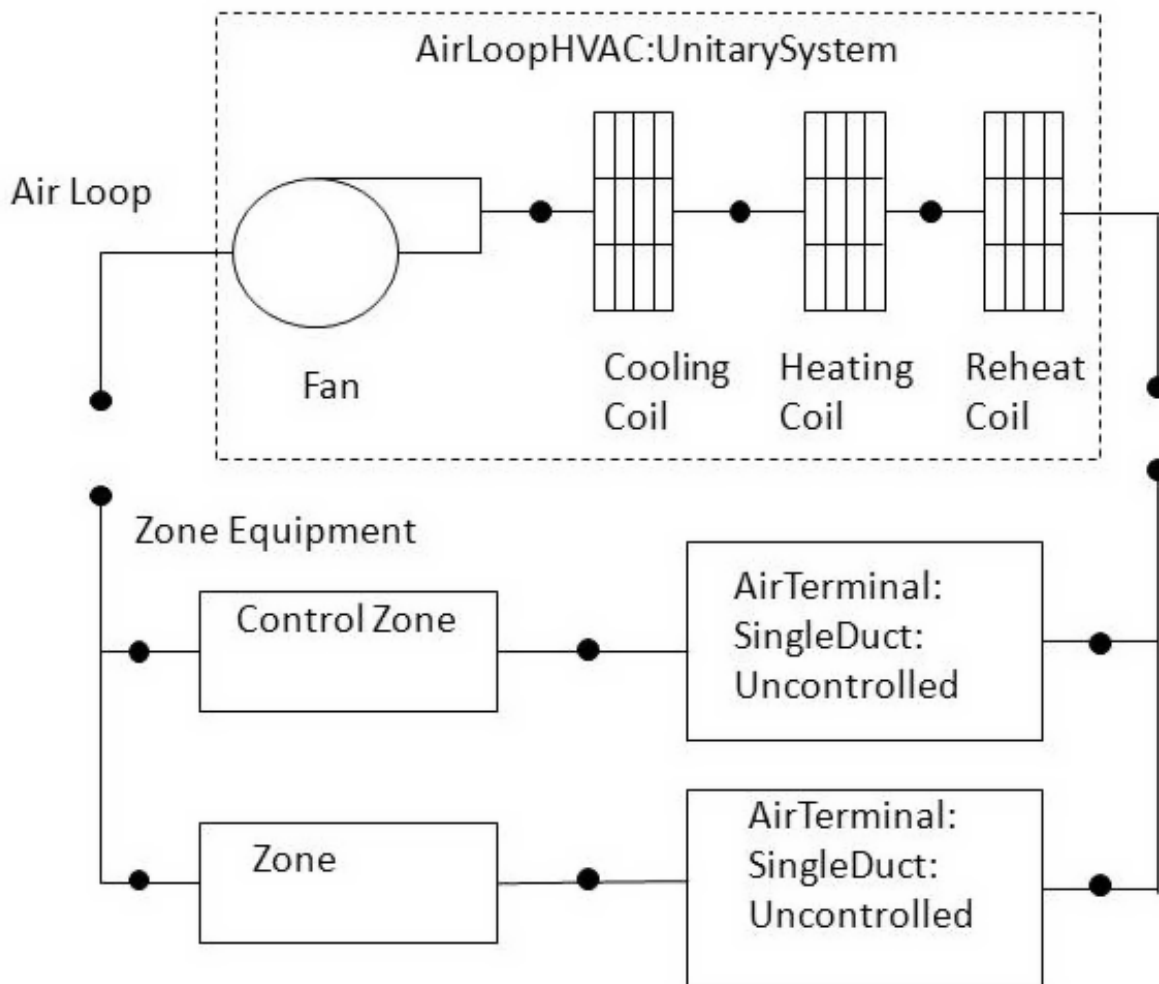
Figure 1.153: Schematic of the EnergyPlus Unitary System
