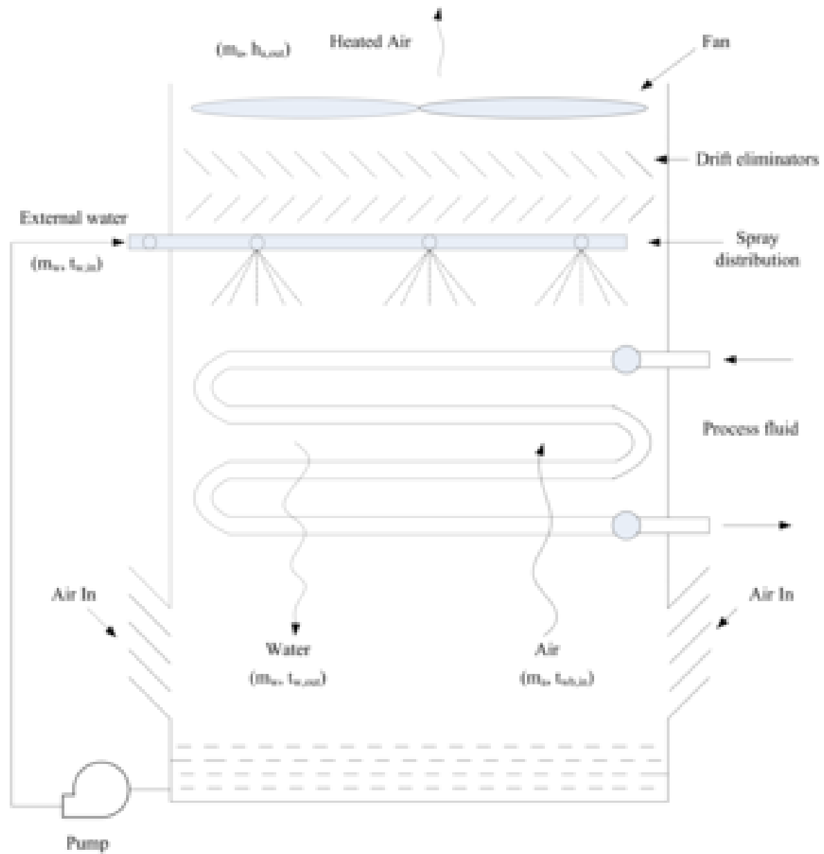
Figure 1.103: Schematic diagram for evaporative fluid cooler
