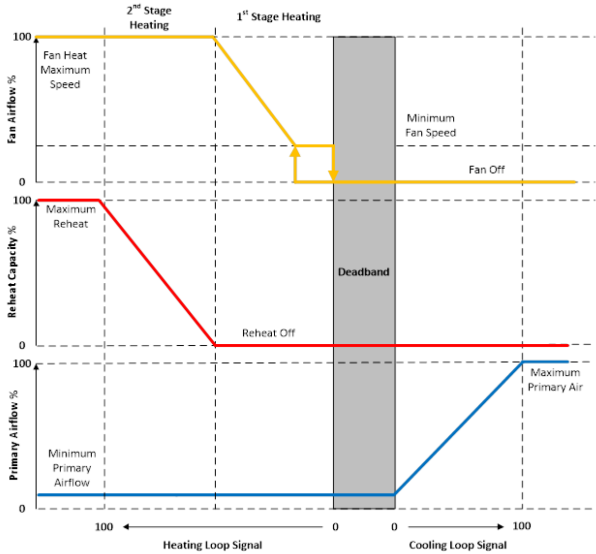
Figure 1.137: Variable Speed Fan with Staged Heat Control
