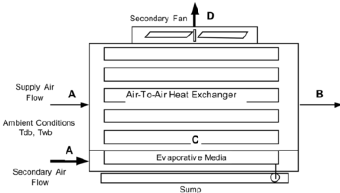
Figure 1.200: Evaporative Cooler – Indirect Dry Coil
