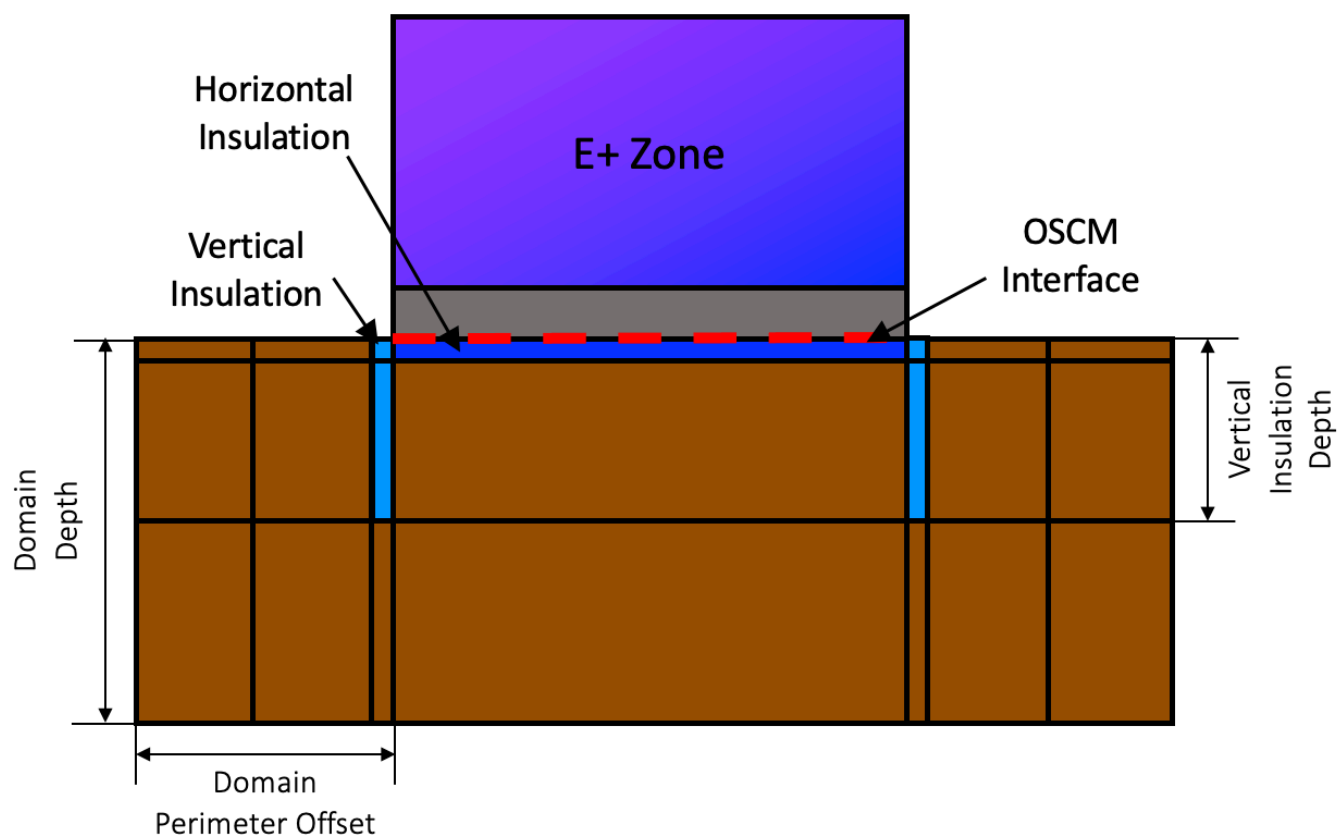
Figure 1.8: On-grade configuration
