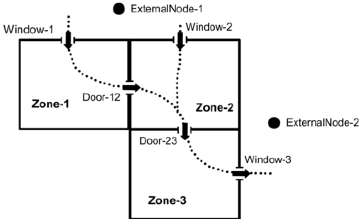
Figure 1.118: Plan view of a simple air flow network showing a possible air flow pattern in which all of the windows and doors are open.
