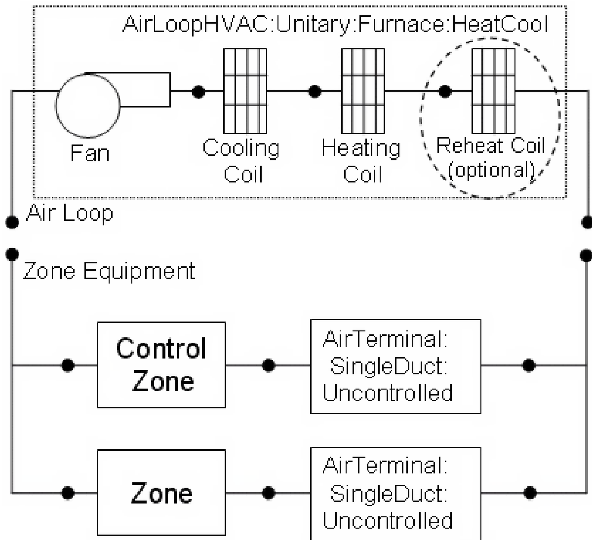
Figure 1.154: Schematic of EnergyPlus Heat/Cool Furnace
