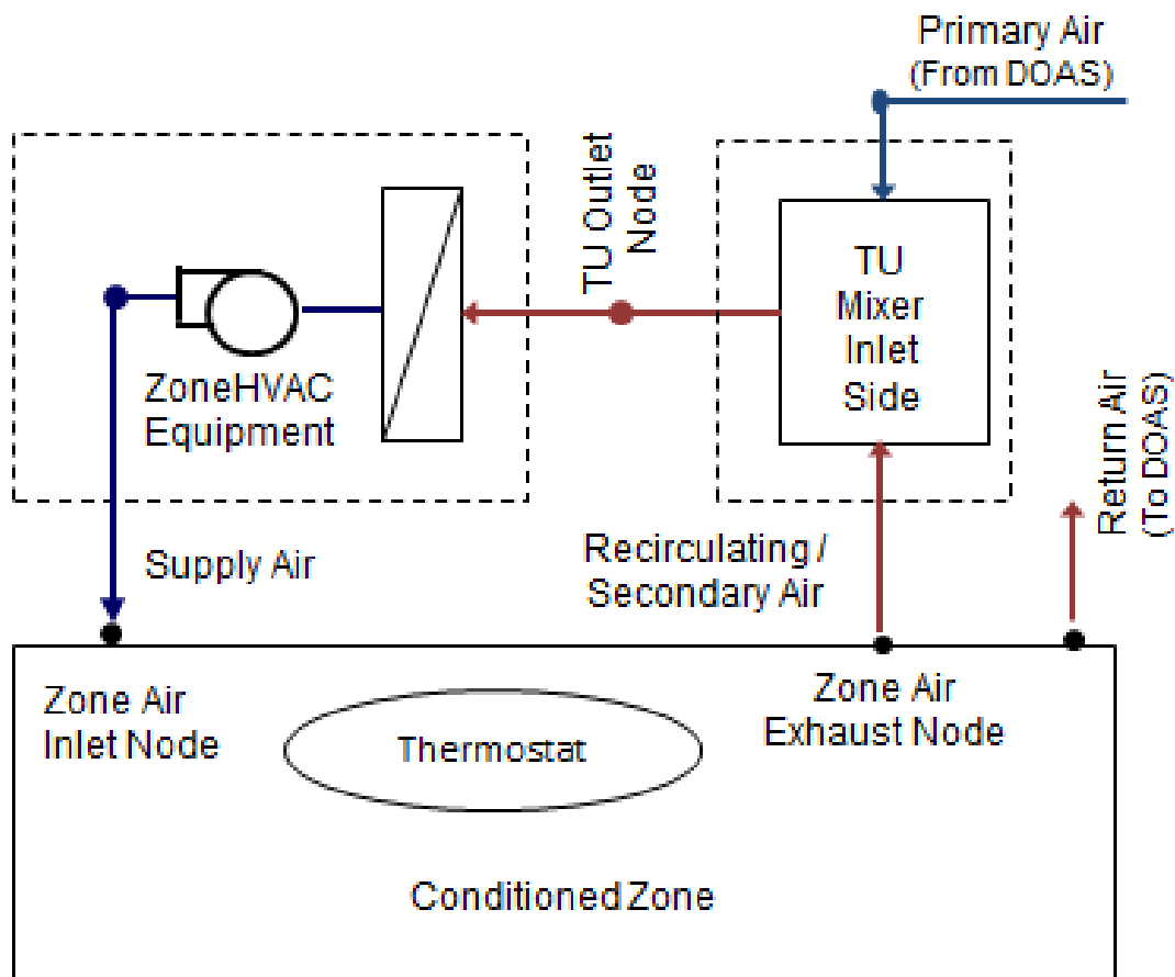
Figure 1.139: Inlet Side Mixer Air Terminal Unit with ZoneHVAC Equipment
