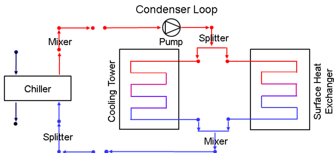
Figure 1.110: Surface Ground Heat Exchanger with other heat exchangers on condenser loop
