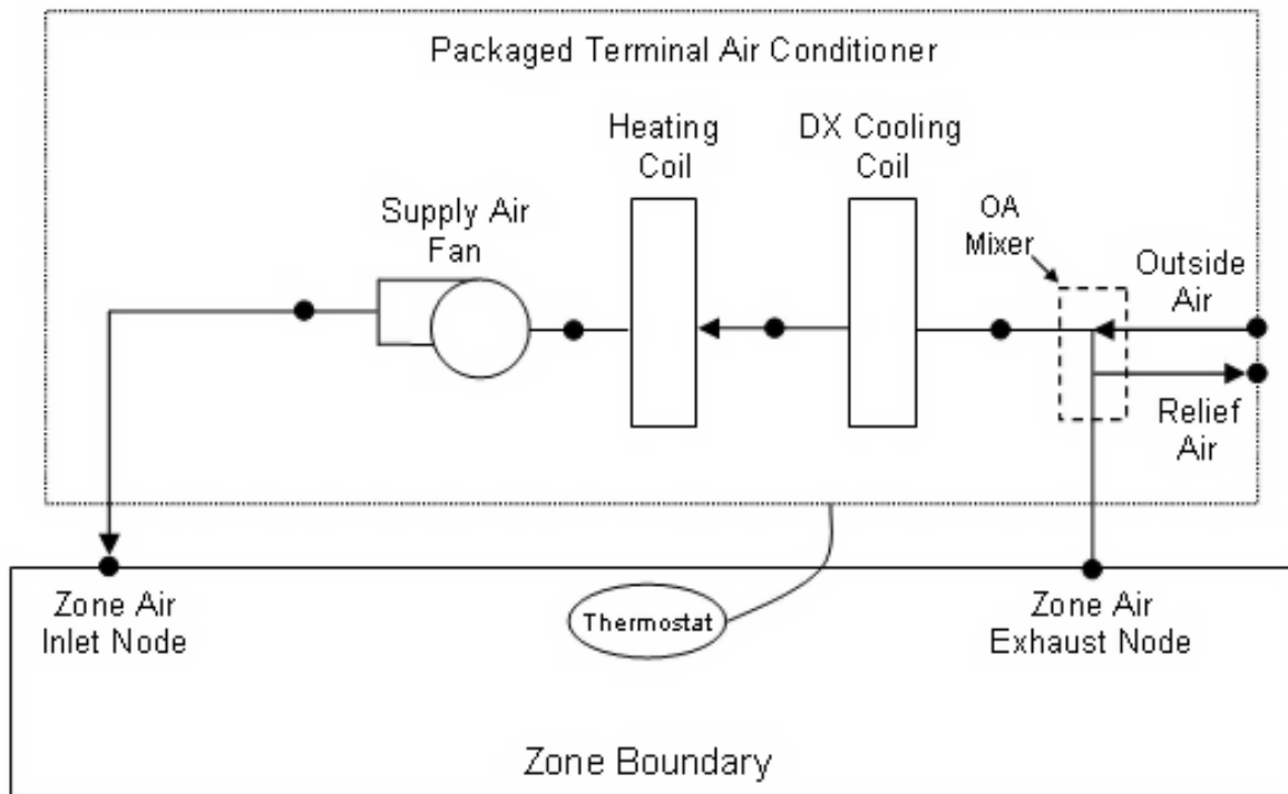
Figure 1.142: Schematic of a packaged terminal air conditioner with draw through fan placement
