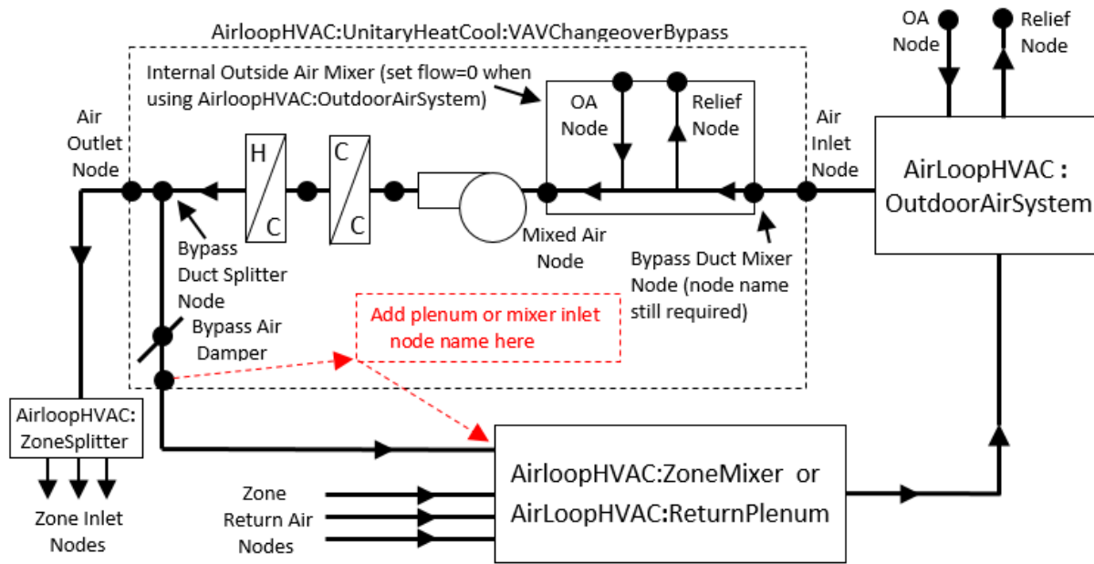
Figure 1.163: Schematic of a CBVAV unitary system used with outdoor air system
