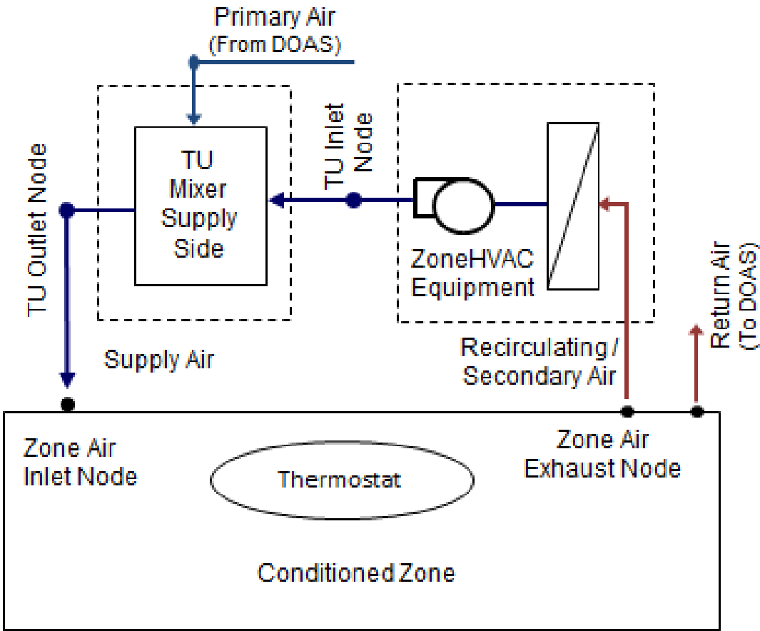
Figure 1.140: Supply Side Mixer Air Terminal Unit with ZoneHVAC equipment
