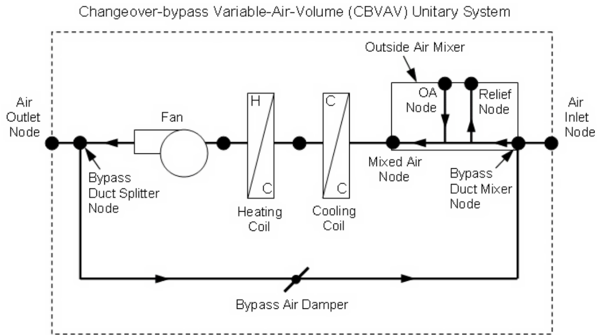
Figure 1.161: Schematic of a CBVAV unitary system (draw through fan placement)
