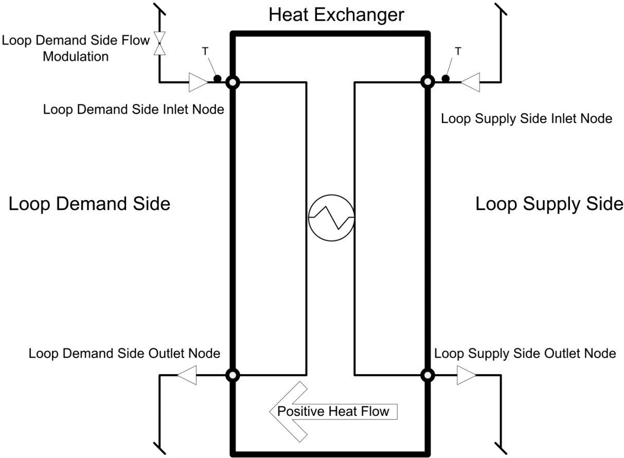
Figure 1.111: Plant Fluid-to-Fluid Heat Exchanger
