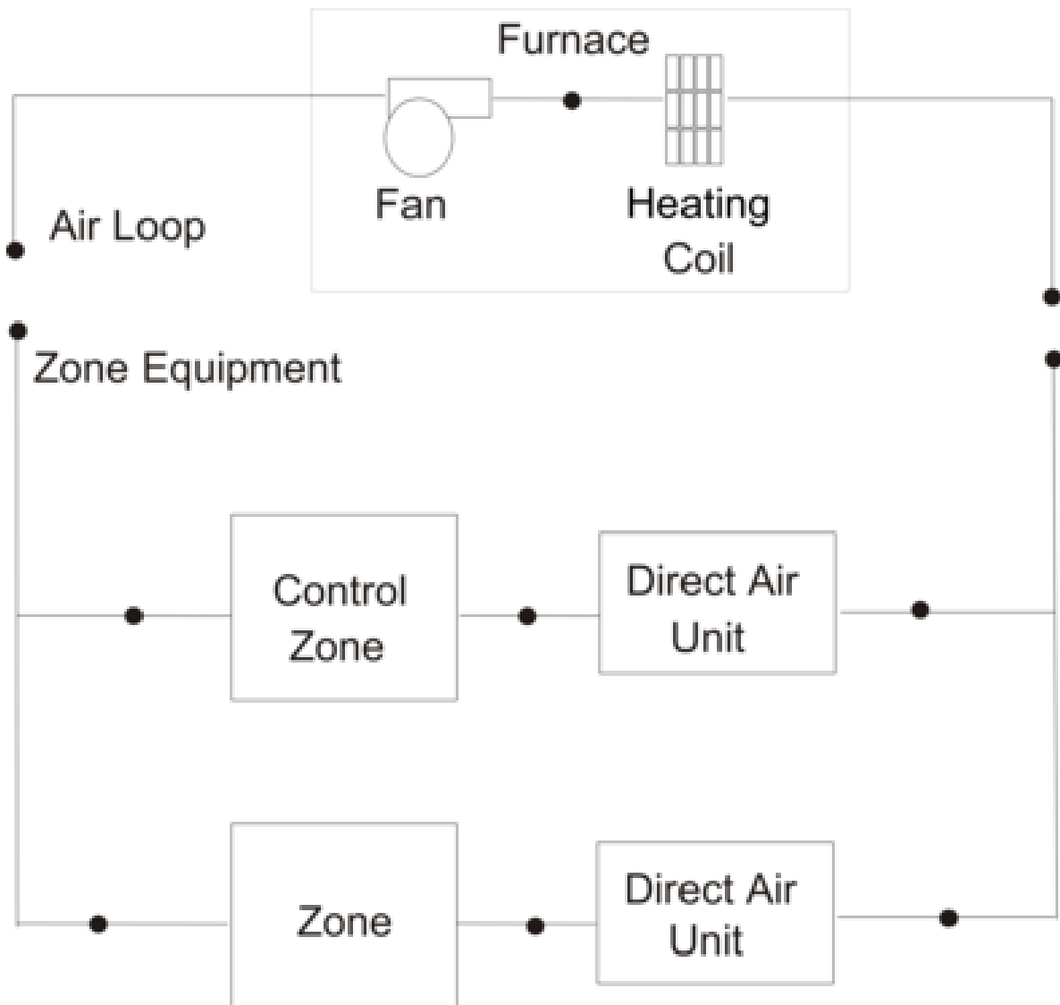
Figure 1.158: Schematic of Blow Through Furnace Model
