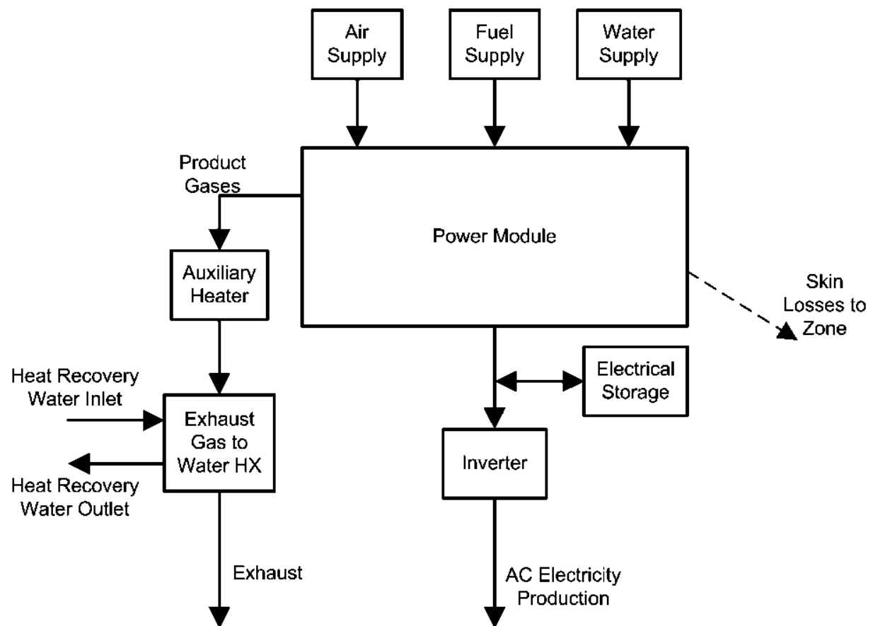
Figure 1.212: Fuel cell subsystems.
