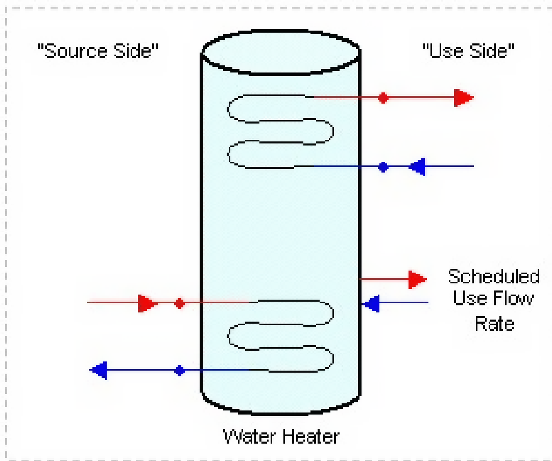
Figure 1.101: Water Heater Configuration
