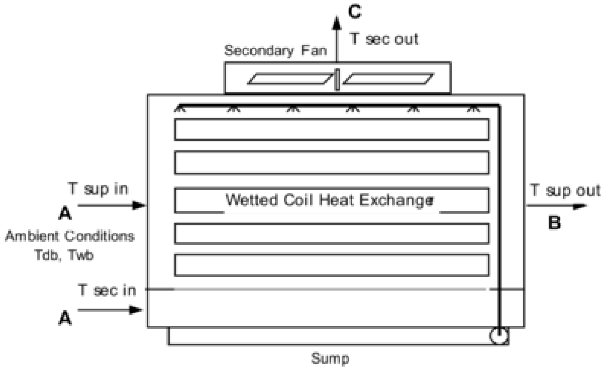
Figure 1.202: Evaporative Cooler Indirect Wet Coil
