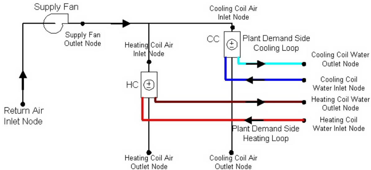
Figure 1.175: Example Air Loop Heating &amp; Cooling Coil
