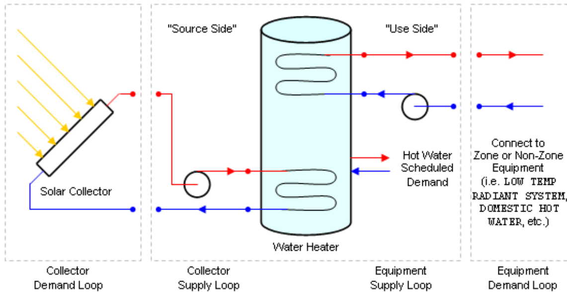
Figure 1.171: Solar Collector Plant Loop Connection Diagram
