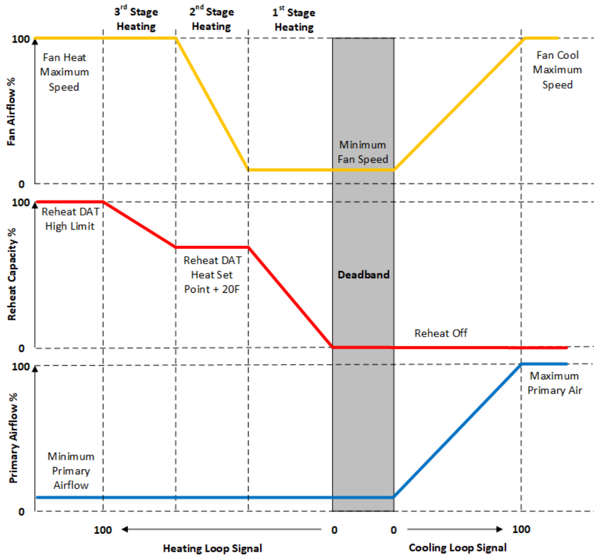
Figure 1.135: Variable Speed Fan with Modulated Heat Control
