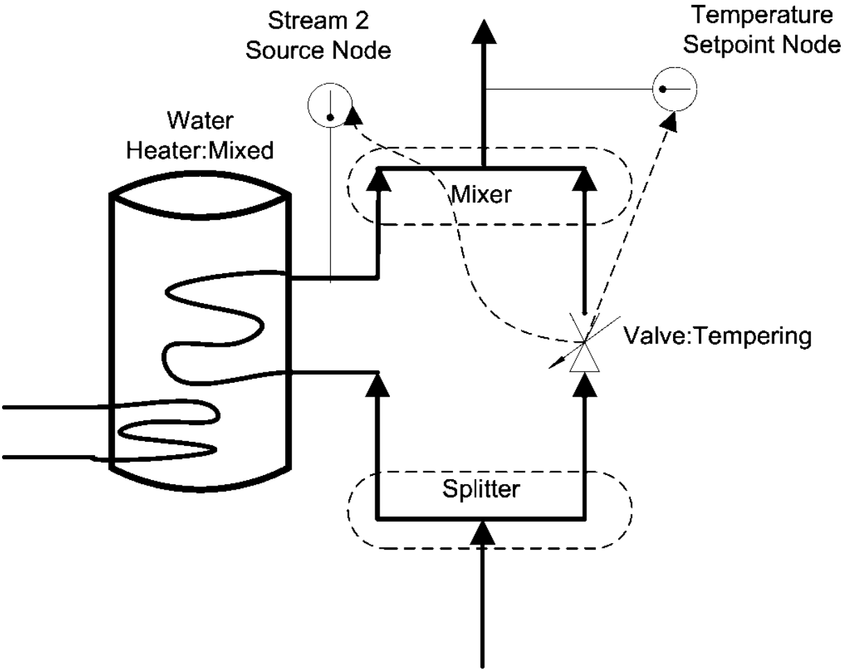
Figure 1.174: Tempering Valve Schematic
