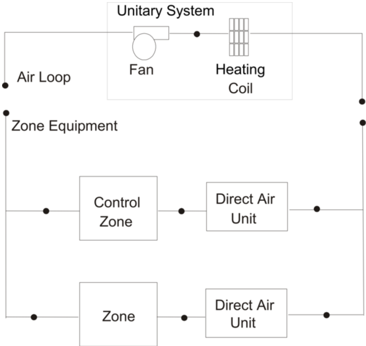
Figure 1.159: Schematic of Blow Through Heat-Only Unitary System
