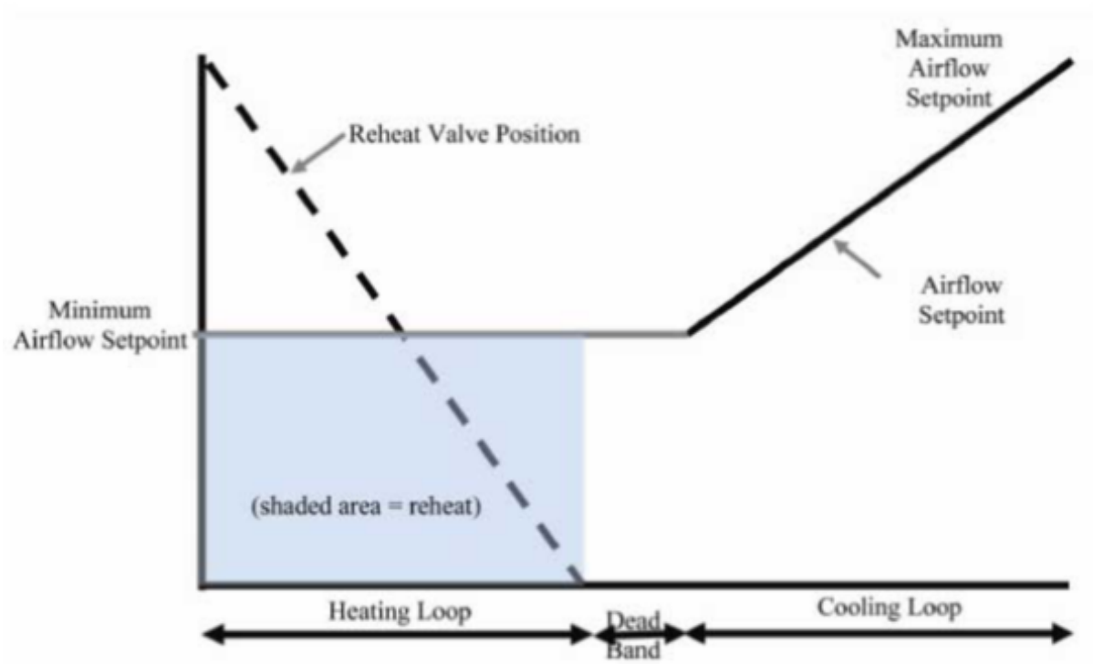
Figure 1.129: The Single Maximum Control Logic
