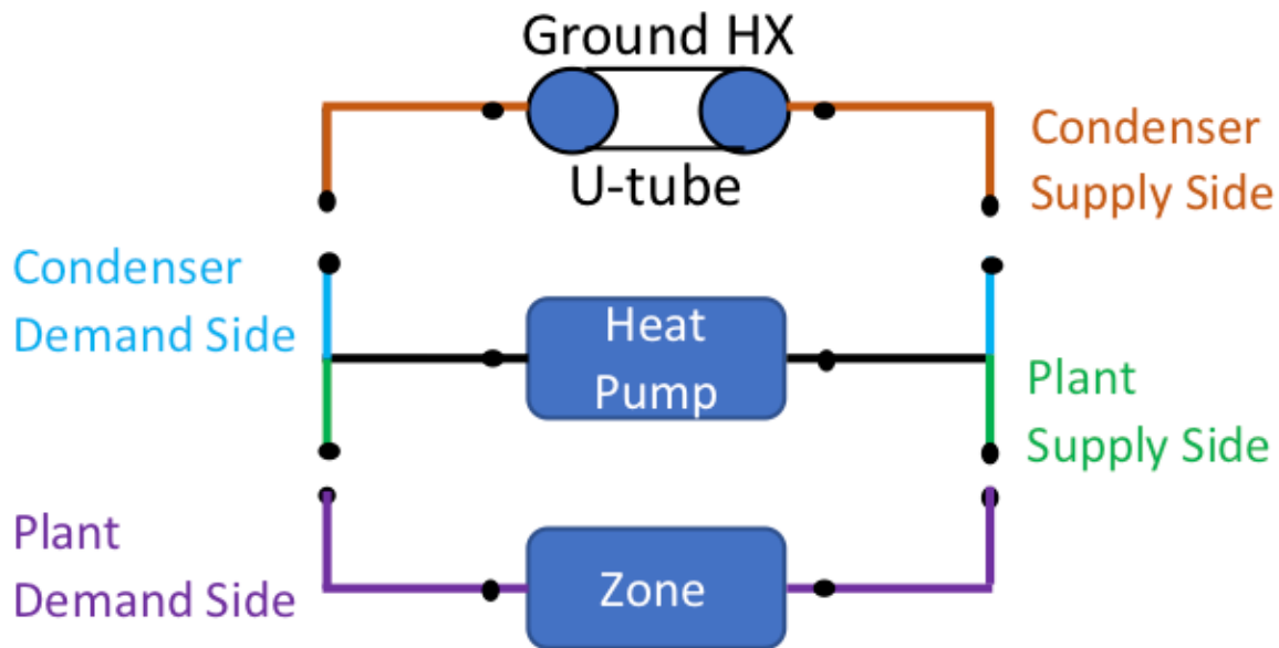
Figure 1.96: Schematic of EnergyPlus Ground Loop Heat Exchanger
