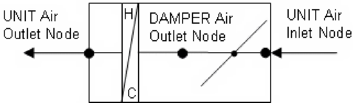
Figure 1.131: Single Duct VAV Heat and Cool Reheat Schematic
