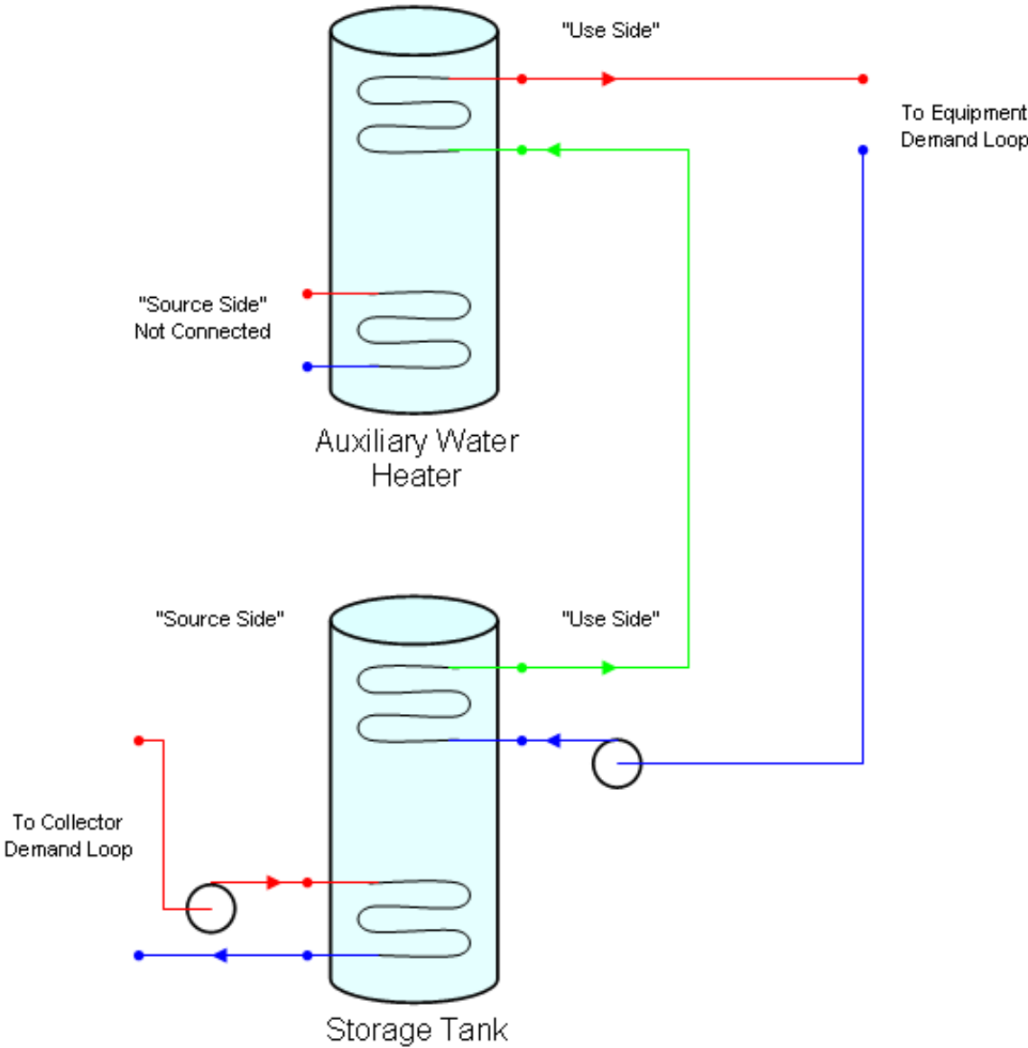
Figure 1.172: Two-Tank Solar Heating System Connection Diagram
