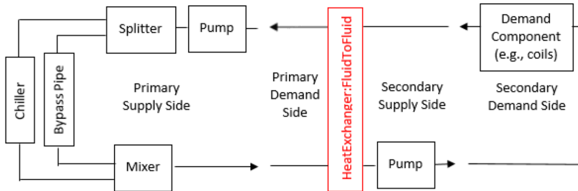
Primary Secondary Plant Schematic: HeatExchanger:FluidToFluid as Primary Plant Demand Side Component and Secondary Plant Supply Side Component using Control Type = CoolingSetpointModulated
