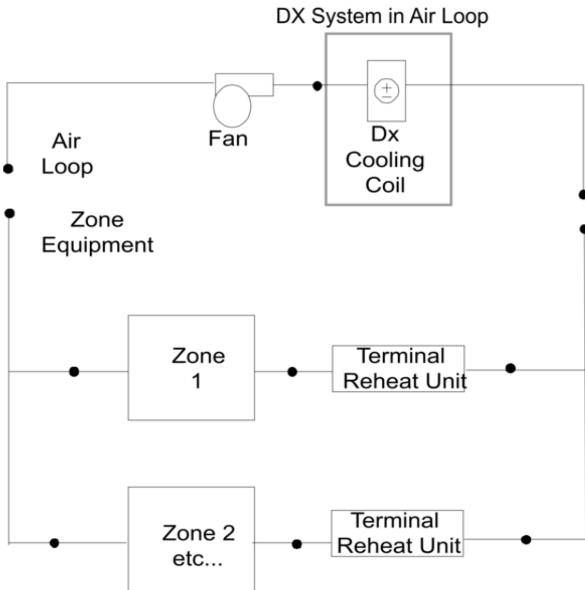
Figure 1.184: Schematic of CoilSystem:Cooling:DX Object in an Air Loop for a Blow Through Application
