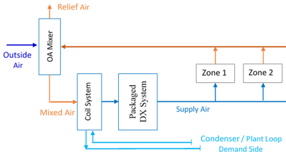
Figure 1.179: Water Side Economizer Coil System Upstream of Packaged DX System
