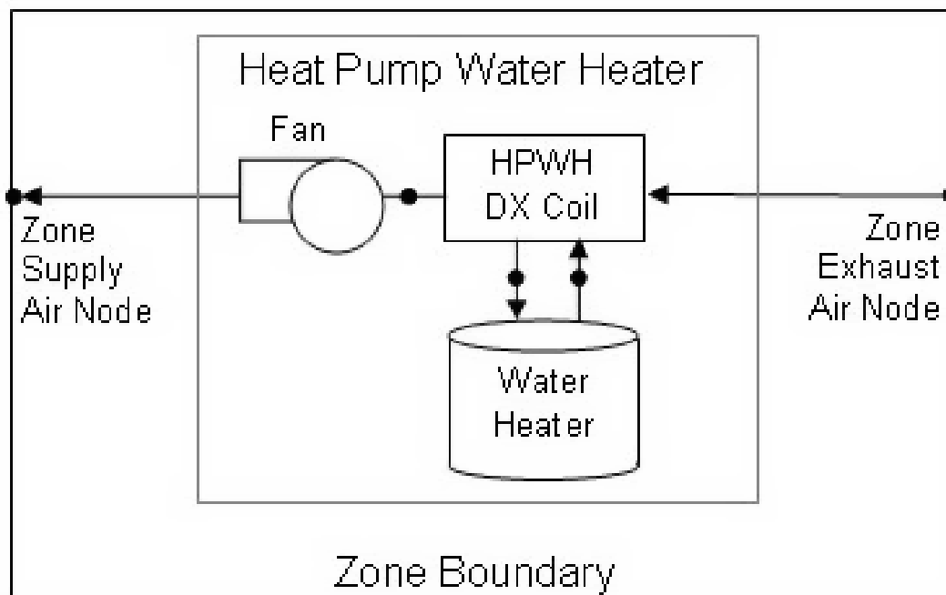
Figure 1.102: Schematic diagram for a heat pump water heater located in a zone
