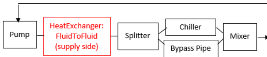
Chilled Water Loop Supply Side Schematic: Series HeatExchanger:FluidToFluid Economizer Configuration using Control Type = CoolingSetpointModulated or CoolingDifferentialOnOff (HX demand side connected to condenser loop)
