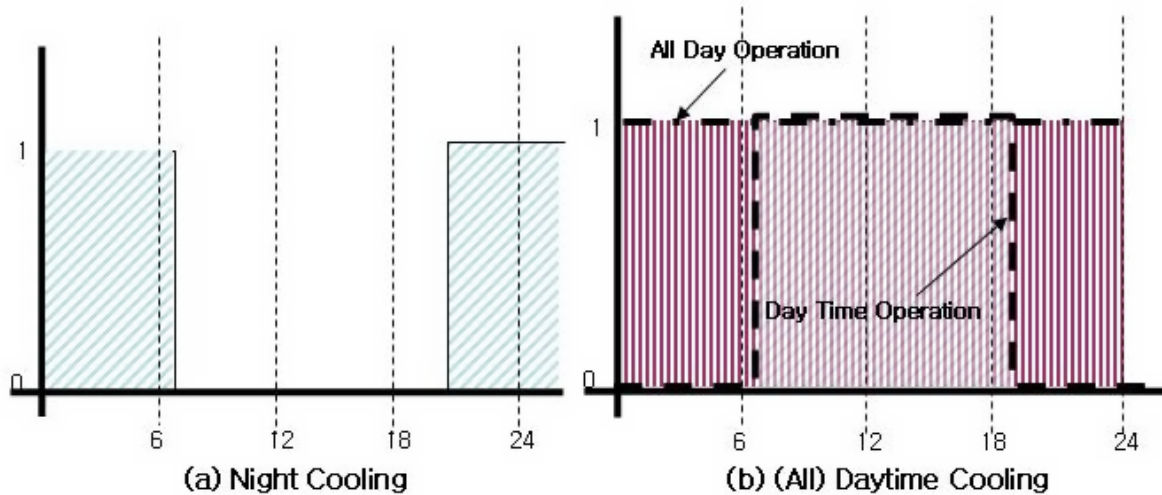
Figure 1.168: Example operating schedule for Ventilated Slab
