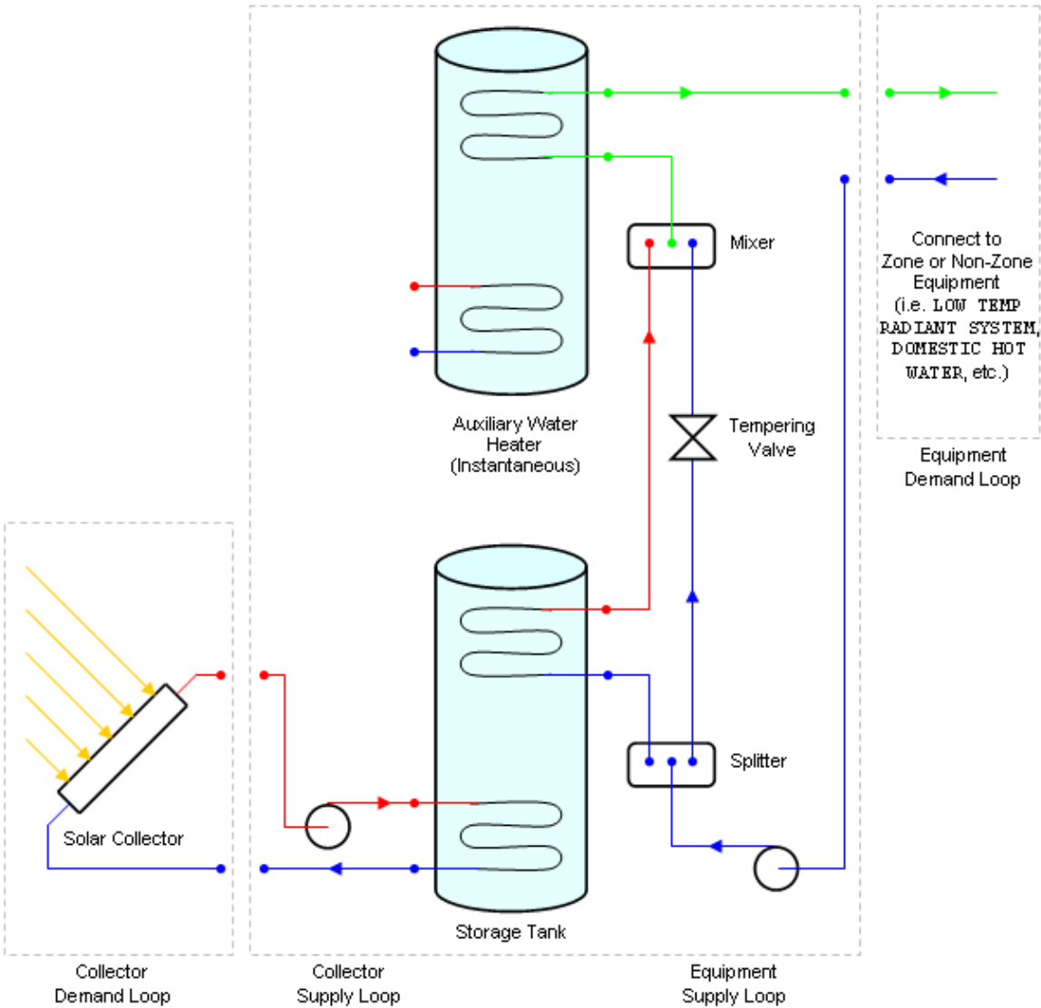
Figure 1.173: Two-Tank Solar Heating System with Tempering Valve
