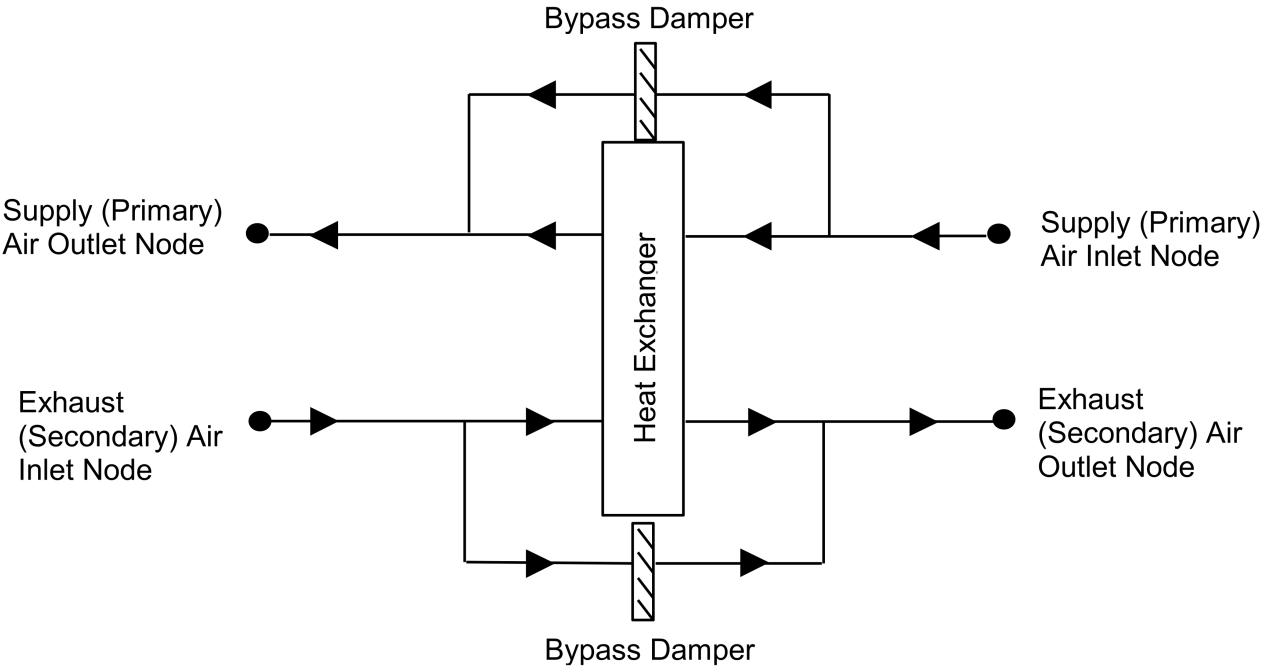
Figure 1.204: Schematic of the Sensible and Latent Air-to-Air Heat Exchanger
