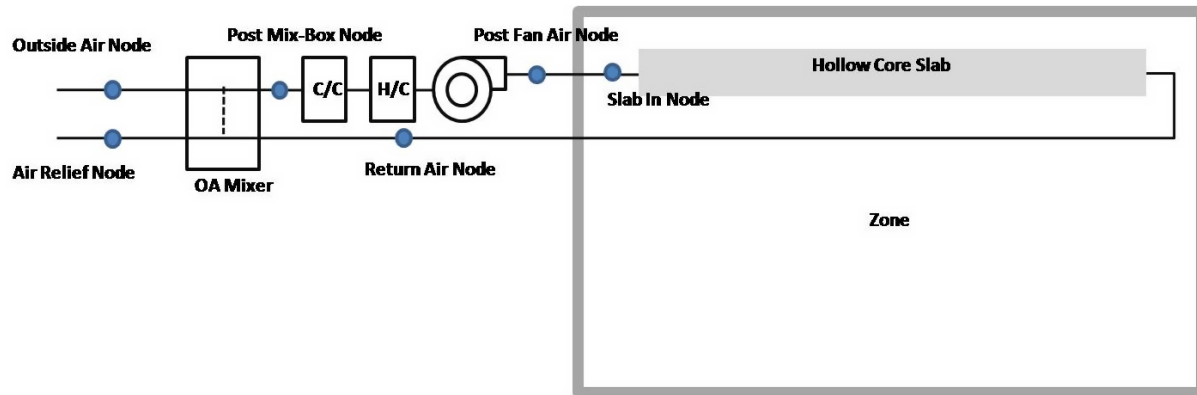
Figure 1.167: Ventilated Slab model - basic system
