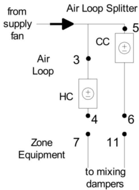
Figure 1.126: Air Loop/Zone Equipment Node Diagram
