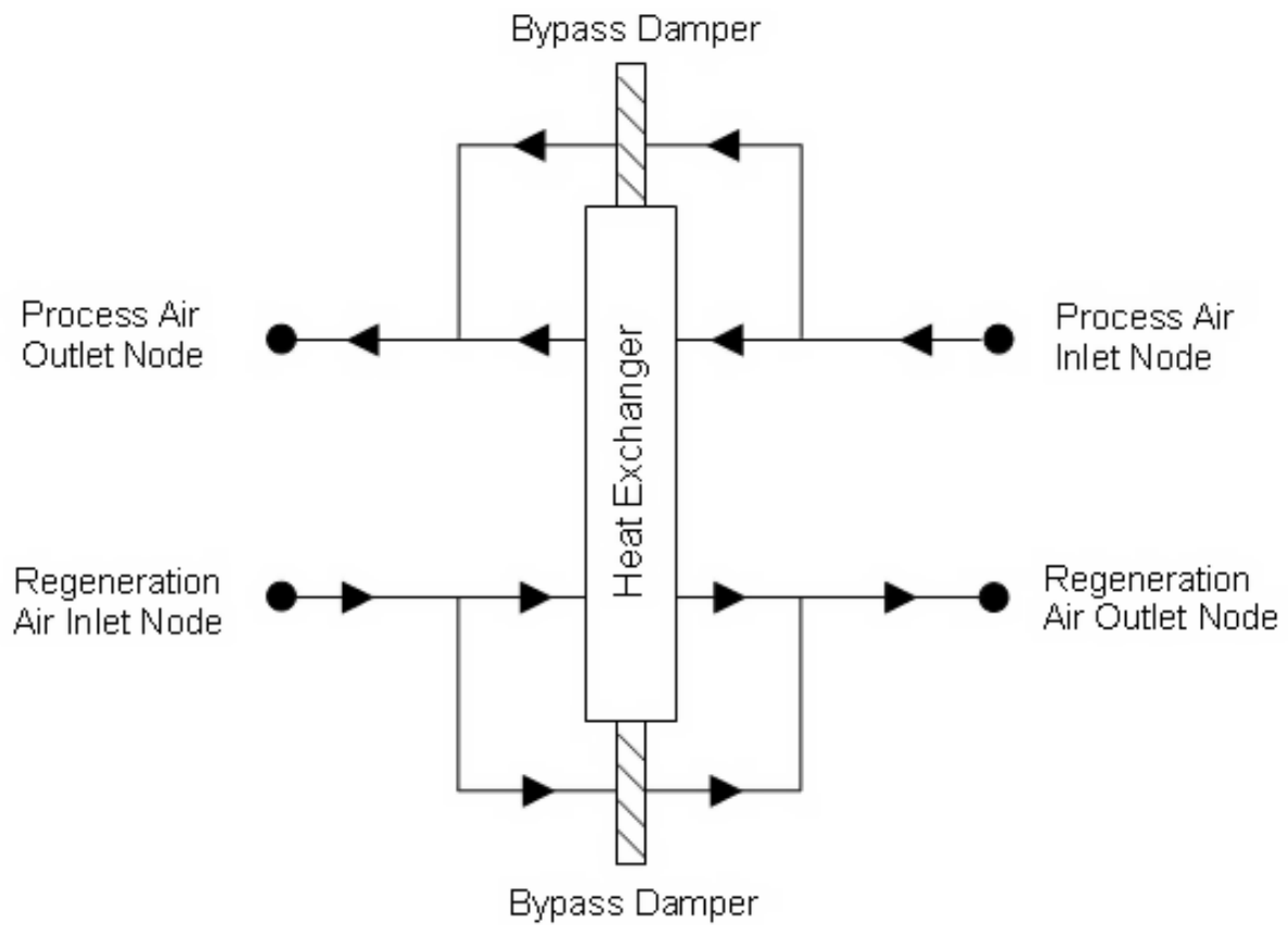
Figure 1.205: Schematic of the Balanced Flow Desiccant Heat Exchanger
