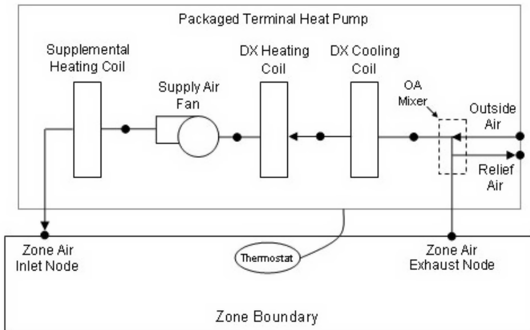
Figure 1.143: Schematic of a packaged terminal heat pump (draw through fan placement)
