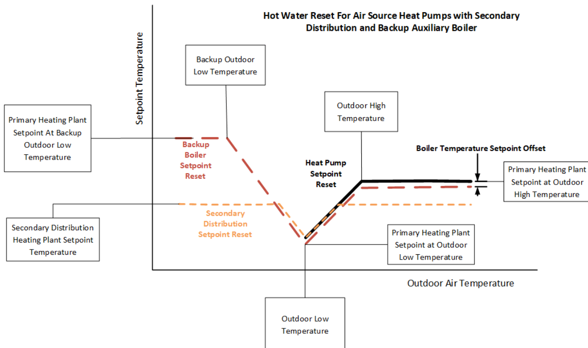
Figure 1.93: Hot Water Temperature Setpoint Vs Outdoor Air Temperature
