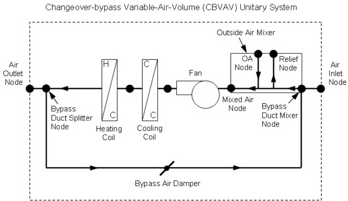
Figure 1.162: Schematic of a CBVAV unitary system (blow through fan placement)
