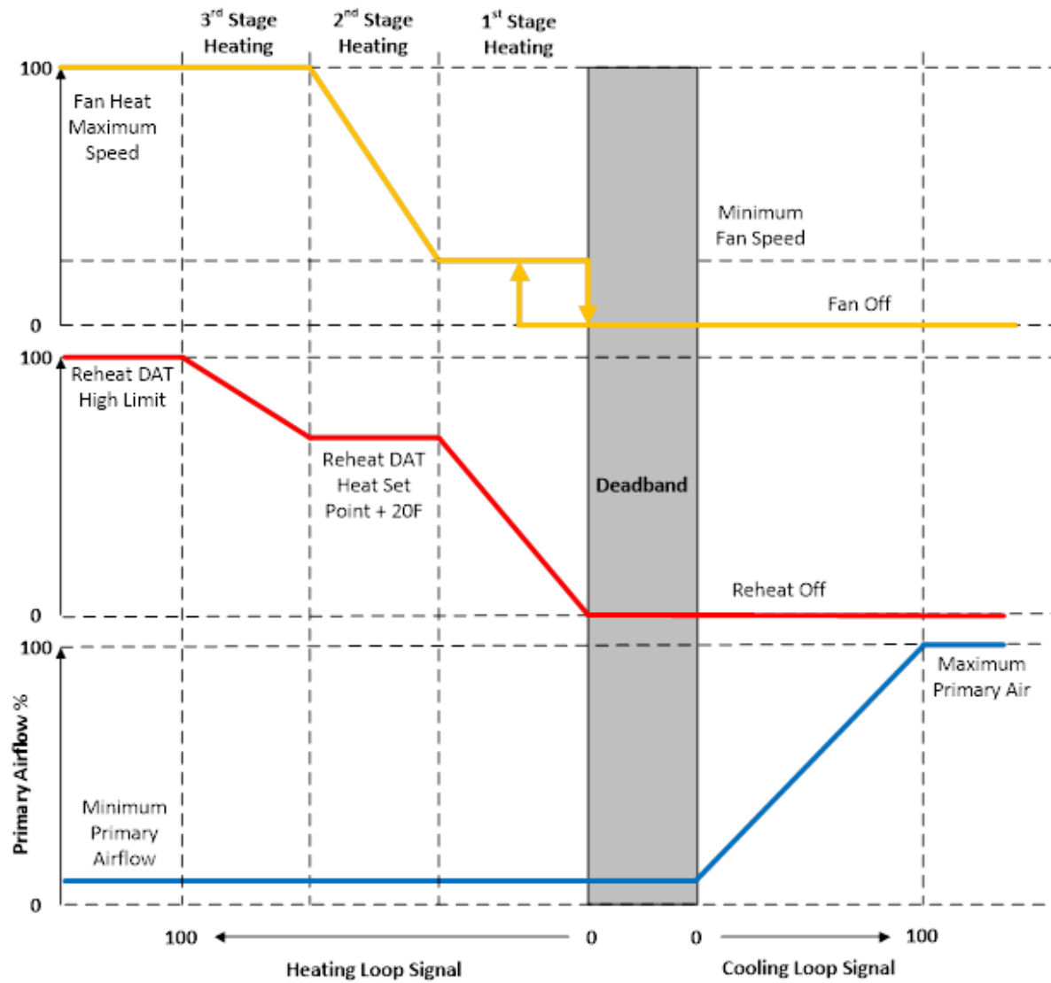
Figure 1.138: Variable Speed Fan with Modulated Heat Control
