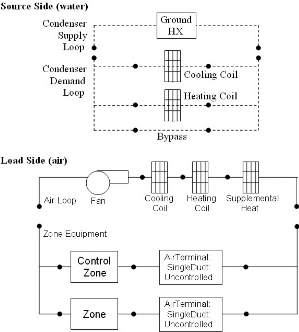
Figure 1.160: Water to Air Heat Pump Schematic for a BlowThrough Configuration with Ground Heat Exchanger
