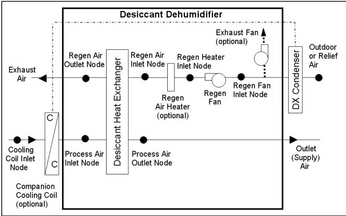
Figure 1.196: Schematic of Dehumidifier:Desiccant:System with Blow Through Regeneration Fan Placement
