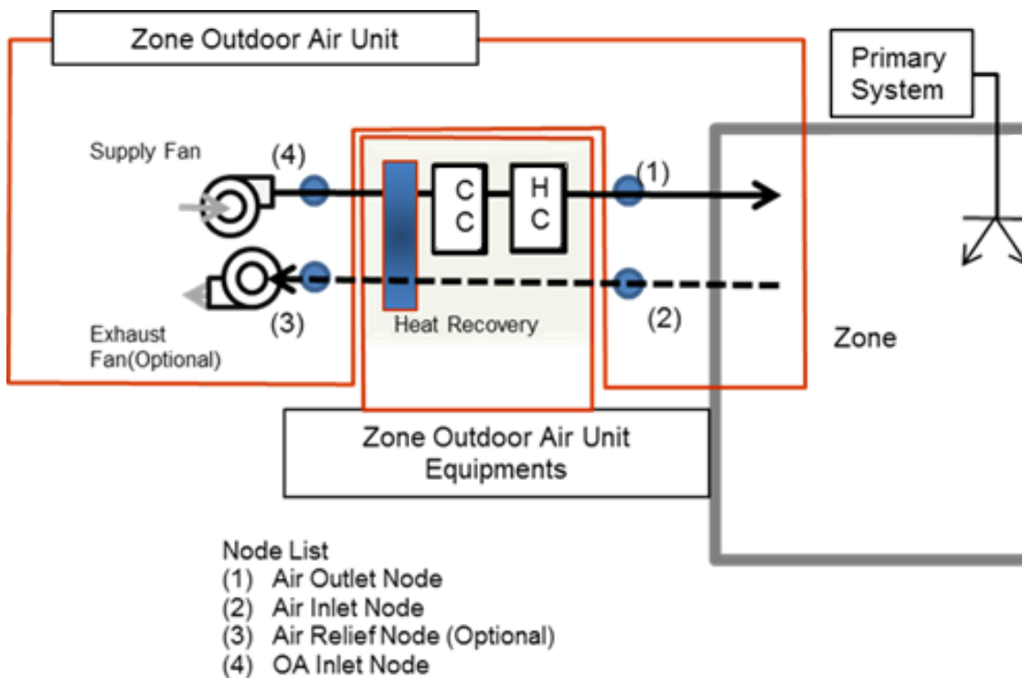
Figure 1.141: Zone Outdoor Air Unit Schematic
