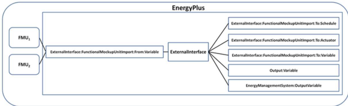
Figure 1.9: Architecture of the FMU for co-simulation import.
