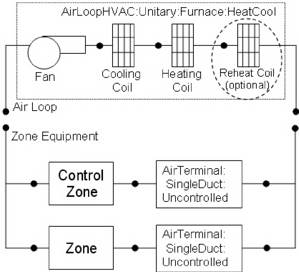
Figure 1.156: Schematic of EnergyPlus Heat/Cool Furnace
