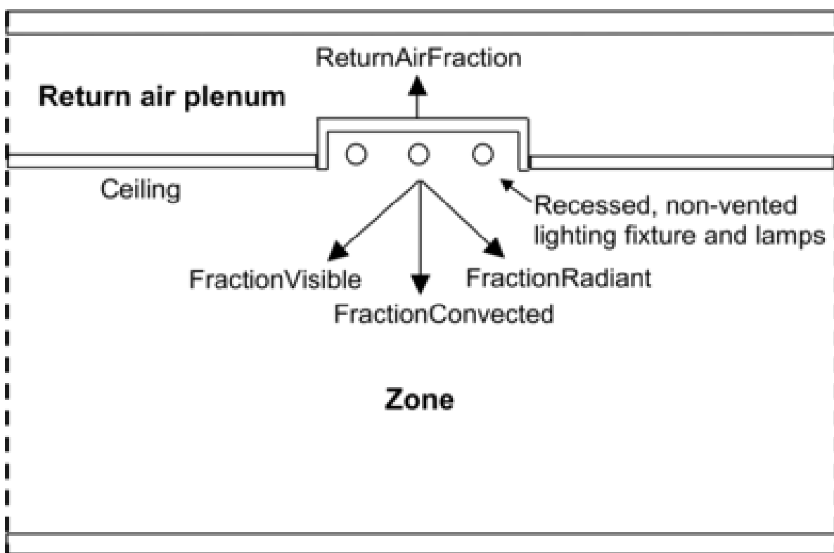
Figure 1.74: Vertical section through a zone and its return air plenum showing recessed lighting (not to scale). The heat from lights is divided into four fractions, three of which— ReturnAirFraction , FractionRadiant and FractionConvected —depend on plenum air temperature.
