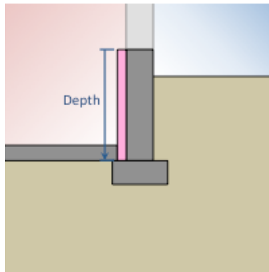
Figure 1.55: Placement of interior vertical insulation
