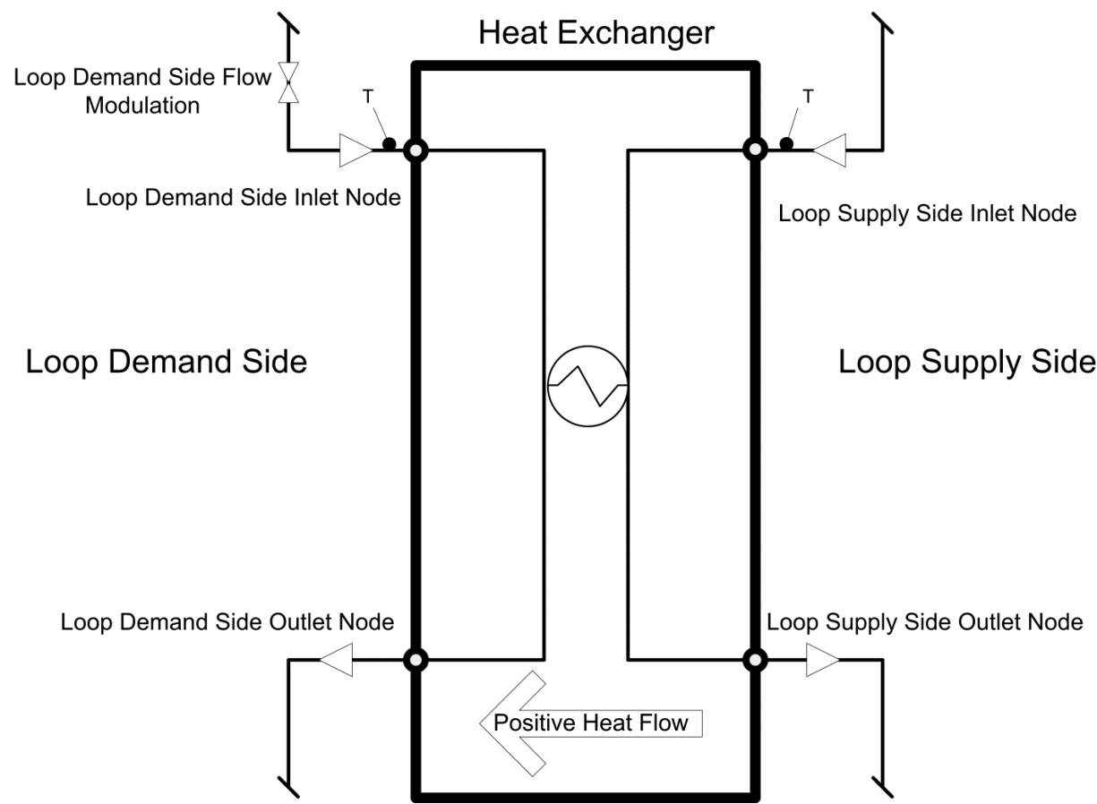
Figure 1.113: Plant Fluid-to-Fluid Heat Exchanger
