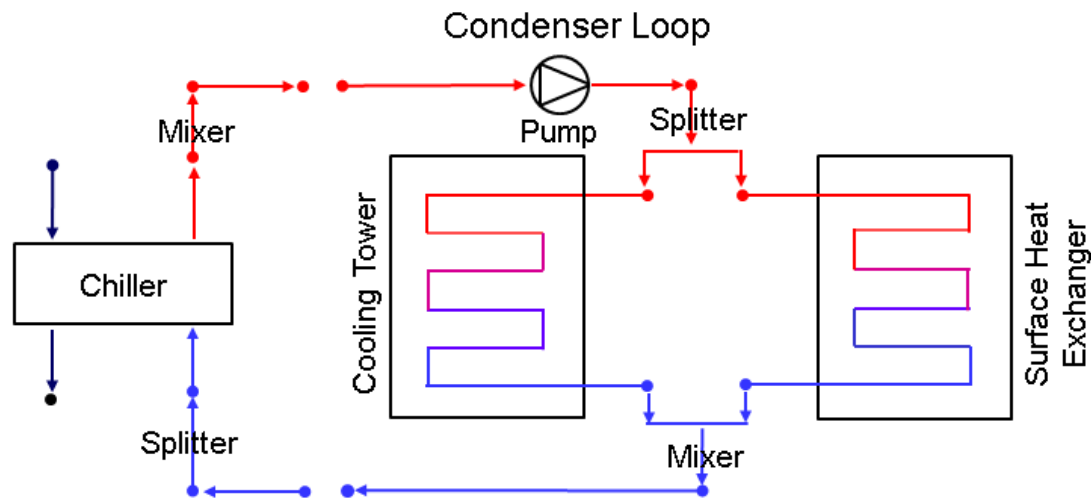
Figure 1.112: Surface Ground Heat Exchanger with other heat exchangers on condenser loop
