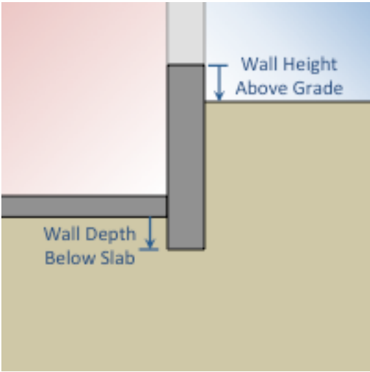
Figure 1.58: Definition of exterior grade and footing wall depth relative to the wall surface (for a basement foundation context)
