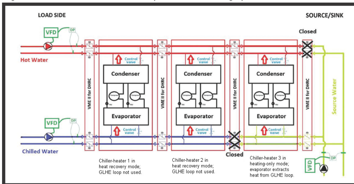
Figure 1.102: Diagram of a central heat pump system with two chiller-heaters in heat recovery mode and one chiller-heater in heating-only mode
