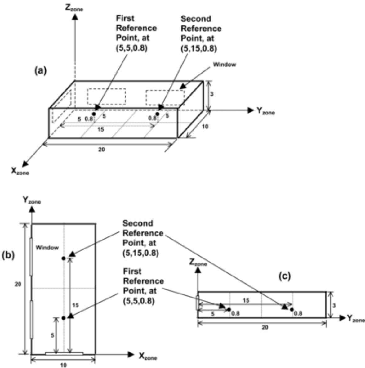
Figure 1.77: Example showing location of daylighting reference points in the zone coordinate system (relative) of a rectangular zone with three windows. (a) Perspective view, (b) plan view, (c) elevation view. All dimensions are in meters.
