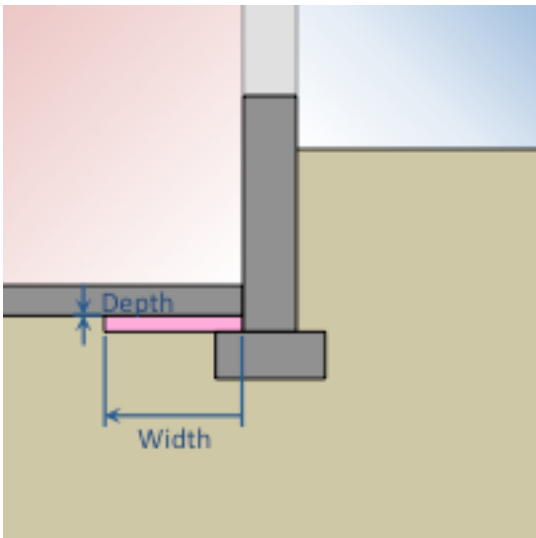
Figure 1.54: Placement of interior horizontal insulation
