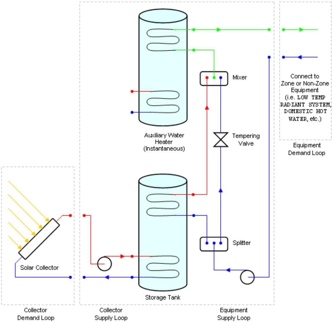
Figure 1.175: Two-Tank Solar Heating System with Tempering Valve
