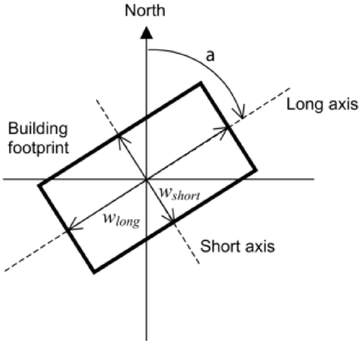
Figure 1.121: Footprint of a rectangular building showing variables used by the program to calculate surface-average wind pressure coefficients. The angle a is the “Azimuth Angle of Long Axis of Building.” w_{short}/w_{long} is the “Ratio of Building Width Along Short Axis to Width Along Long Axis.”
