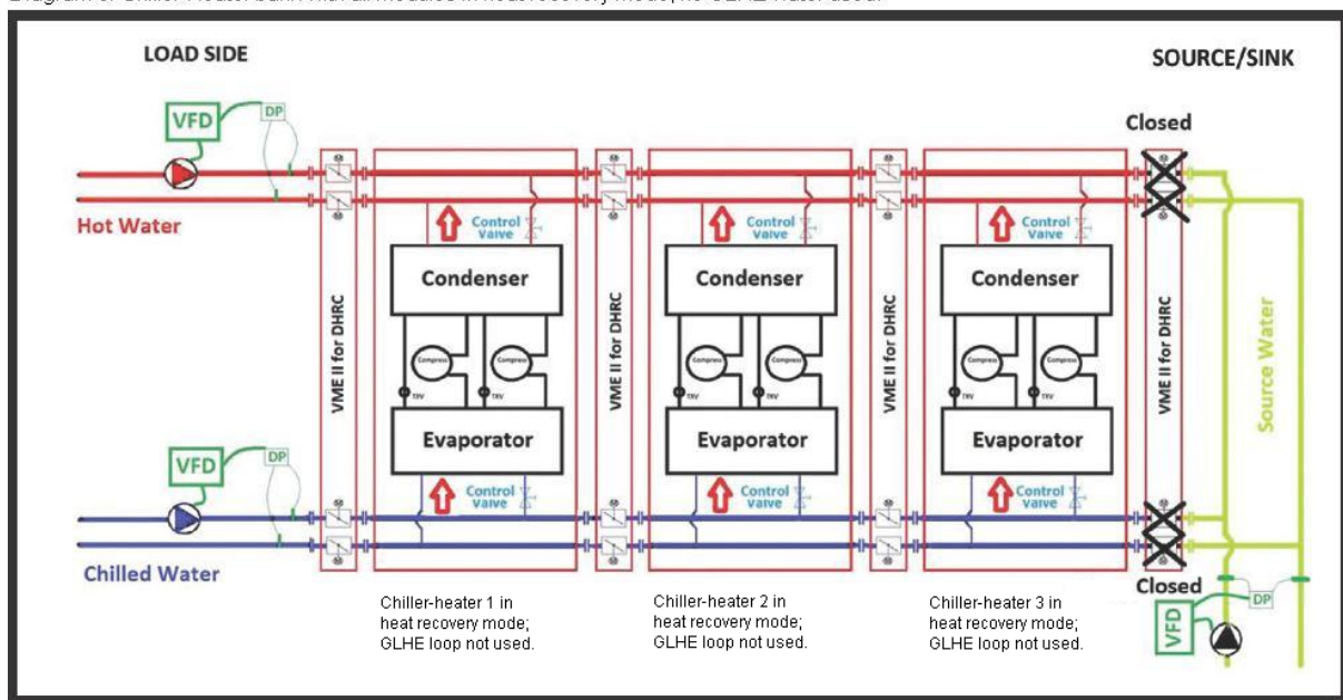
Figure 1.100: Diagram of a central heat pump system with three chiller-heaters in heat recovery mode (No heat is exchanged with the ground source loop)
