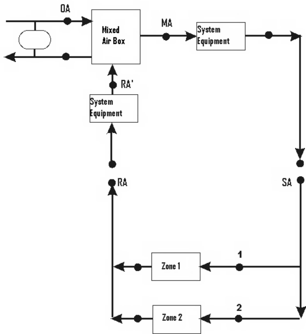
Figure 1.115: Example System for Ventilation Loads Report
