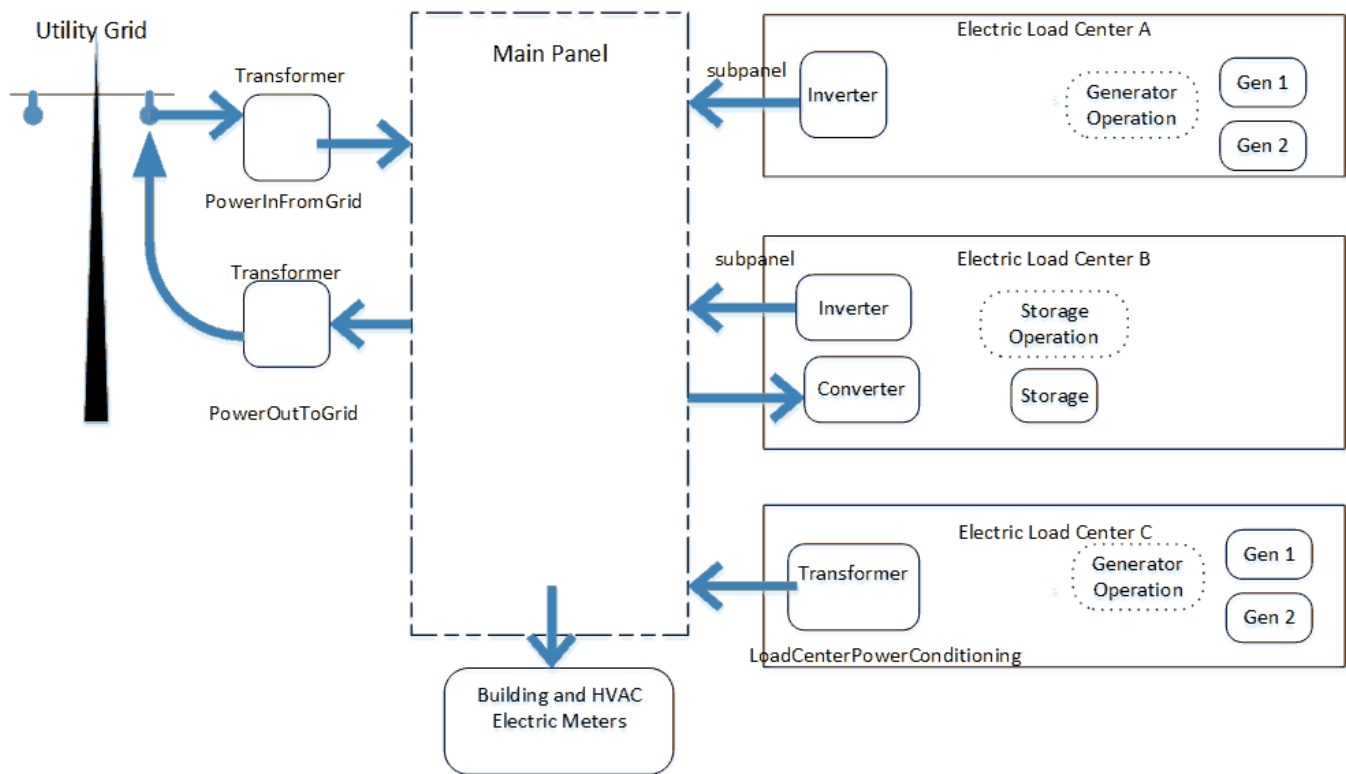
Figure 1.208: PowerServiceOverview
