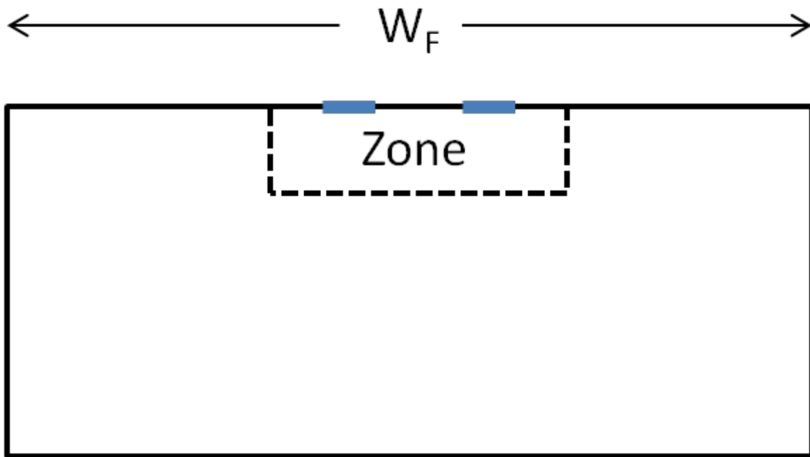
Figure 1.122: Footprint of a rectangular building showing W_F , the “Façade Width”, used by the Single Sided Wind Pressure Coefficient Algorithm.
