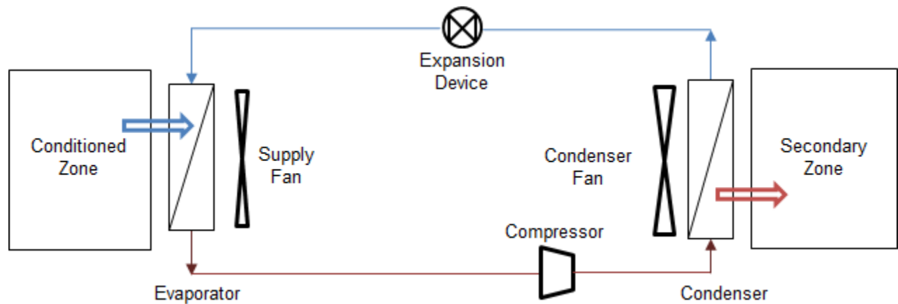
Figure 1.194: Schematic of DX System and heat pump in cooling operating mode
