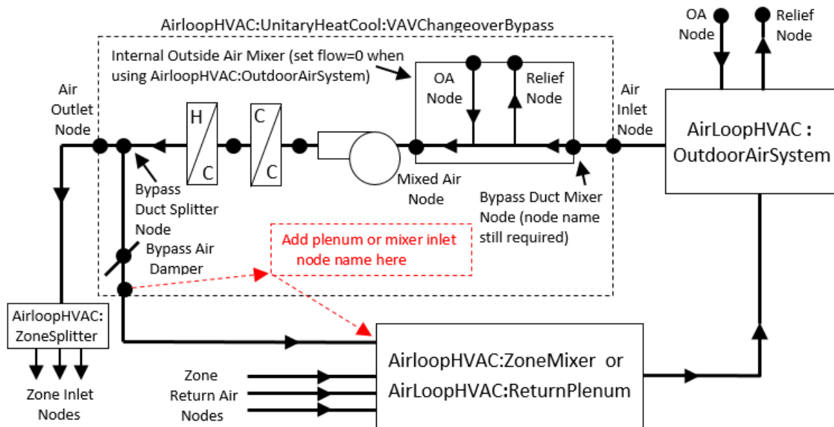
Figure 1.165: Schematic of a CBVAV unitary system used with outdoor air system
