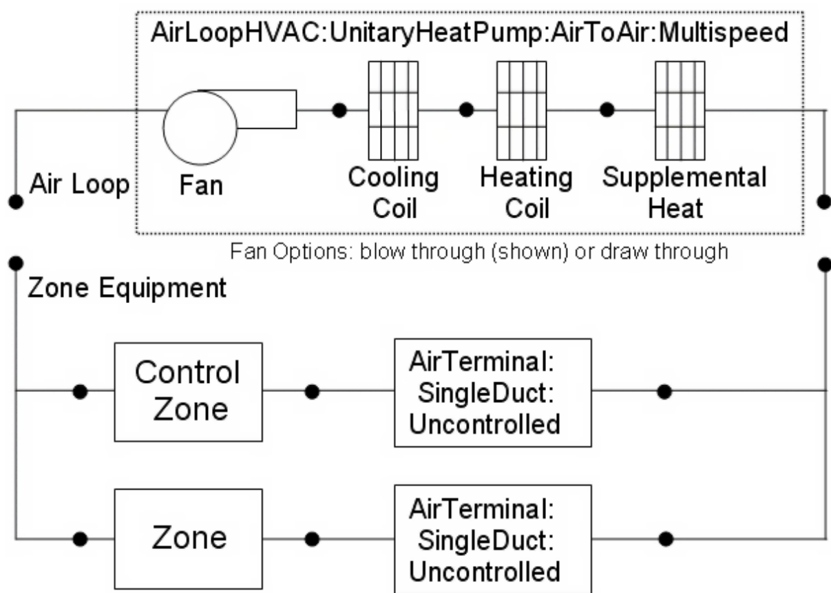
Figure 1.159: Schematic of EnergyPlus Unitary Air-to-Air Multi Speed Heat Pump
