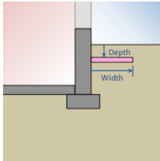
Figure 1.56: Placement of exterior horizontal insulation
