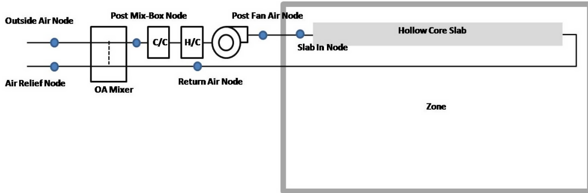
Figure 1.169: Ventilated Slab model - basic system
