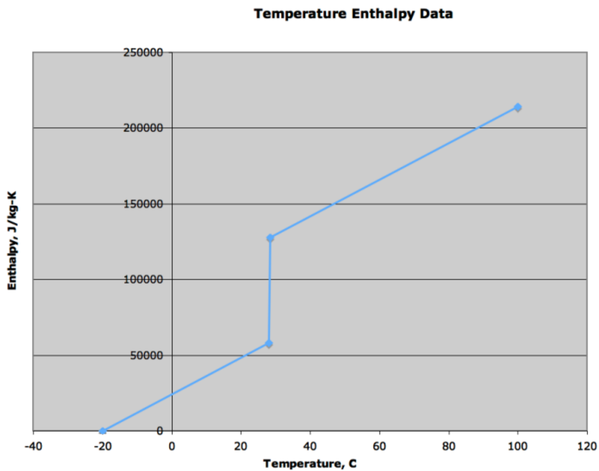
Figure 1.11: Temp-Enth Example
