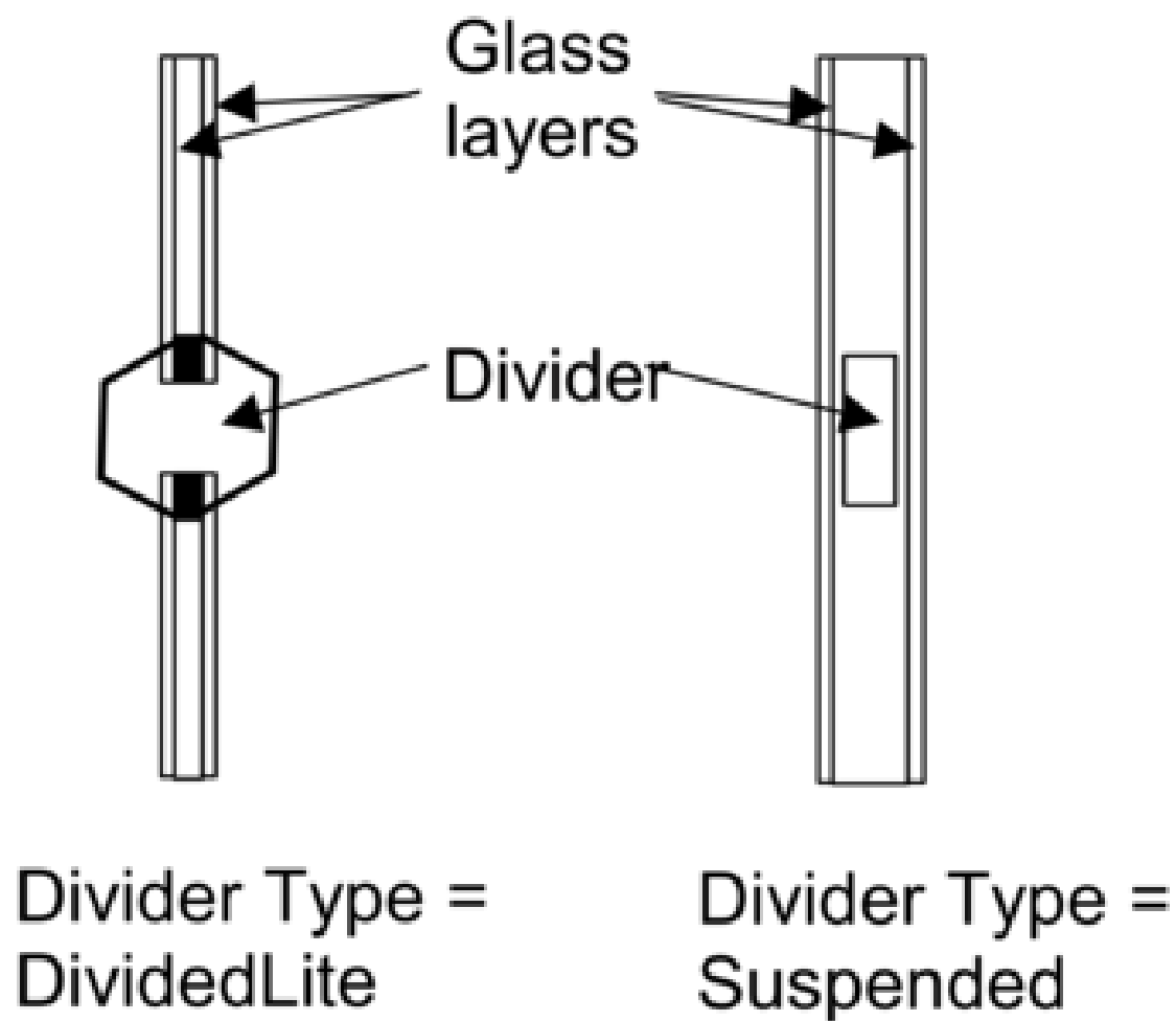
Figure 1.41: Illustration showing divider types.
