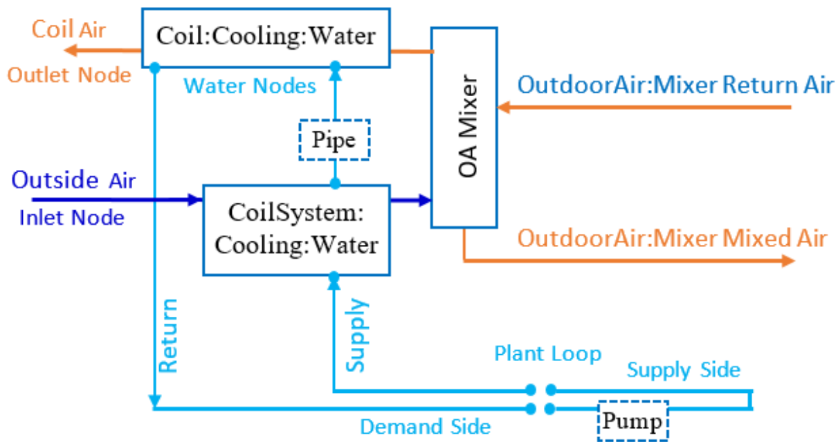
Figure 1.183: Wrap-Around Water Coil Heat Recovery System In Outdoor Air System
