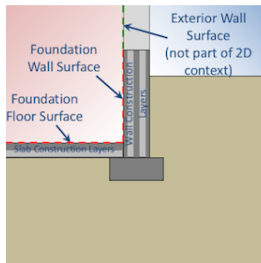
Figure 1.50: Two-dimensional interpretation of foundation surface data
