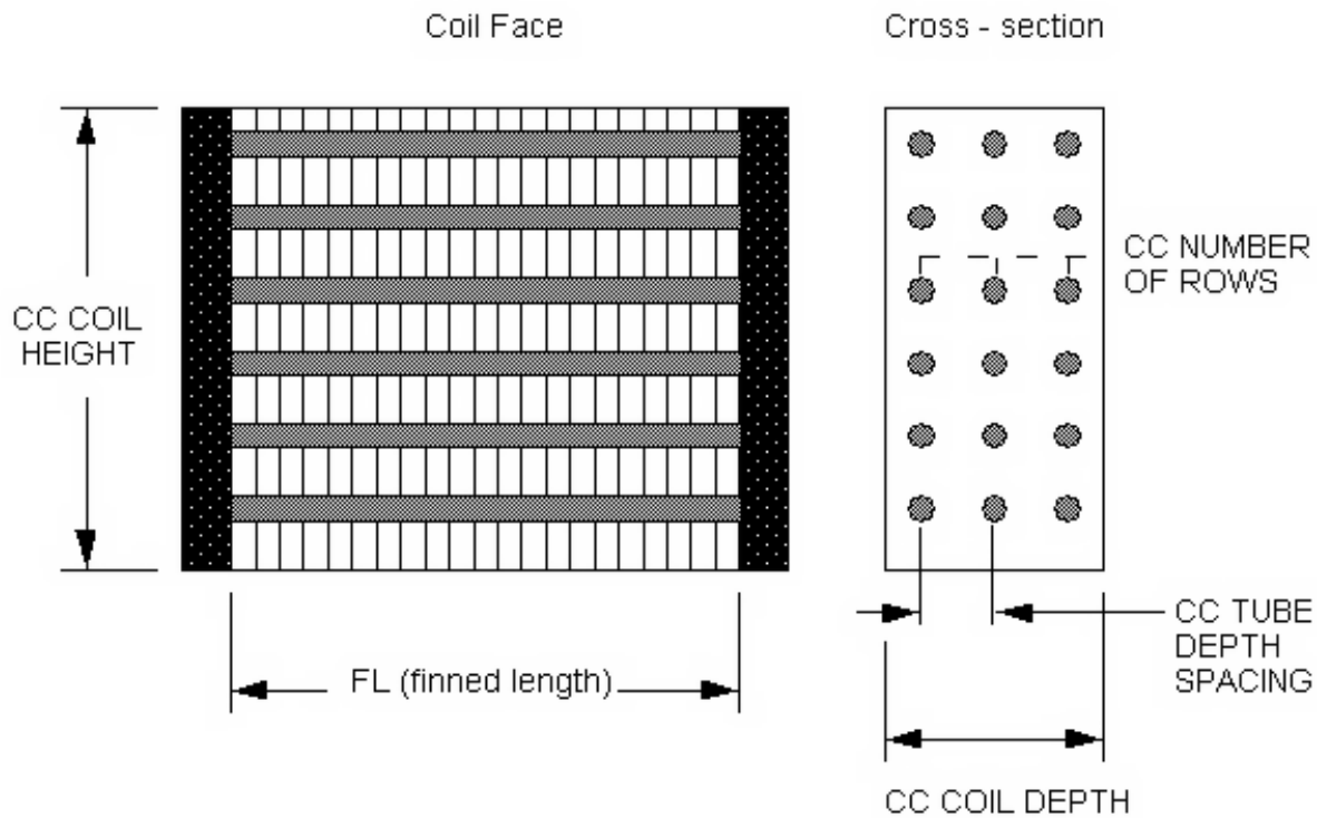
Figure 1.178: Geometry of a Cooling Coil (CC)
