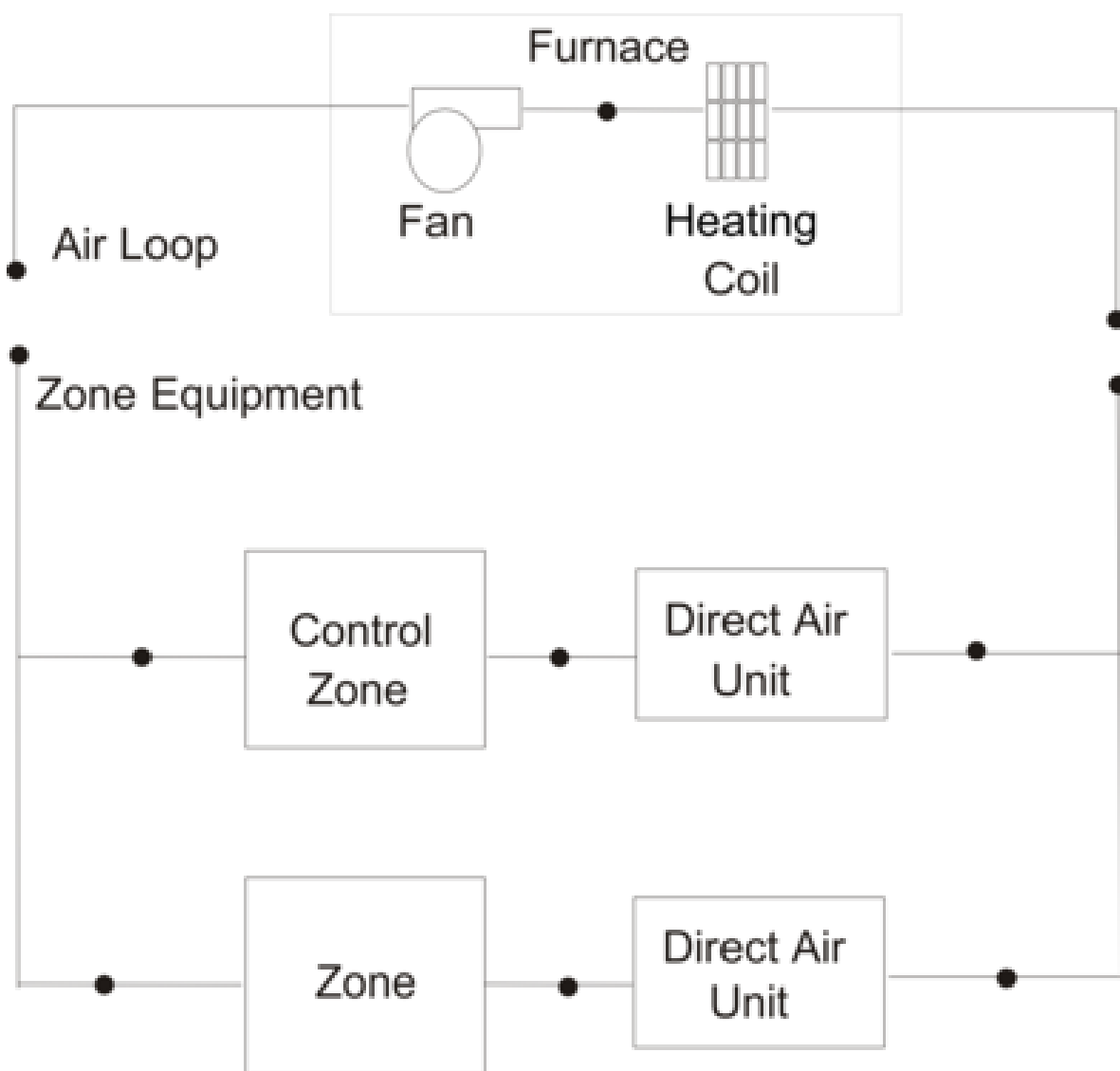
Figure 1.160: Schematic of Blow Through Furnace Model
