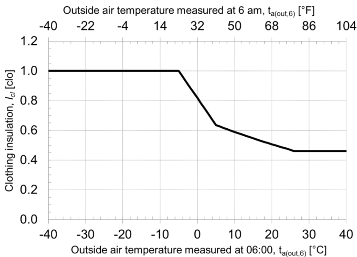
Figure 1.71: Graphical representation of the dynamic predictive clothing insulation model
