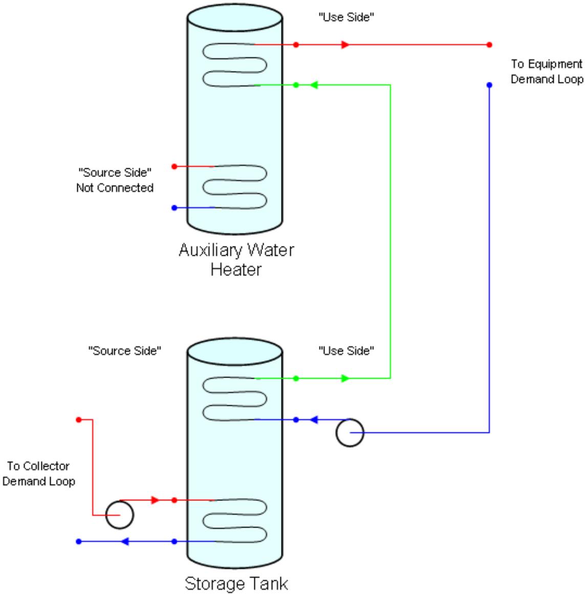
Figure 1.174: Two-Tank Solar Heating System Connection Diagram
