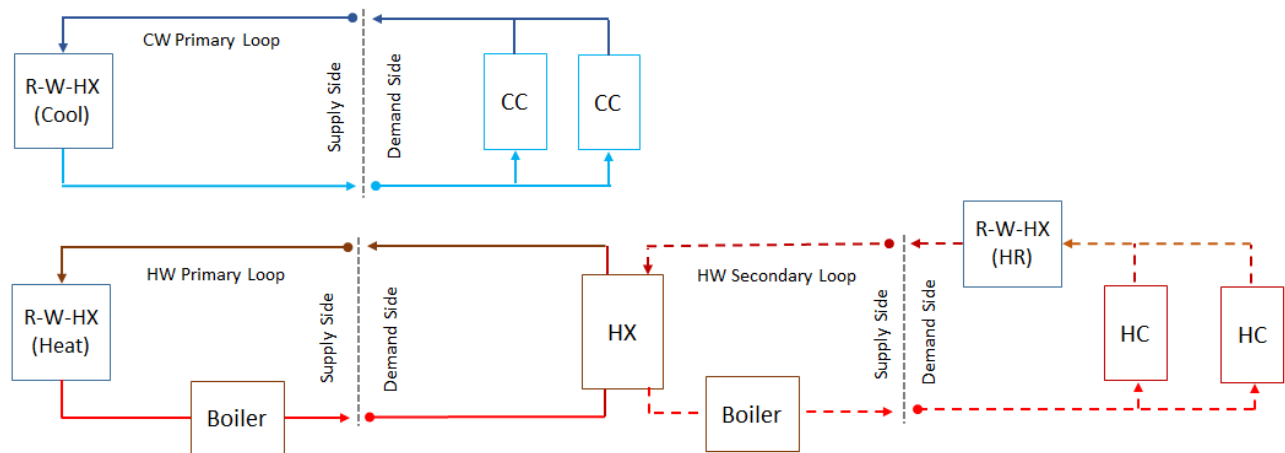
Figure 1.97: Schematic of Six-Pipe Air-to-Water Heat Pump with Heat Recovery
