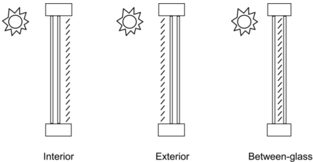
Figure 1.38: Allowed locations of a window shading device.
