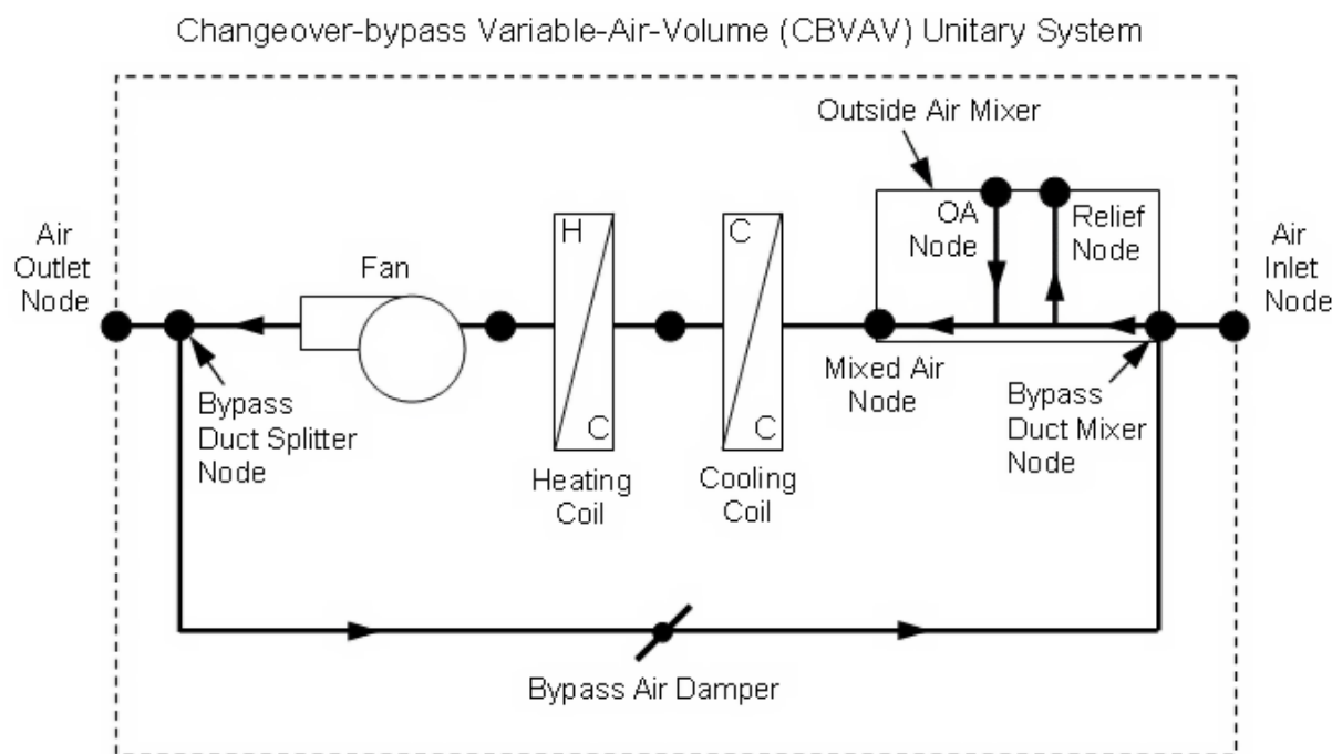
Figure 1.163: Schematic of a CBVAV unitary system (draw through fan placement)
