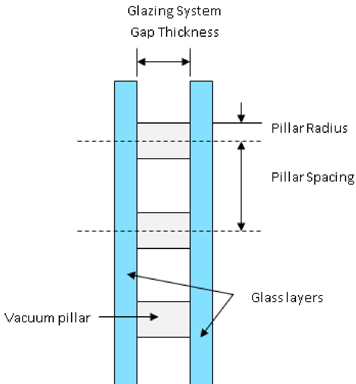
Figure 1.13: Support Pillar
