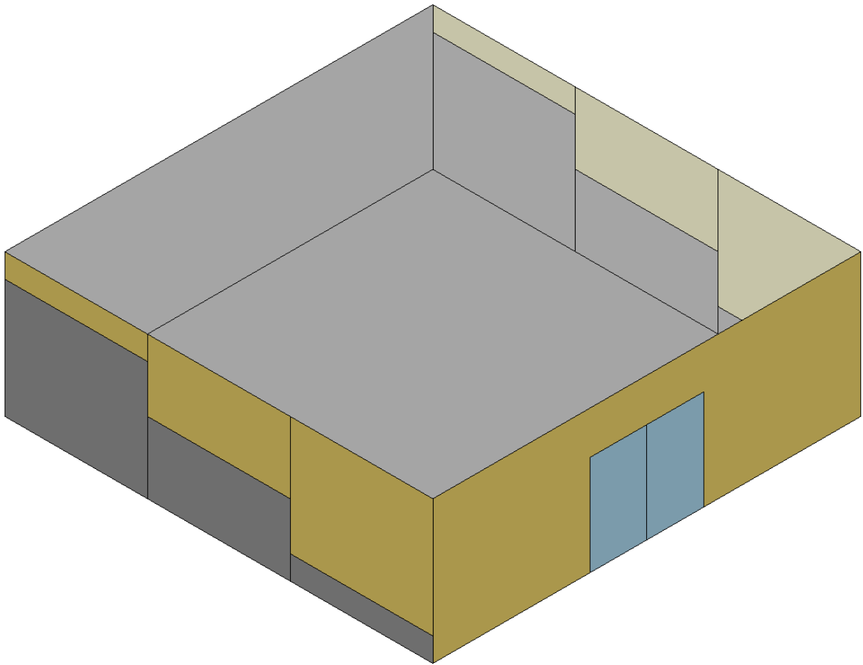
Figure 1.53: Walkout basement wall and floor surfaces (in gray) all reference the same Foundation:Kiva object
