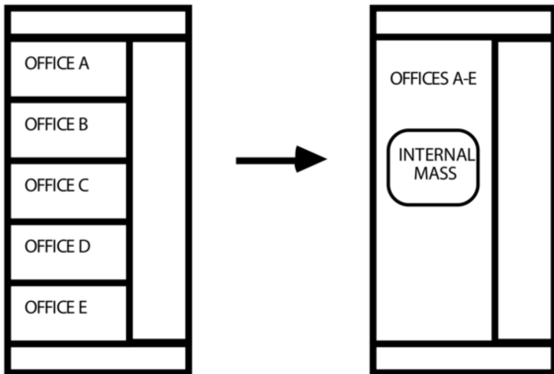
Figure 1.34: Representing 11 internal walls as internal mass
