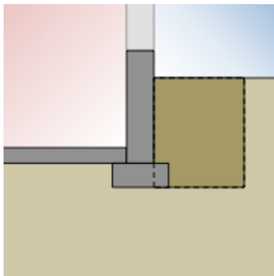
Figure 1.62: Custom block representing exterior backfill
