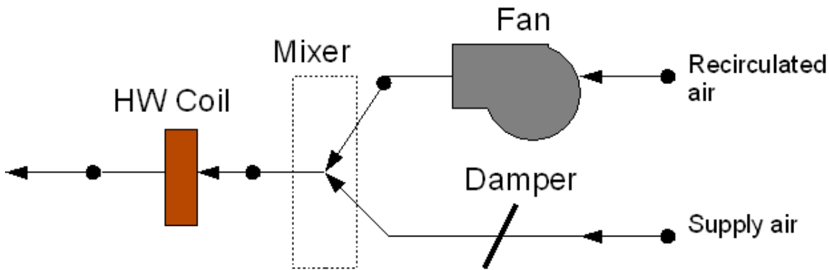
Figure 1.138: Parallel PIU Terminal Unit
