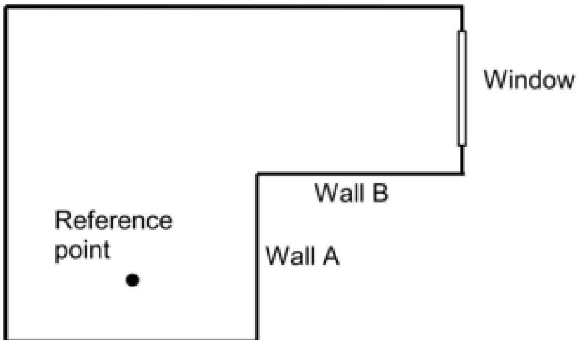
Figure 1.81: Wall A (or Wall B) is an interior obstruction that prevents light from directly reaching the daylighting reference point from the window.
