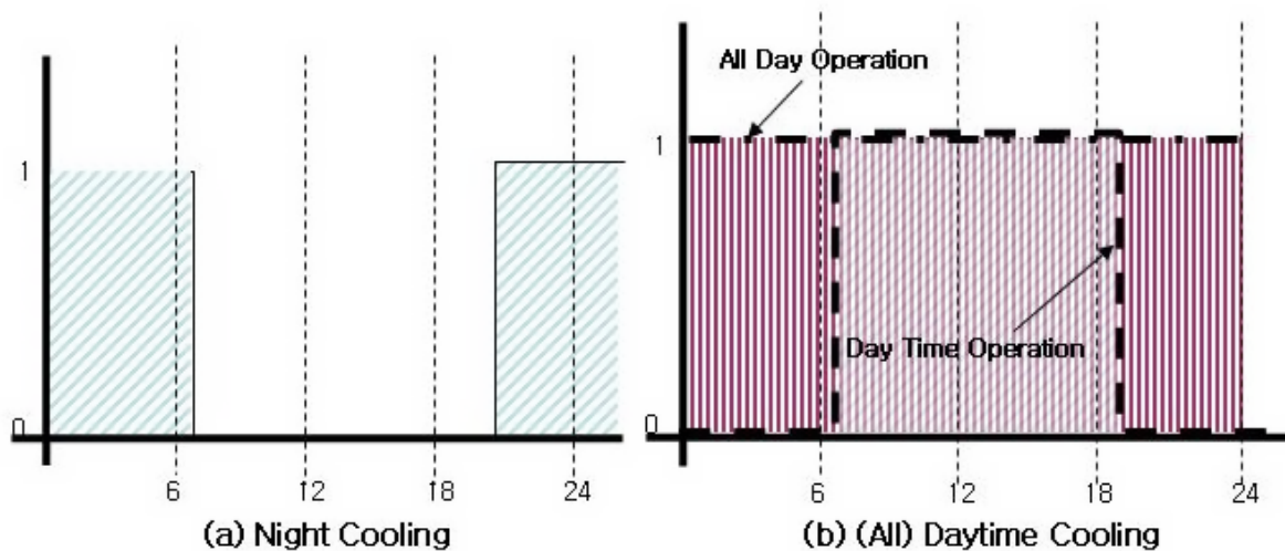
Figure 1.170: Example operating schedule for Ventilated Slab
