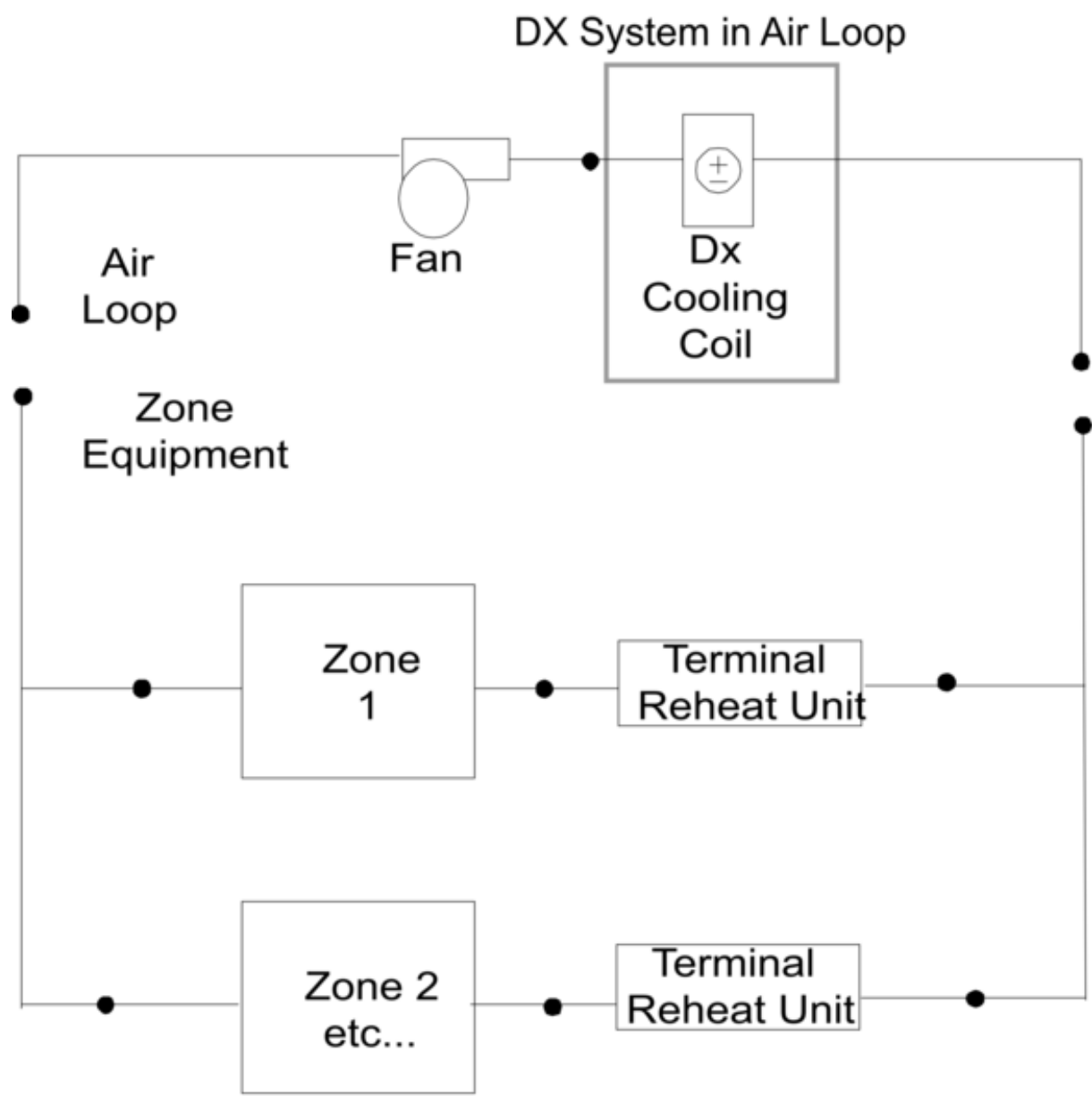
Figure 1.186: Schematic of CoilSystem:Cooling:DX Object in an Air Loop for a Blow Through Application
