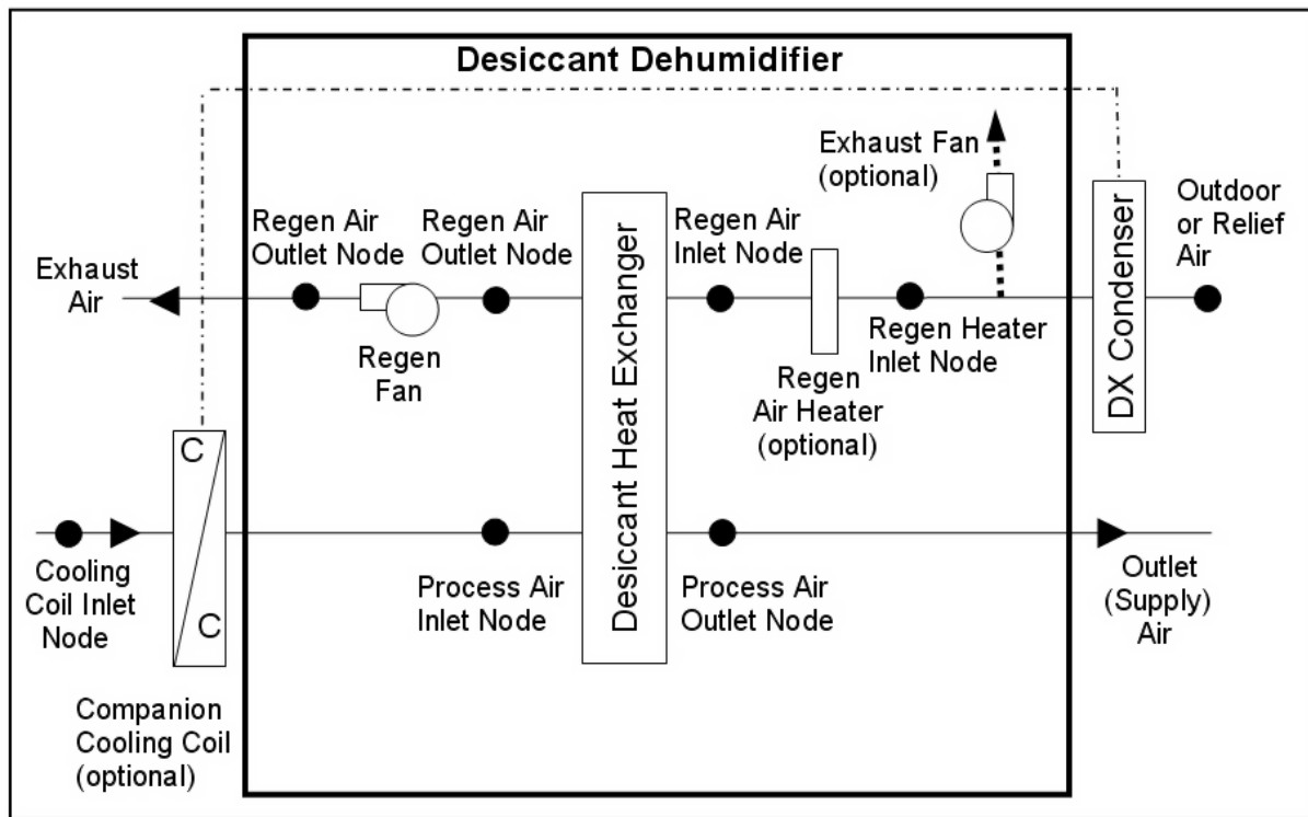
Figure 1.197: Schematic of Dehumidifier:Desiccant:System with Draw Through Regeneration Fan Placement
