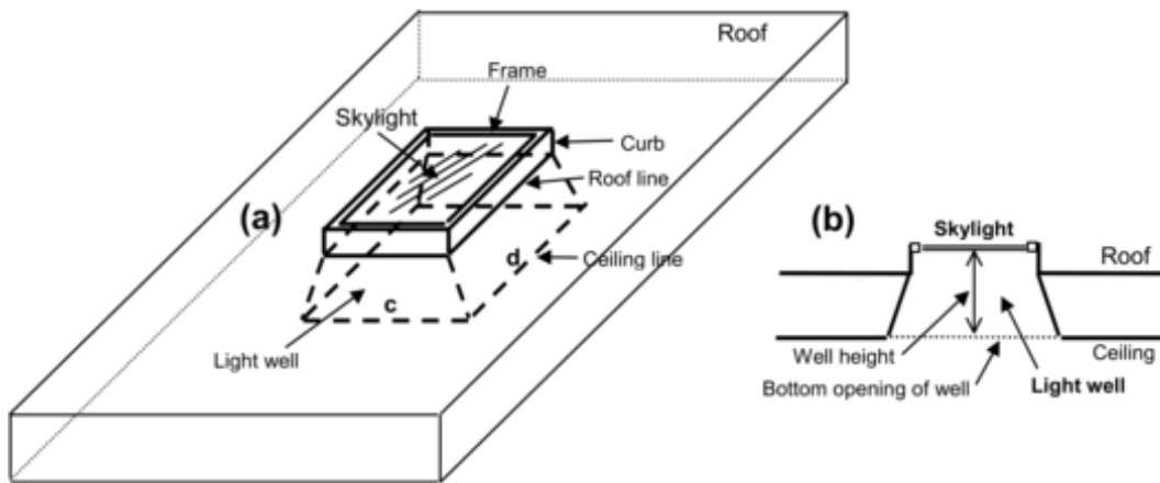
Figure 1.89: Skylight with light well: (a) perspective view, (b) vertical section. If the bottom of the light well is a rectangle of side lengths c and d , as shown in (a), then the perimeter of the bottom of the well = 2(c+d) and the area = cd (see description of field names for the Light Well object).
