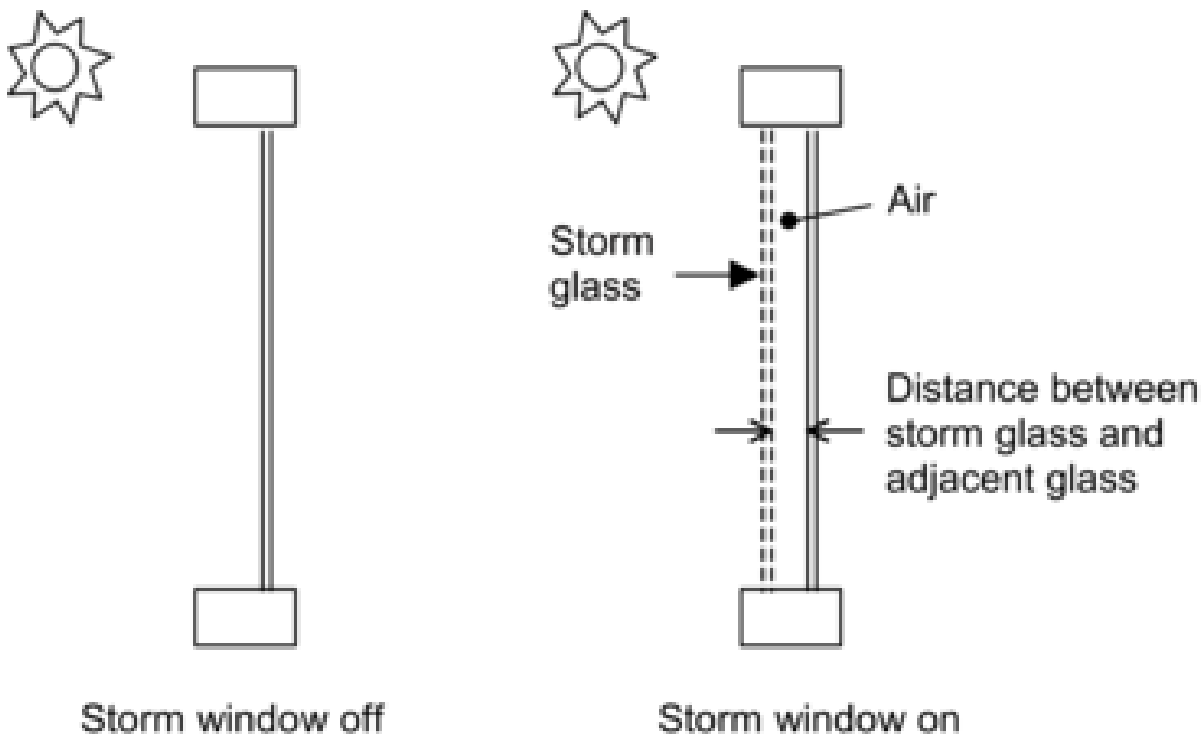
Figure 1.45: Section through a single-glazed window without (left) and with (right) a storm glass layer. Not to scale.
