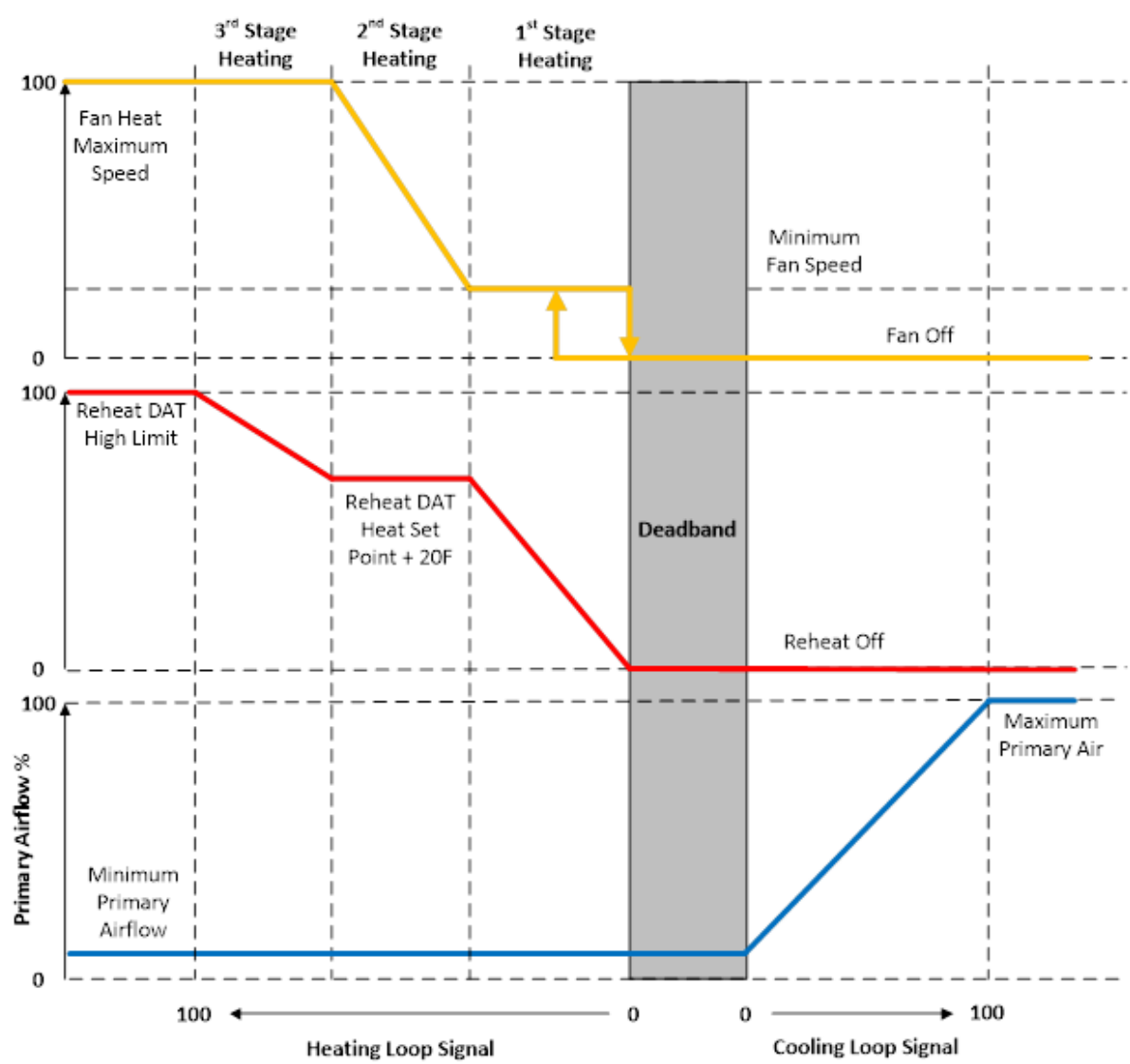
Figure 1.140: Variable Speed Fan with Modulated Heat Control
