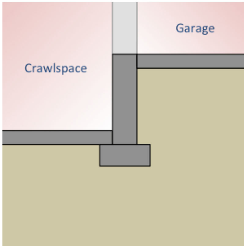
Figure 1.65: Interior foundation wall
