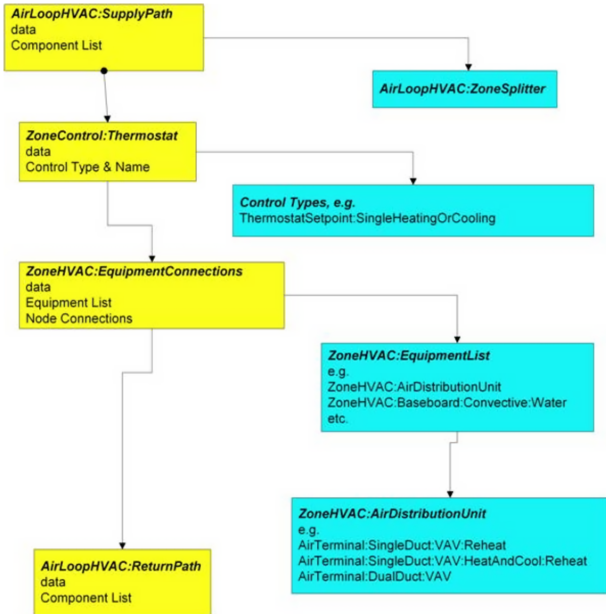
Figure 1.126: Zone Equipment Input Syntax Map
