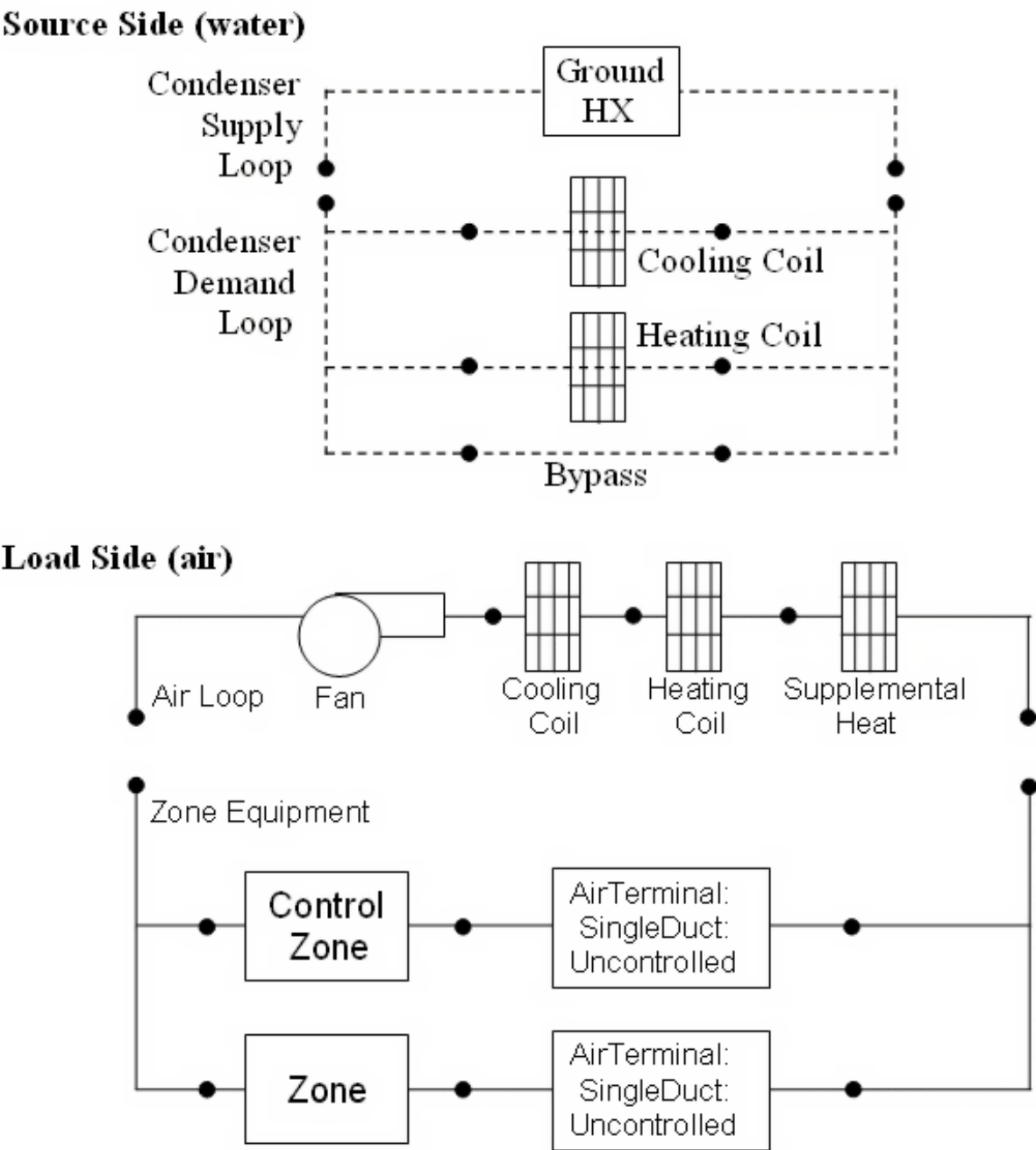
Figure 1.162: Water to Air Heat Pump Schematic for a BlowThrough Configuration with Ground Heat Exchanger
