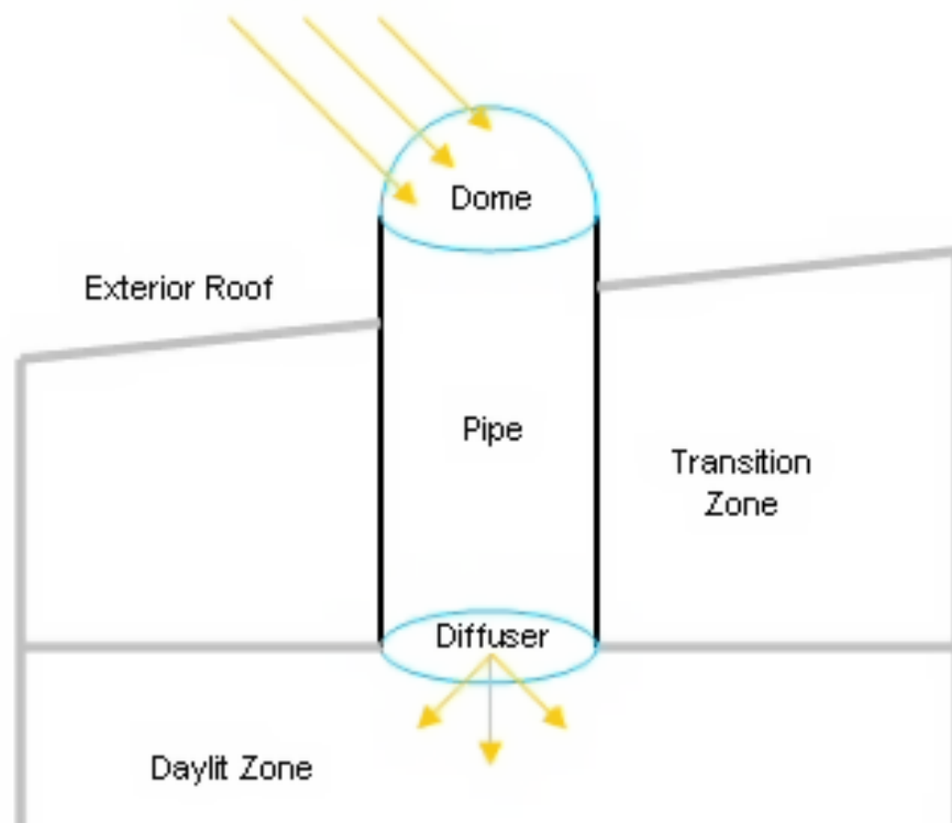
Figure 1.85: Tubular daylighting device diagram.
