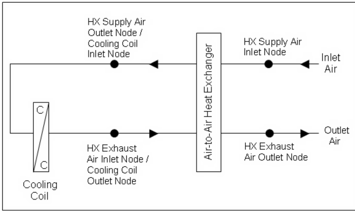
Figure 1.187: Schematic of the CoilSystem:Cooling:DX:HeatExchangerAssisted compound object
