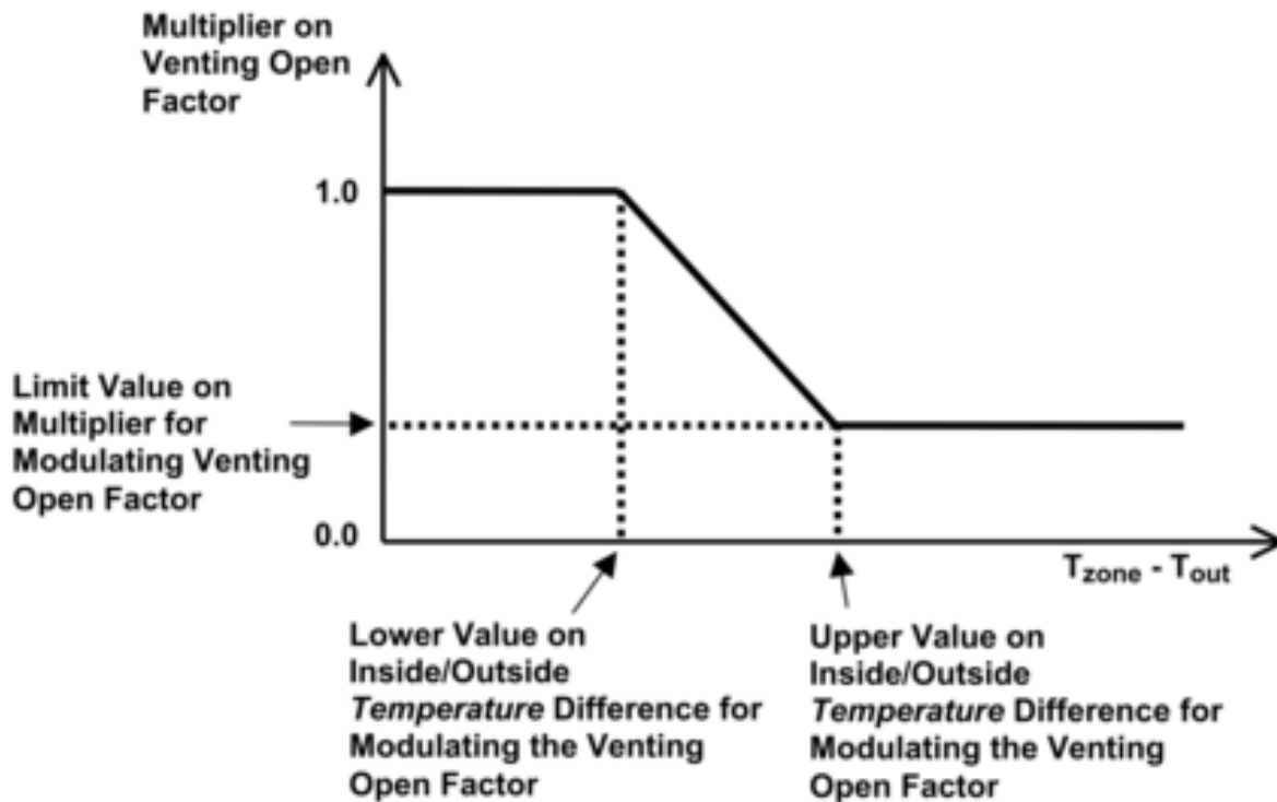
Figure 1.123: Modulation of venting area according to inside-outside temperature difference.
