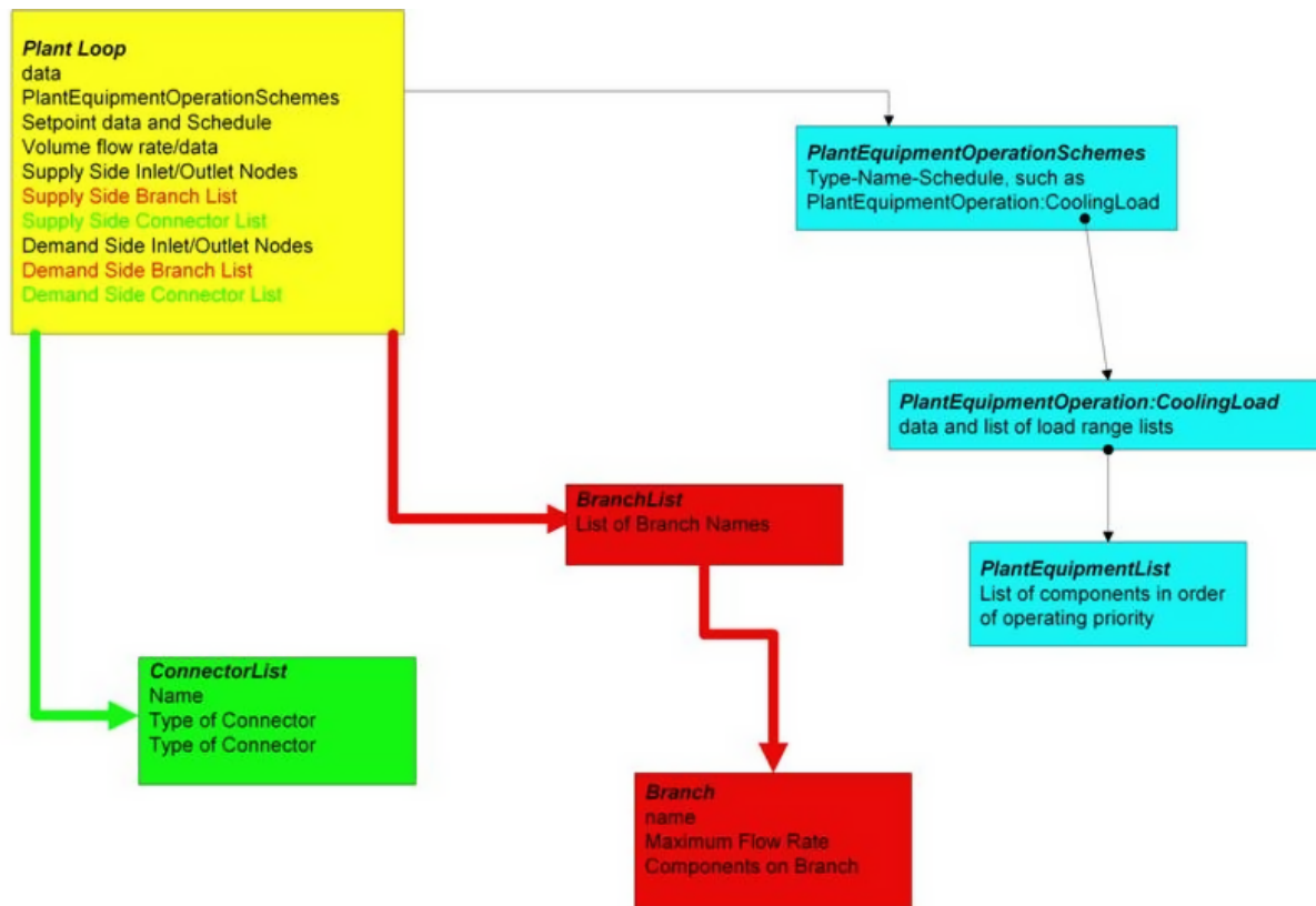
Figure 1.92: Plant Loop Input Syntax Map
