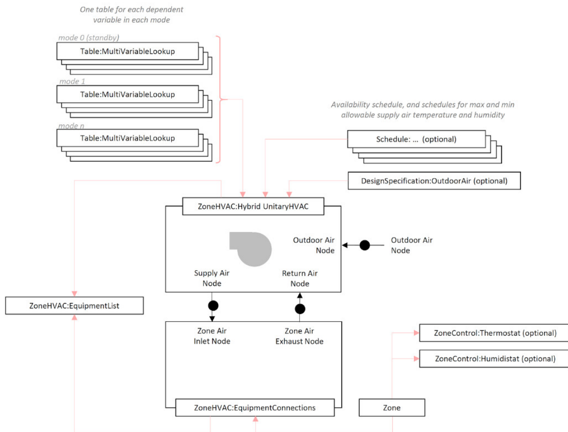
Figure 1.152: Schematic of object links for ZoneHVAC:HybridUnitaryHVAC
