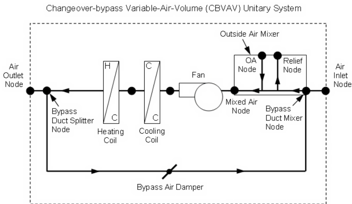
Figure 1.164: Schematic of a CBVAV unitary system (blow through fan placement)
