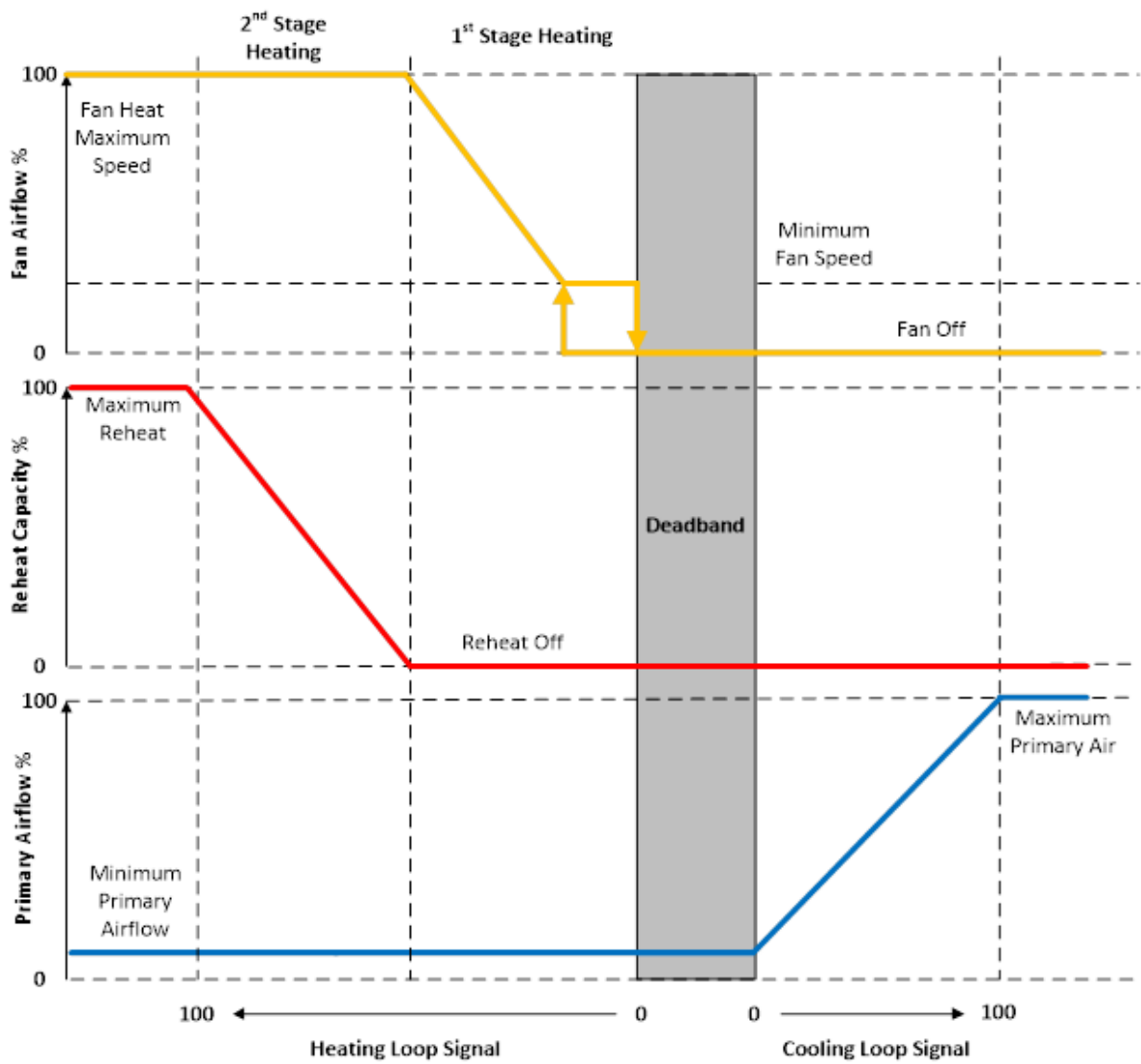
Figure 1.139: Variable Speed Fan with Staged Heat Control
