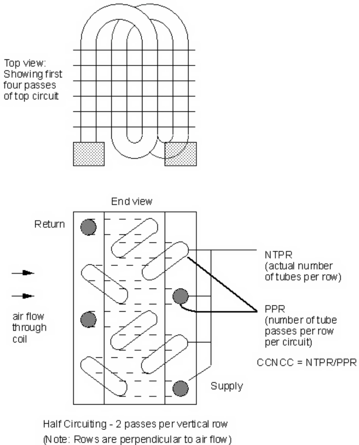
Figure 1.179: Number of Coolant Circuits (CCNCC)
