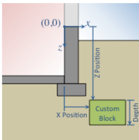
Figure 1.63: Placement of a custom block
