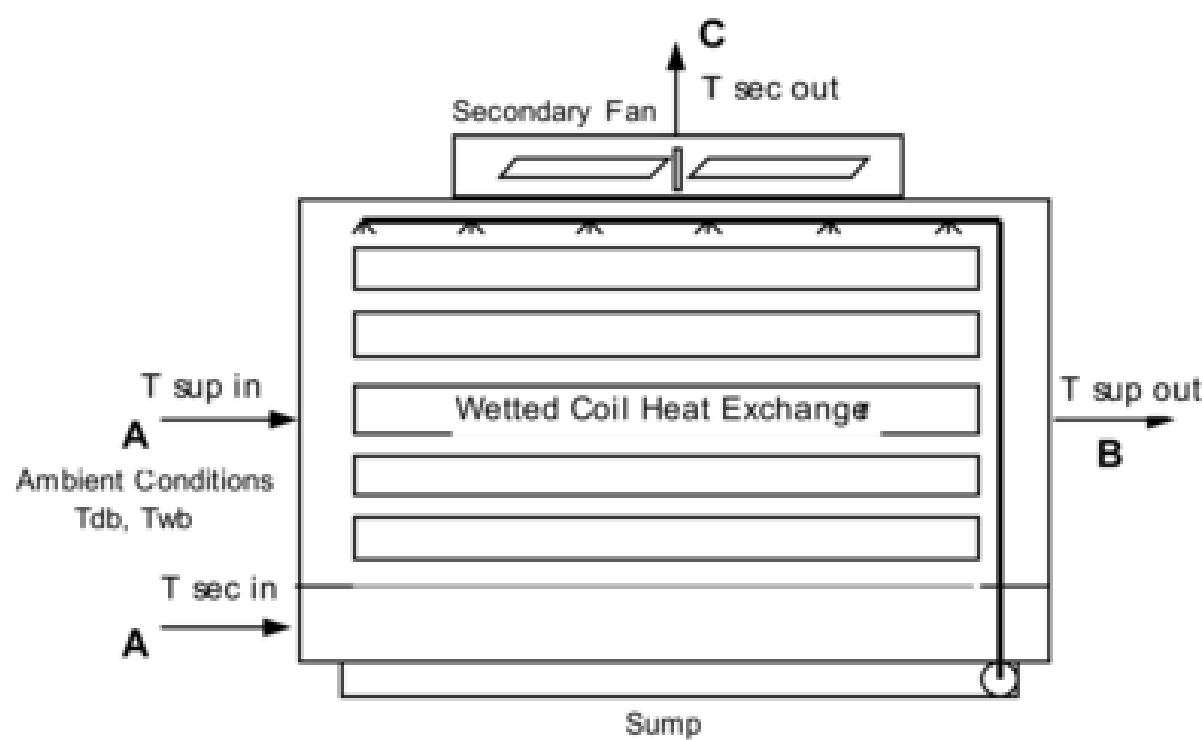
Figure 1.204: Evaporative Cooler Indirect Wet Coil
