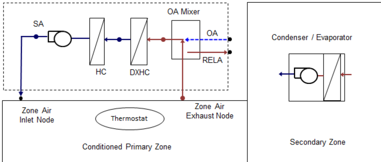
Figure 1.195: Schematic of DX system and secondary coil in cooling mode
