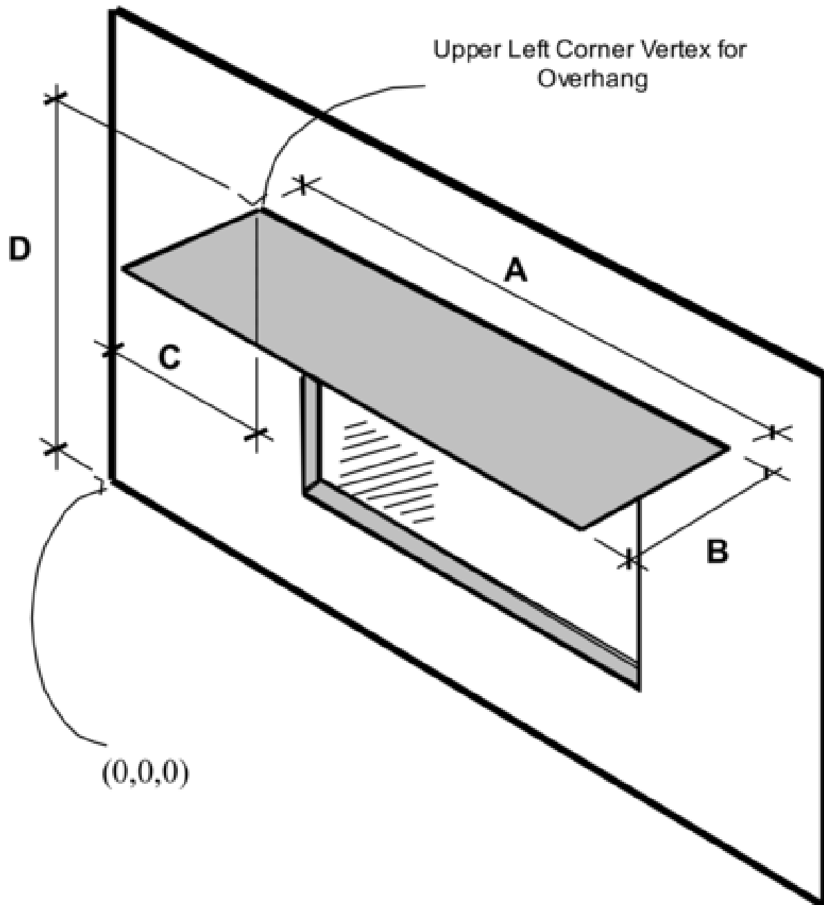
Figure 1.37: Illustration for Attached Shading Surface
