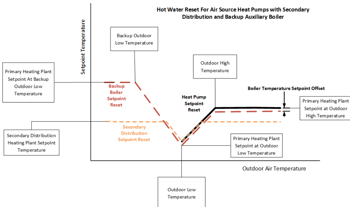
Figure 1.95: Hot Water Temperature Setpoint Vs Outdoor Air Temperature
