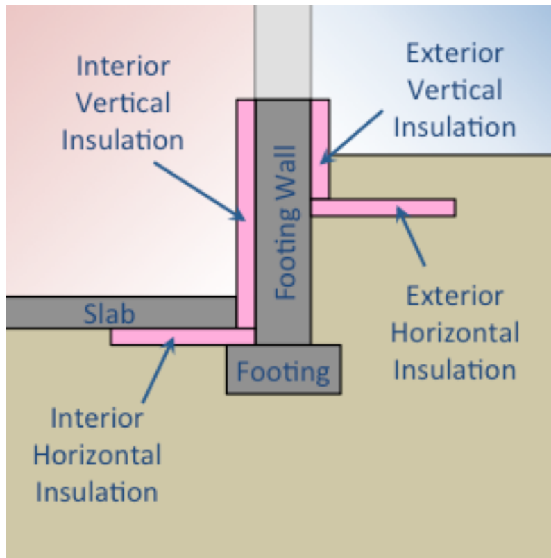
Figure 1.49: Structural and insulation components of Foundation:Kiva objects
