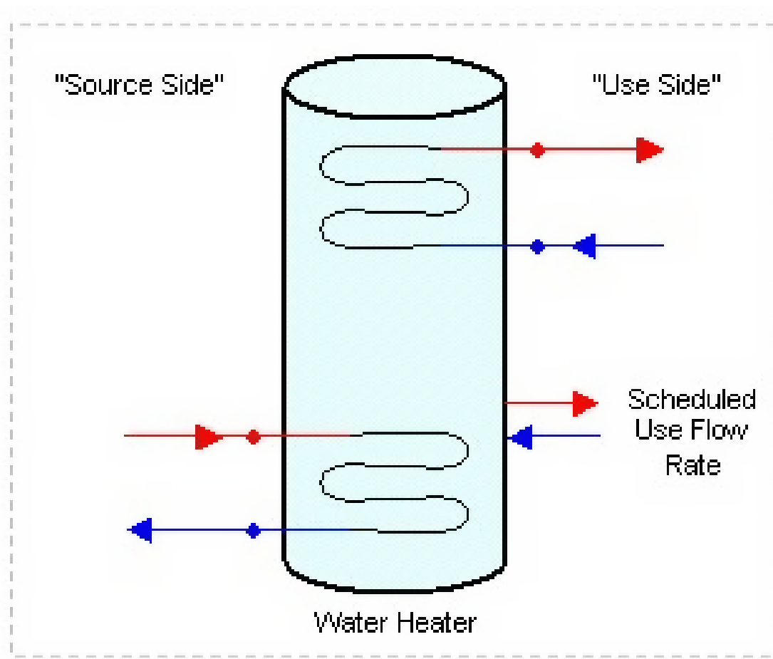
Figure 1.103: Water Heater Configuration
