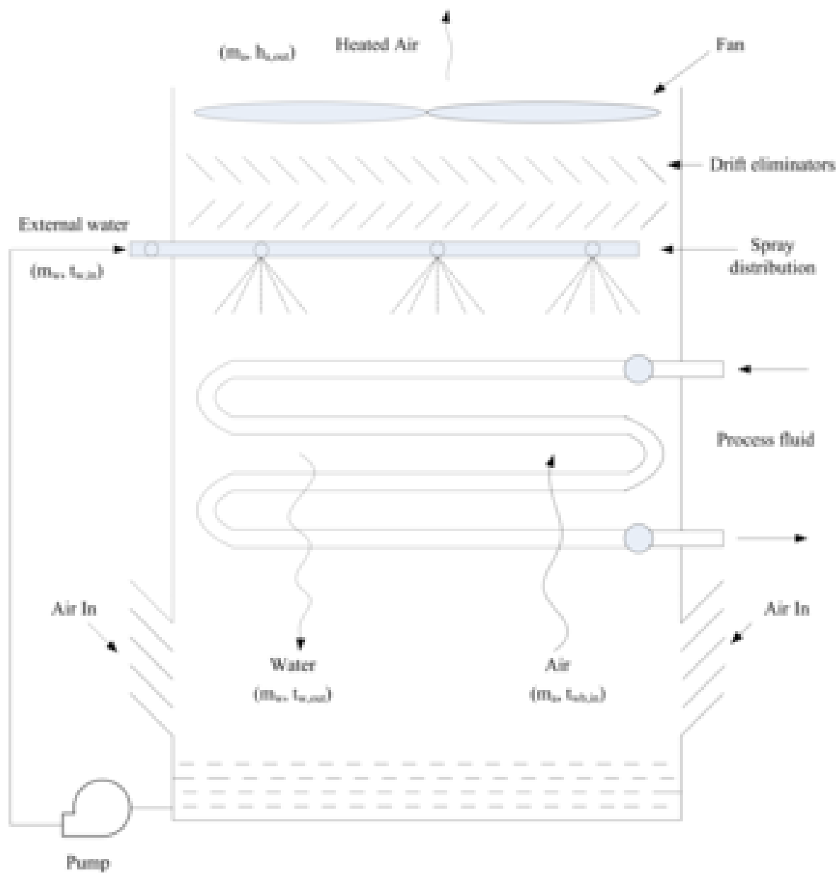
Figure 1.105: Schematic diagram for evaporative fluid cooler
