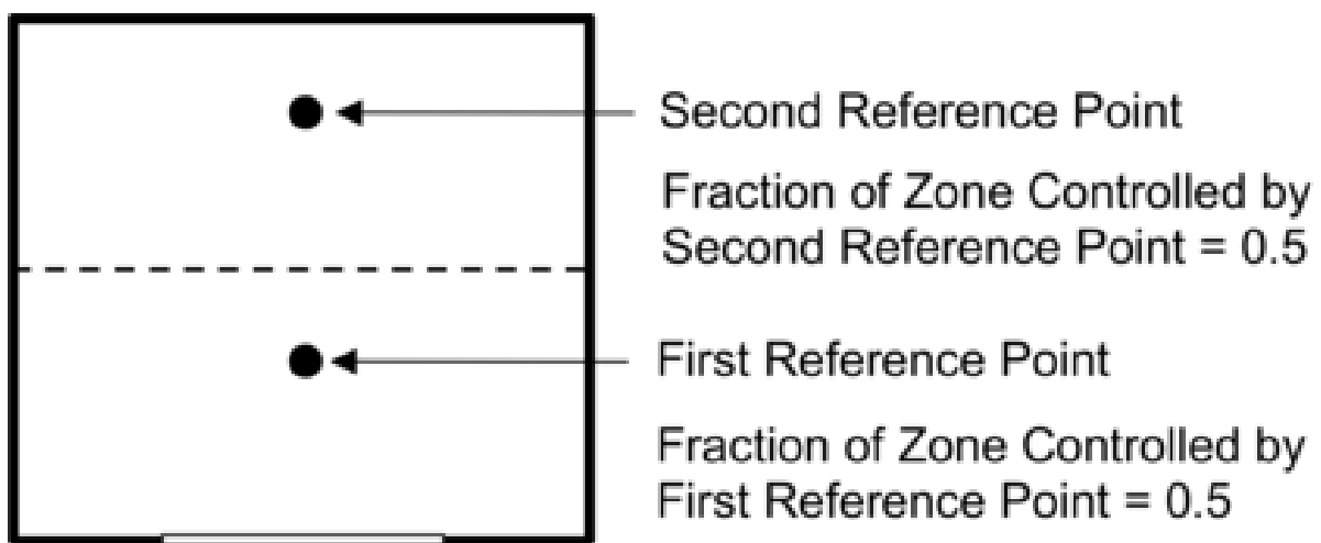
Figure 1.80: Two independently-controlled lighting zones, each with 50% of the area of the thermal zone.
