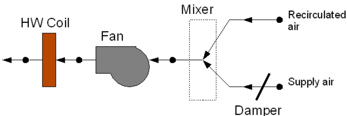
Figure 1.135: Series PIU Terminal Unit
