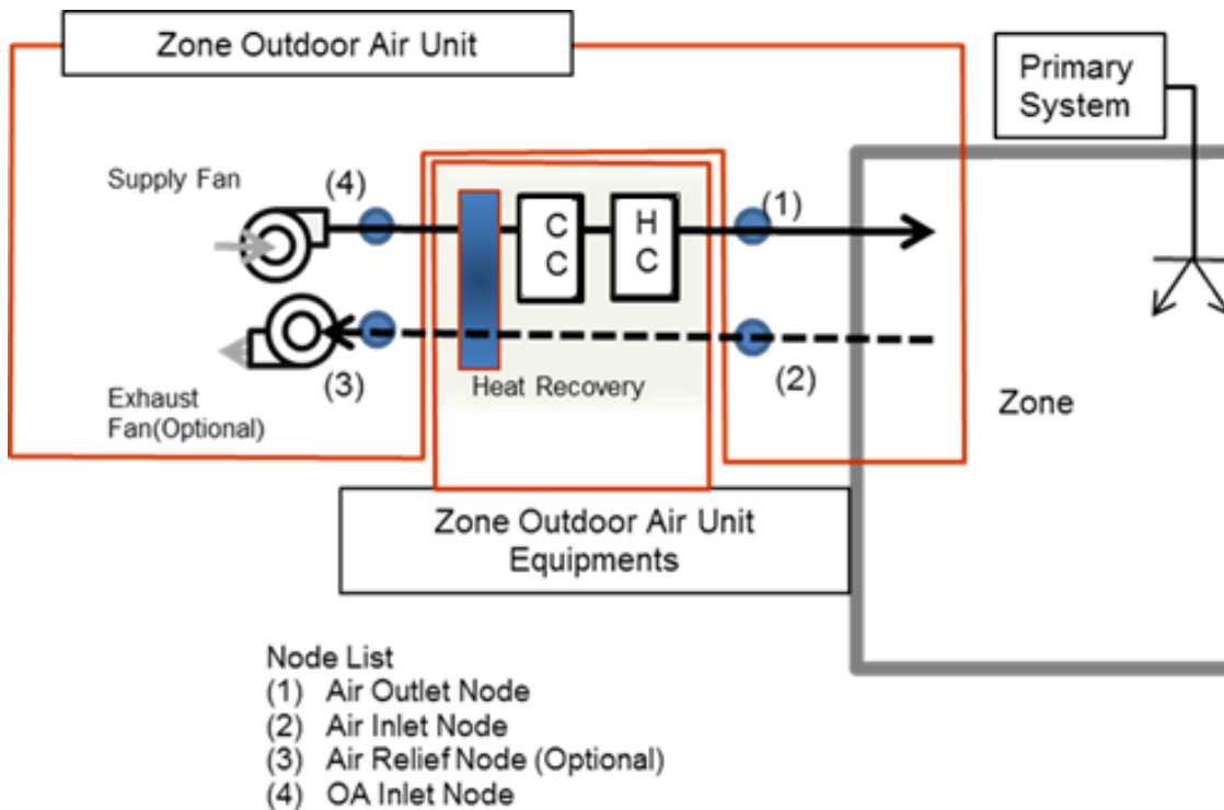
Figure 1.143: Zone Outdoor Air Unit Schematic
