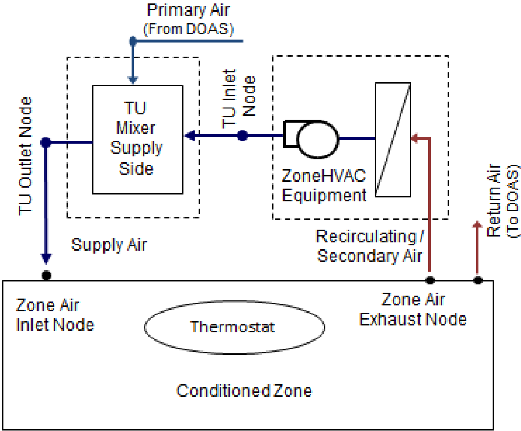
Figure 1.142: Supply Side Mixer Air Terminal Unit with ZoneHVAC equipment
