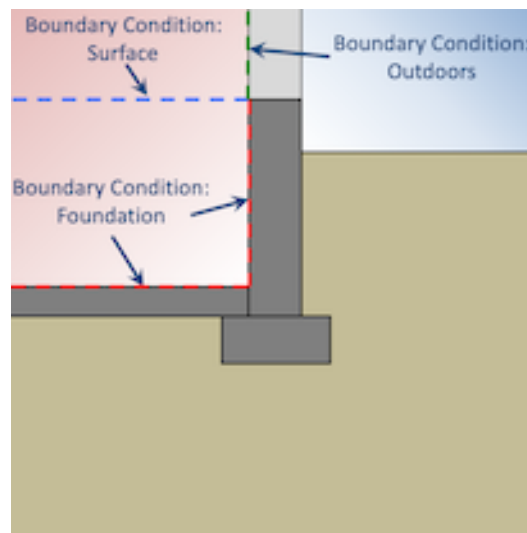
Figure 1.48: Outside Boundary Conditions for surfaces within Kiva’s Two-dimensional context. Only surfaces referencing “Foundation” are simulated in Kiva
