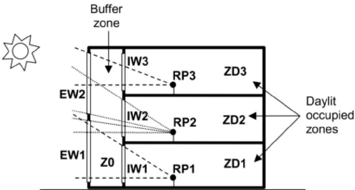
Figure 1.82: Vertical section through a double-façade building showing daylighting through interior windows. The dashed lines show that (1) reference point RP1 receives direct light from exterior window EW1 via interior window IW1; (2) RP2 receives direct light from EW1 and EW2 via IW2; and (3) RP3 receives direct light from EW2 via IW3.
