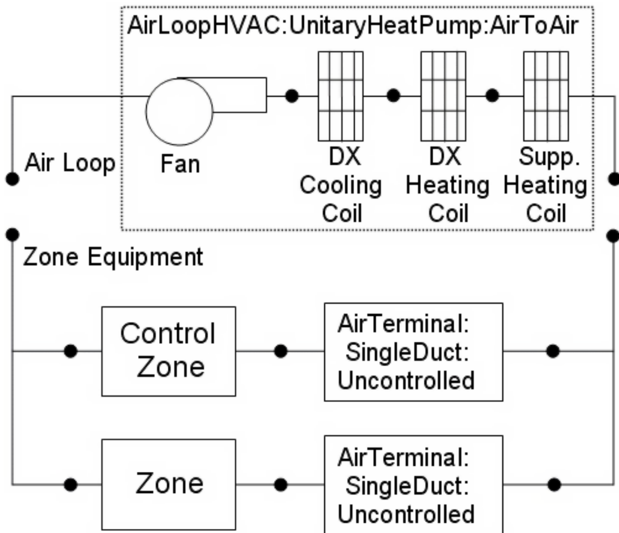
Figure 1.158: Schematic of EnergyPlus Unitary Air-to-Air Heat Pump (Blow Through Configuration)
