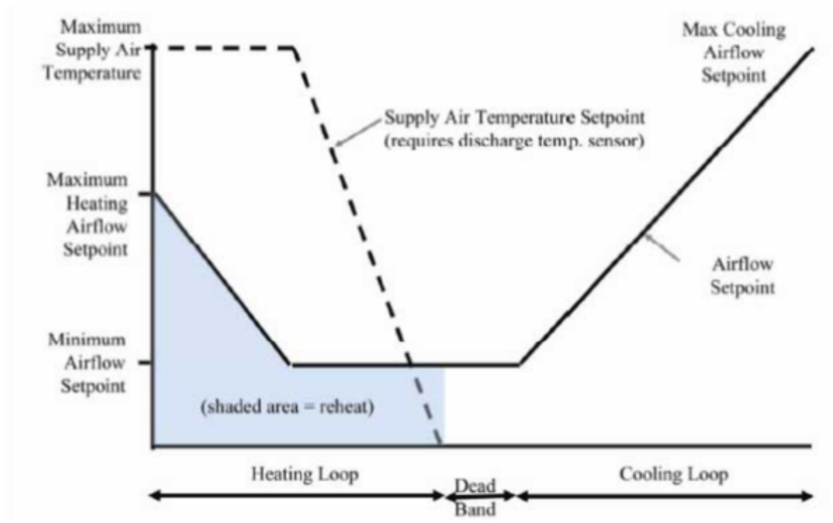
Figure 1.132: The Dual Maximum Control Logic
