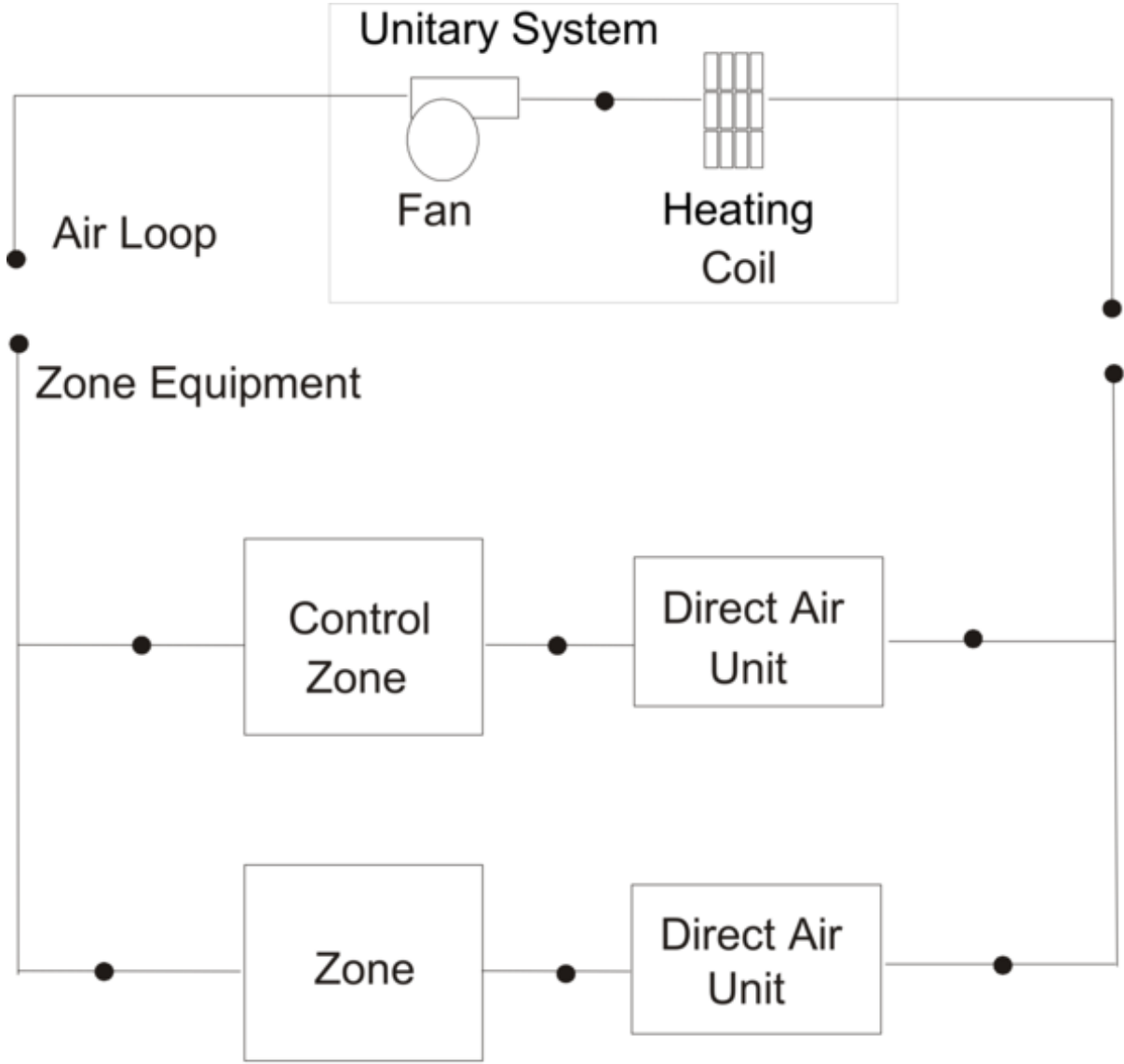
Figure 1.161: Schematic of Blow Through Heat-Only Unitary System
