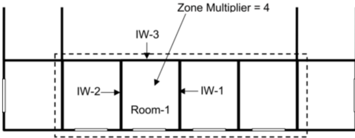
Figure 1.78: For daylighting purposes the thermal zone enclosed by the dashed boundary line should be modeled as a typical zone (Room-1) with a zone multiplier of 4.
