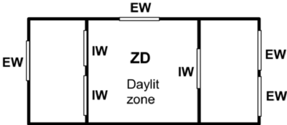
Figure 1.83: General configuration of daylighting through interior windows that can be calculated with EnergyPlus. IW = interior window, EW = exterior window.
