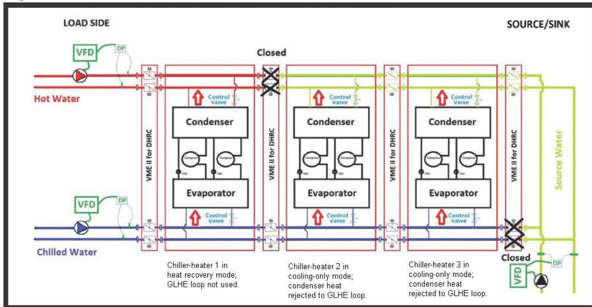
Figure 1.101: Diagram of a central heat pump system with one chiller-heater in heat recovery mode and two chiller-heaters in cooling-only mode
