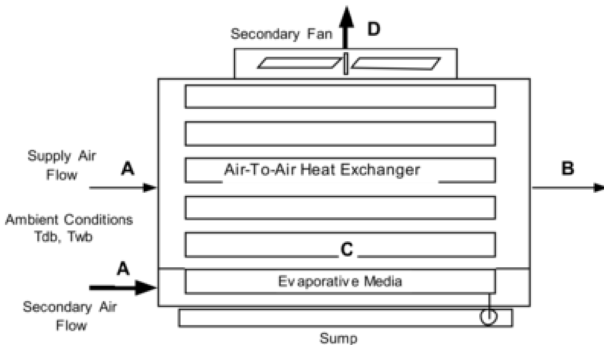
Figure 1.202: Evaporative Cooler – Indirect Dry Coil
