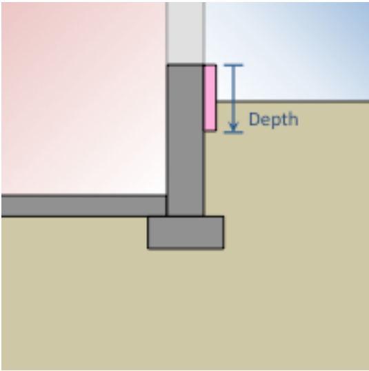
Figure 1.57: Placement of exterior vertical insulation
