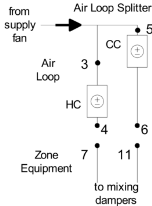
Figure 1.128: Air Loop/Zone Equipment Node Diagram
