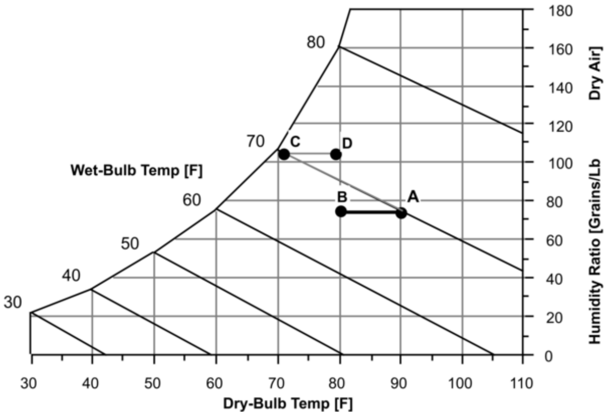
Figure 1.203: Secondary Air Process – Indirect Dry Coil Evap Cooler
