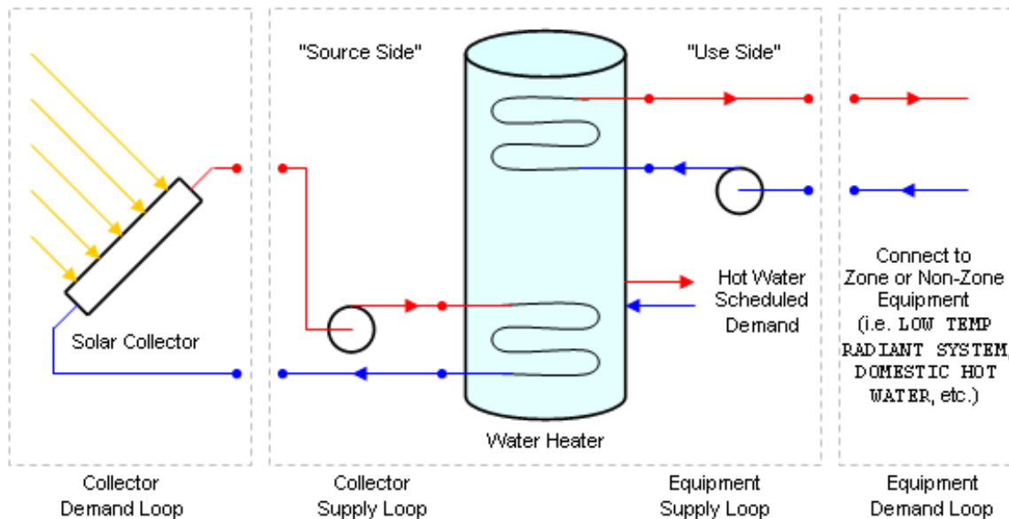
Figure 1.173: Solar Collector Plant Loop Connection Diagram
