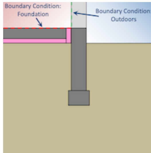
Figure 1.51: Two-dimensional interpretation of foundation surface data
