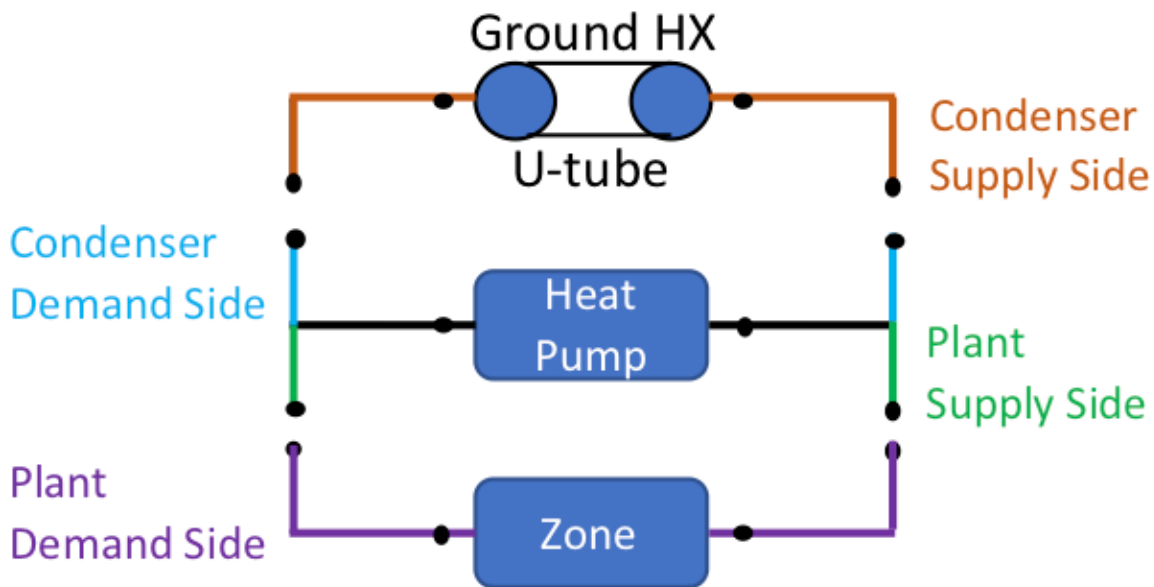
Figure 1.98: Schematic of EnergyPlus Ground Loop Heat Exchanger
