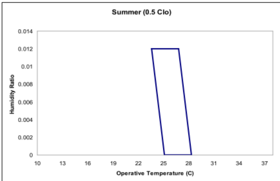
Figure 1.73: Summer Comfort Range
