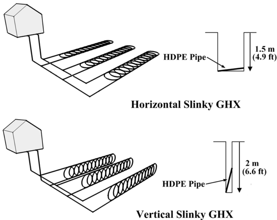
Figure 1.107: Slinky Ground Heat Exchanger Configurations
