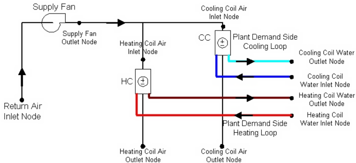
Figure 1.177: Example Air Loop Heating &amp; Cooling Coil
