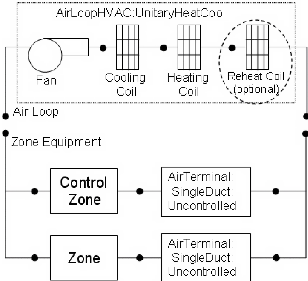
Figure 1.157: Schematic of Blow Through Heat/Cool Unitary System
