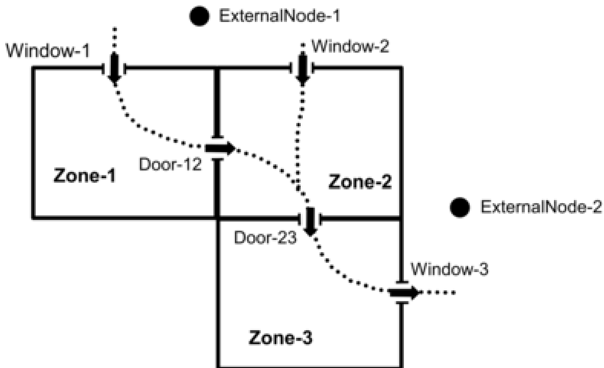
Figure 1.120: Plan view of a simple air flow network showing a possible air flow pattern in which all of the windows and doors are open.
