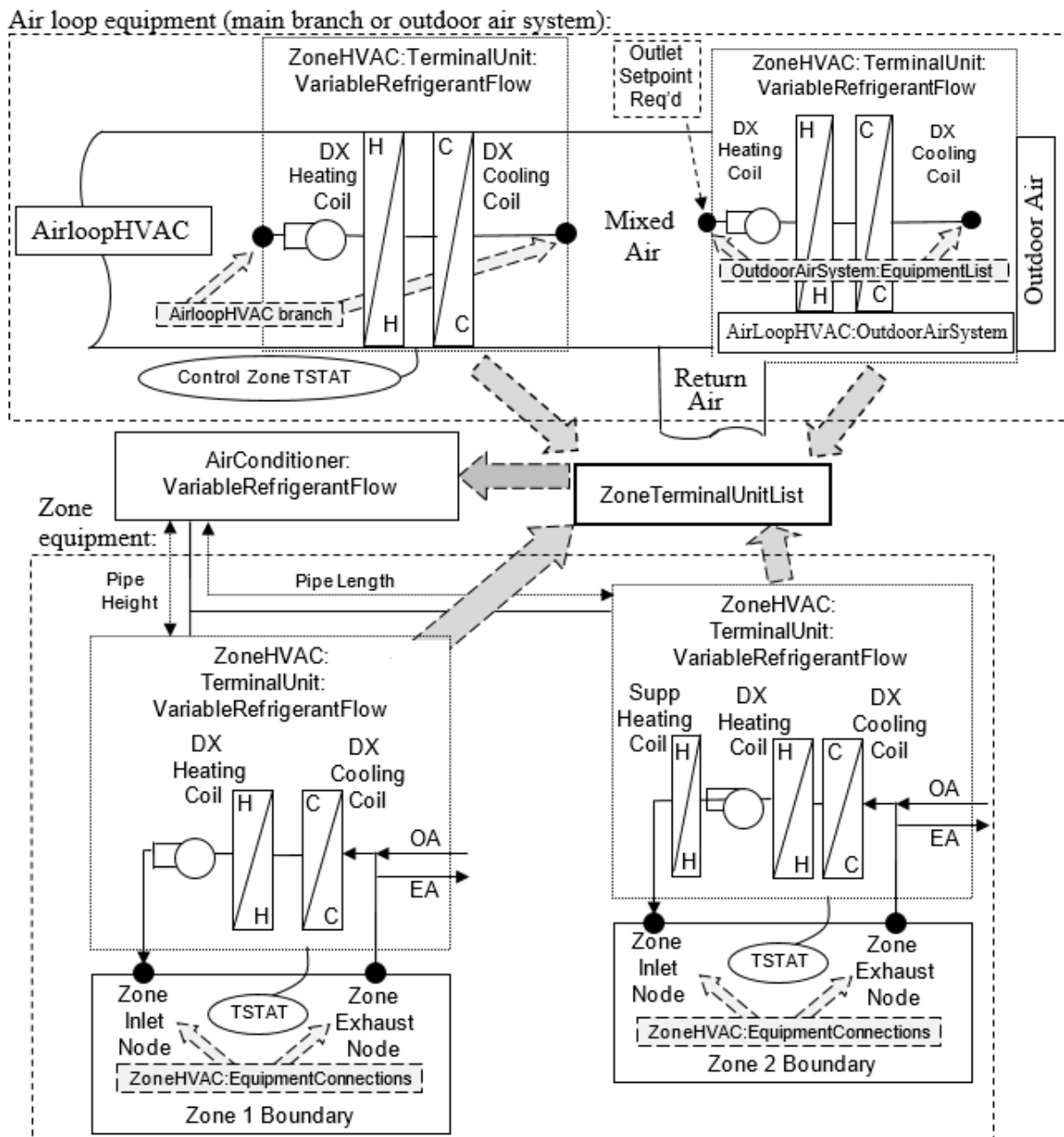
Figure 1.166: Variable Refrigerant Flow Schematic
