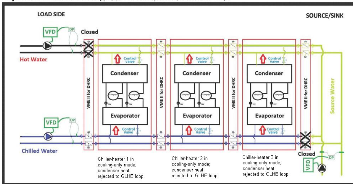
Figure 1.99: Diagram of a central heat pump system with three chiller-heaters in cooling-only mode (Condensers reject heat to the ground source loop)
