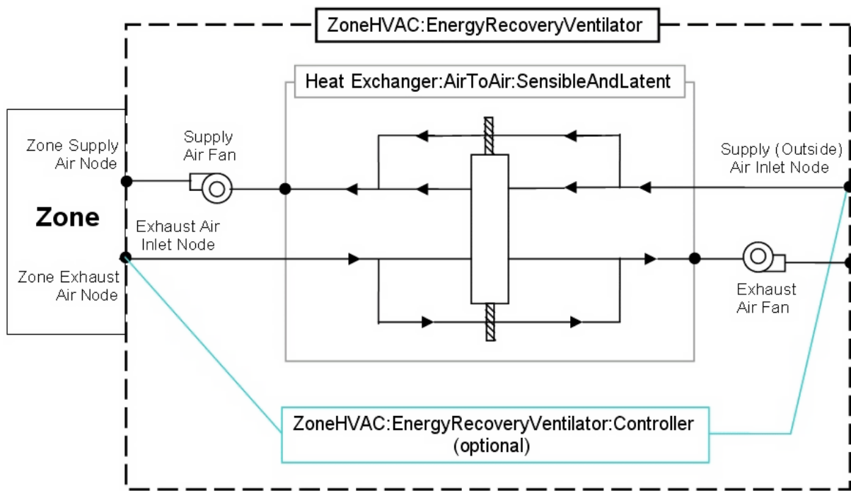
Figure 1.151: ZoneHVAC:EnergyRecoveryVentilator compound object Schematic
