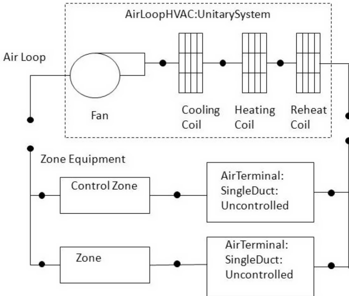
Figure 1.155: Schematic of the EnergyPlus Unitary System
