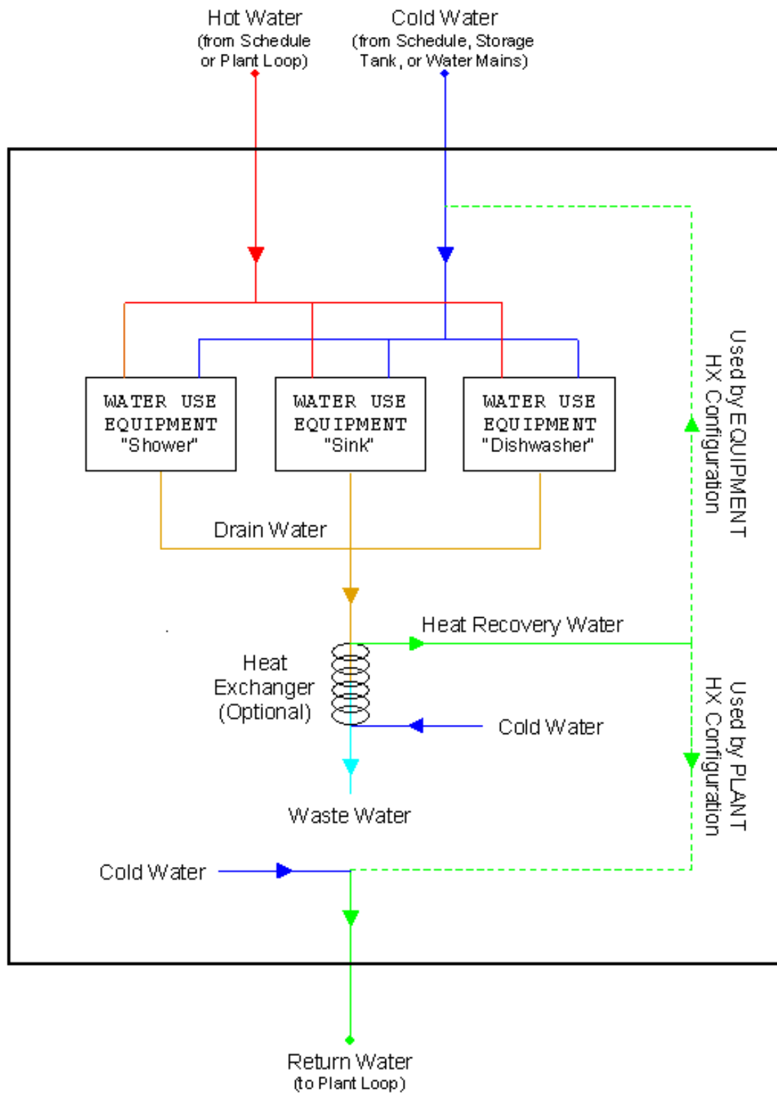
Figure 1.215: Diagram of internal connections for WaterUse:Connections
