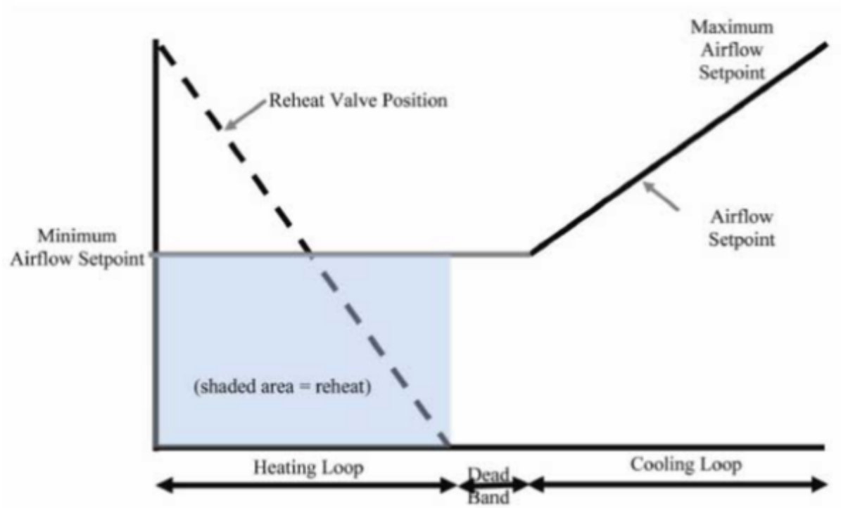
Figure 1.131: The Single Maximum Control Logic
