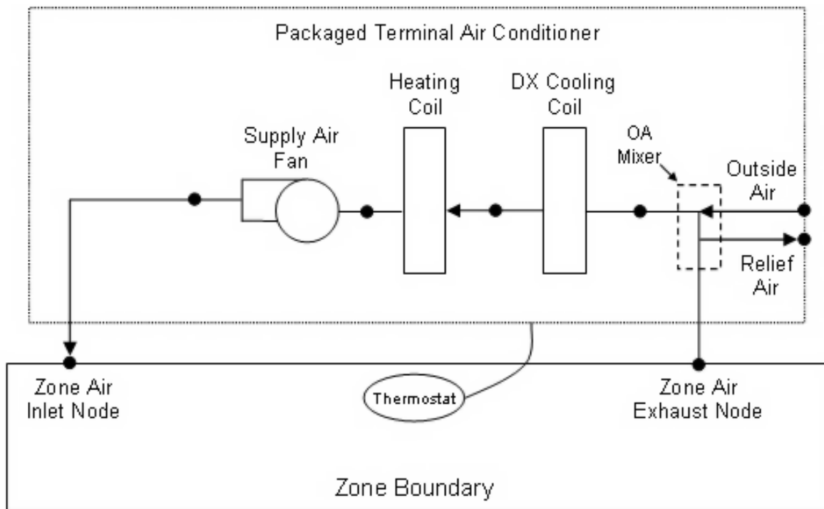
Figure 1.144: Schematic of a packaged terminal air conditioner with draw through fan placement
