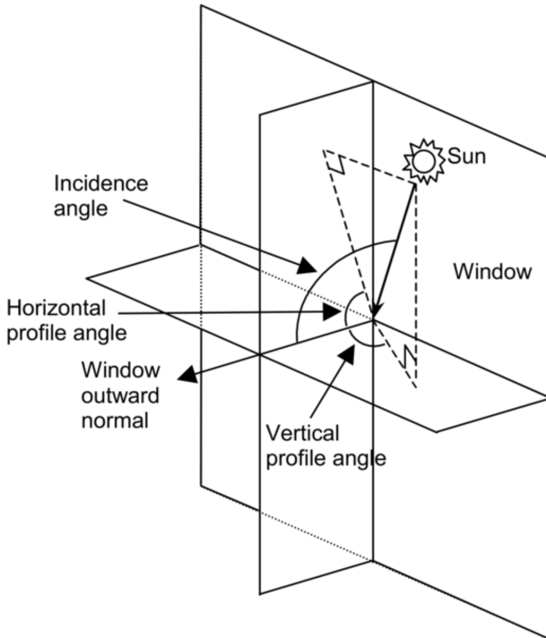
Figure 1.36: Vertical exterior window showing solar horizontal profile angle, solar vertical profile angle and solar incidence angle.
