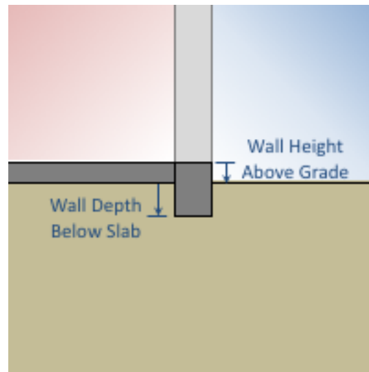
Figure 1.59: Definition of exterior grade and footing wall depth relative to the wall surface (for a slab foundation context)
