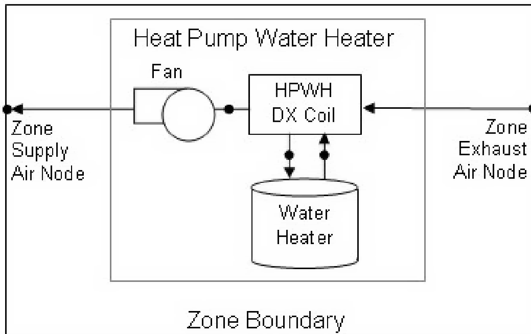
Figure 1.104: Schematic diagram for a heat pump water heater located in a zone
