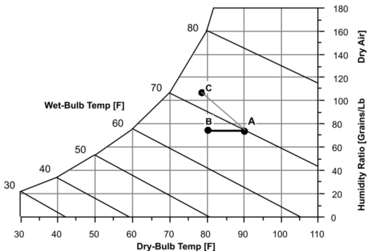
Figure 1.205: Secondary Air Process Indirect Wet Coil Evap Cooler
