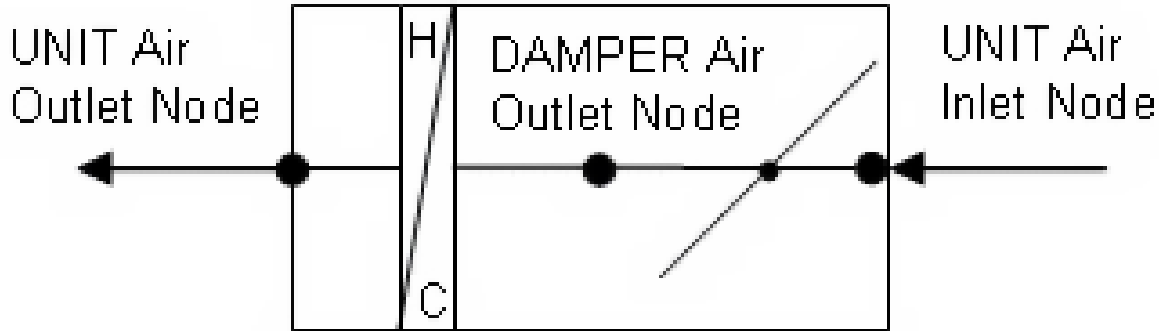
Figure 1.133: Single Duct VAV Heat and Cool Reheat Schematic
