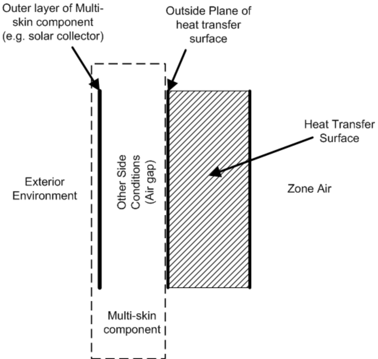
Figure 1.47: Illustration for Other Side Conditions Model
