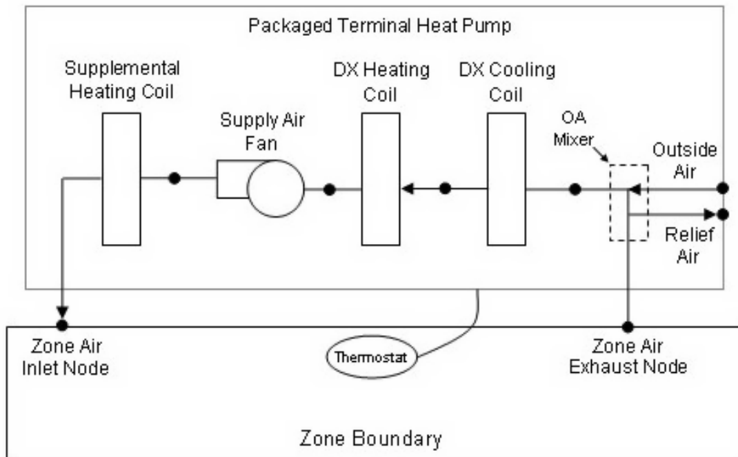
Figure 1.145: Schematic of a packaged terminal heat pump (draw through fan placement)
