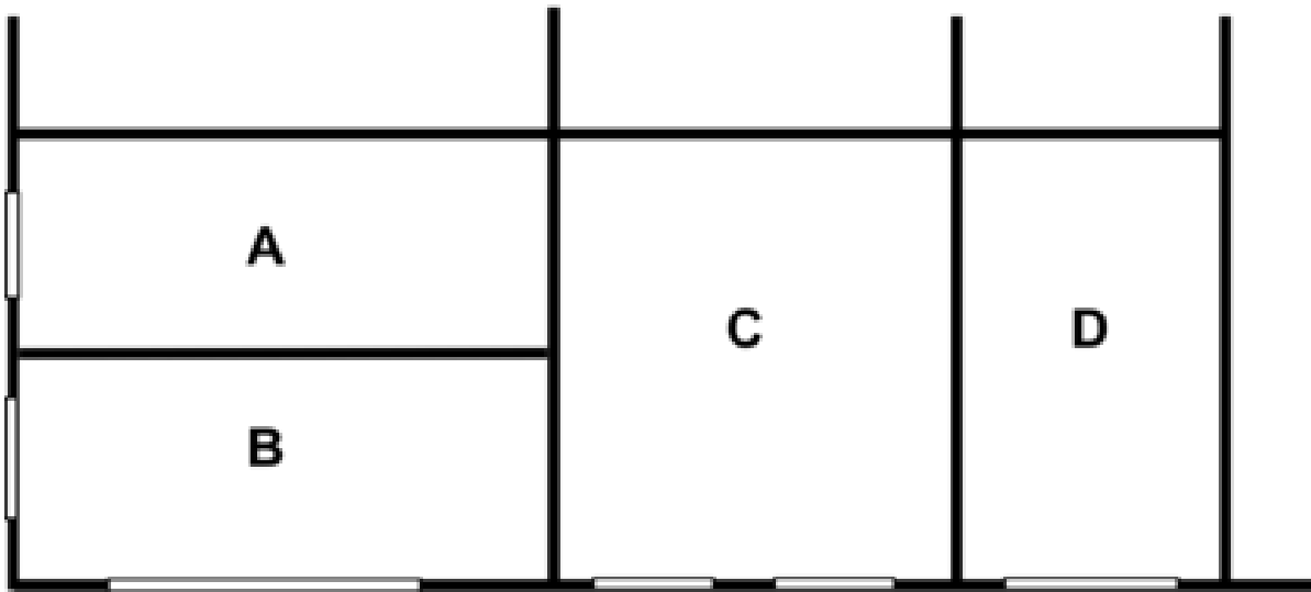
Figure 1.79: Rooms A, B, C and D have different daylighting characteristics. If lumped into a single thermal zone the daylighting calculation will be less accurate because the blockage of direct light by the interior walls between these rooms is modeled with some simplifications (see Interior Obstructions below). To get a good daylighting calculation each room should be input as a separate thermal zone.
