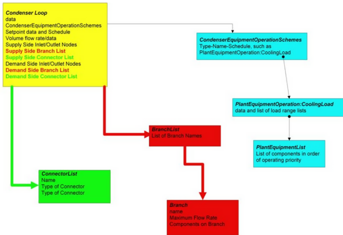
Figure 1.93: Condenser Loop Input Syntax Map
