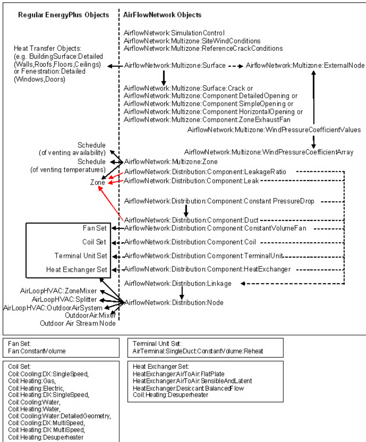
Figure 1.119: Relationships among AirflowNetwork objects (right-hand side) and between AirflowNetwork objects and regular EnergyPlus objects. An arrow from object A to object B means that A references B.
