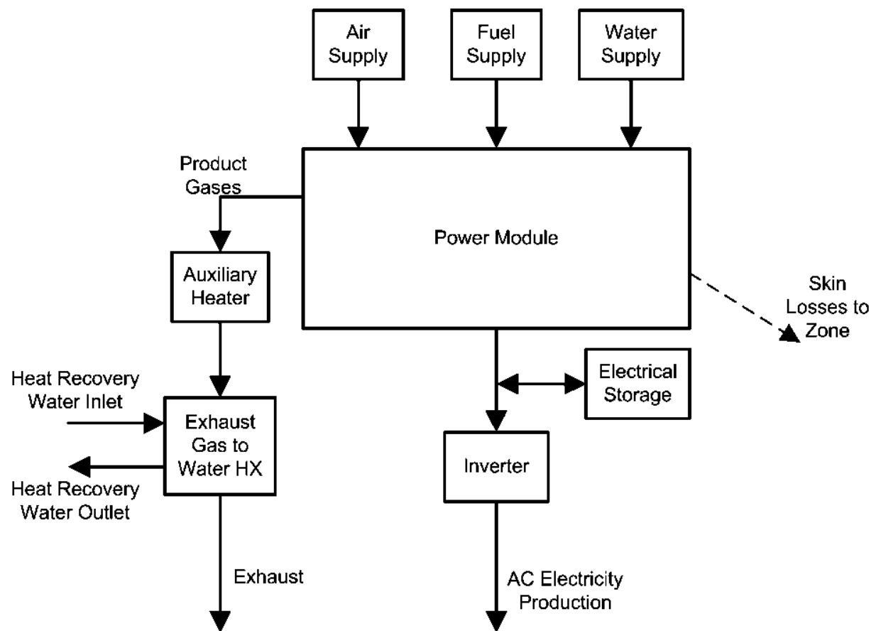
Figure 1.214: Fuel cell subsystems.
