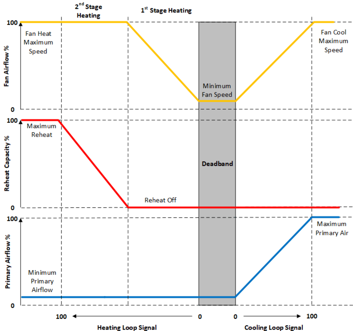
Figure 1.136: Variable Speed Fan with Staged Heat Control
