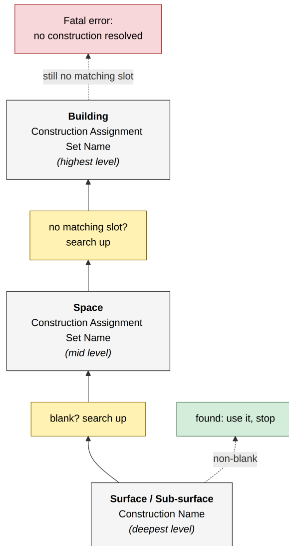
Figure 1.29: Construction resolution order: explicit assignment, then Space-level, then Building-level ConstructionAssignmentSet
