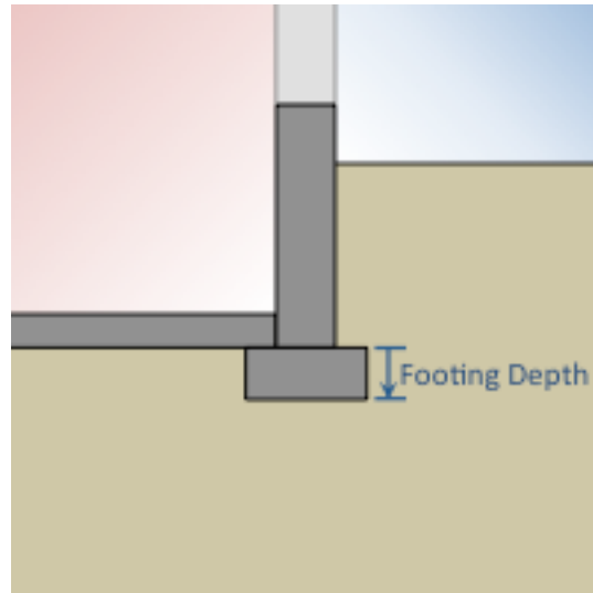
Figure 1.60: Placement of footing
