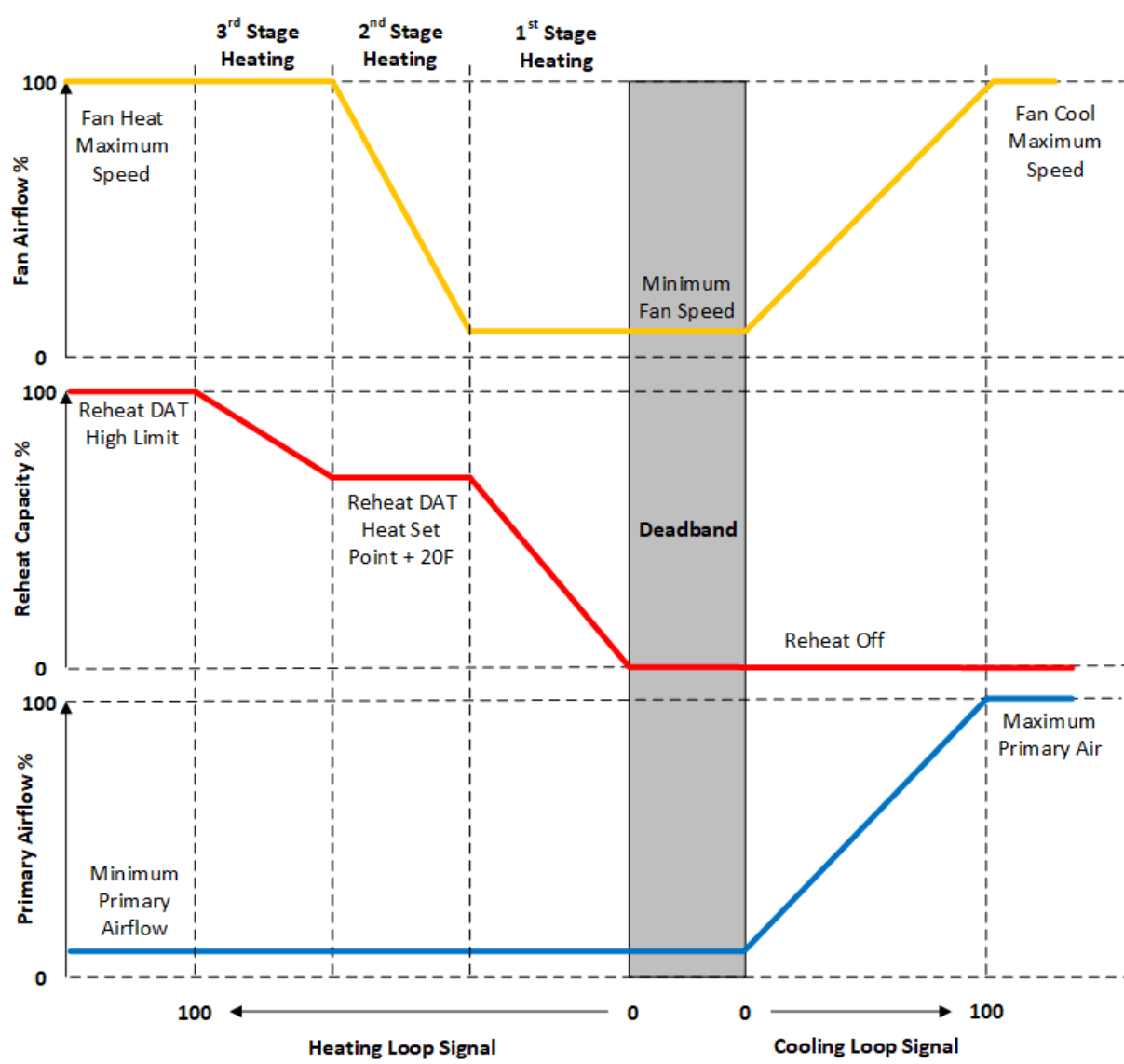
Figure 1.137: Variable Speed Fan with Modulated Heat Control
