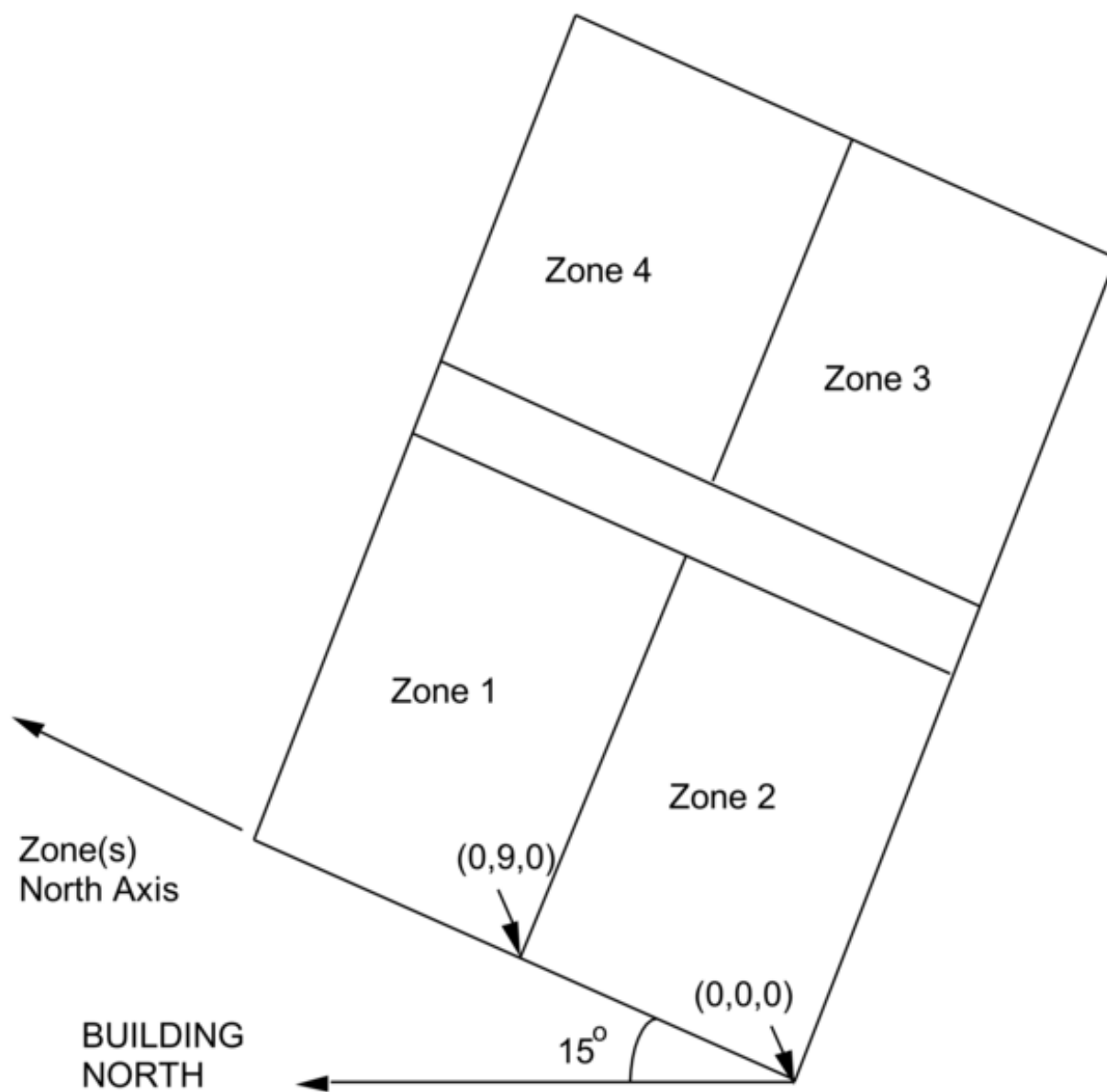
Figure 1.31: Illustration of Zone North Axis and Origins
