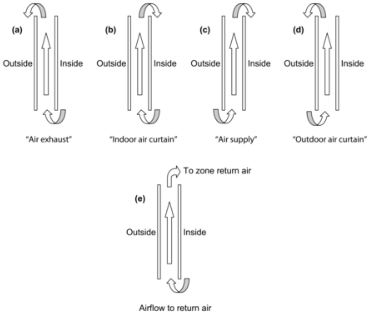
Figure 1.44: Gap airflow configurations for airflow windows. (a) Air exhaust window : Airflow Source = InsideAir, Airflow Destination = OutsideAir; (b) Indoor air curtain window : Airflow Source = InsideAir, Airflow Destination = InsideAir; (c) Air supply window : Airflow Source = OutsideAir, Airflow Destination = InsideAir; (d) Outdoor air curtain window : Airflow Source = OutsideAir, Airflow Destination = OutsideAir; (e) Airflow to Return Air : Airflow Source = InsideAir, Airflow Destination = ReturnAir. Based on “Active facades,” Version no. 1, Belgian Building Research Institute, June 2002.
