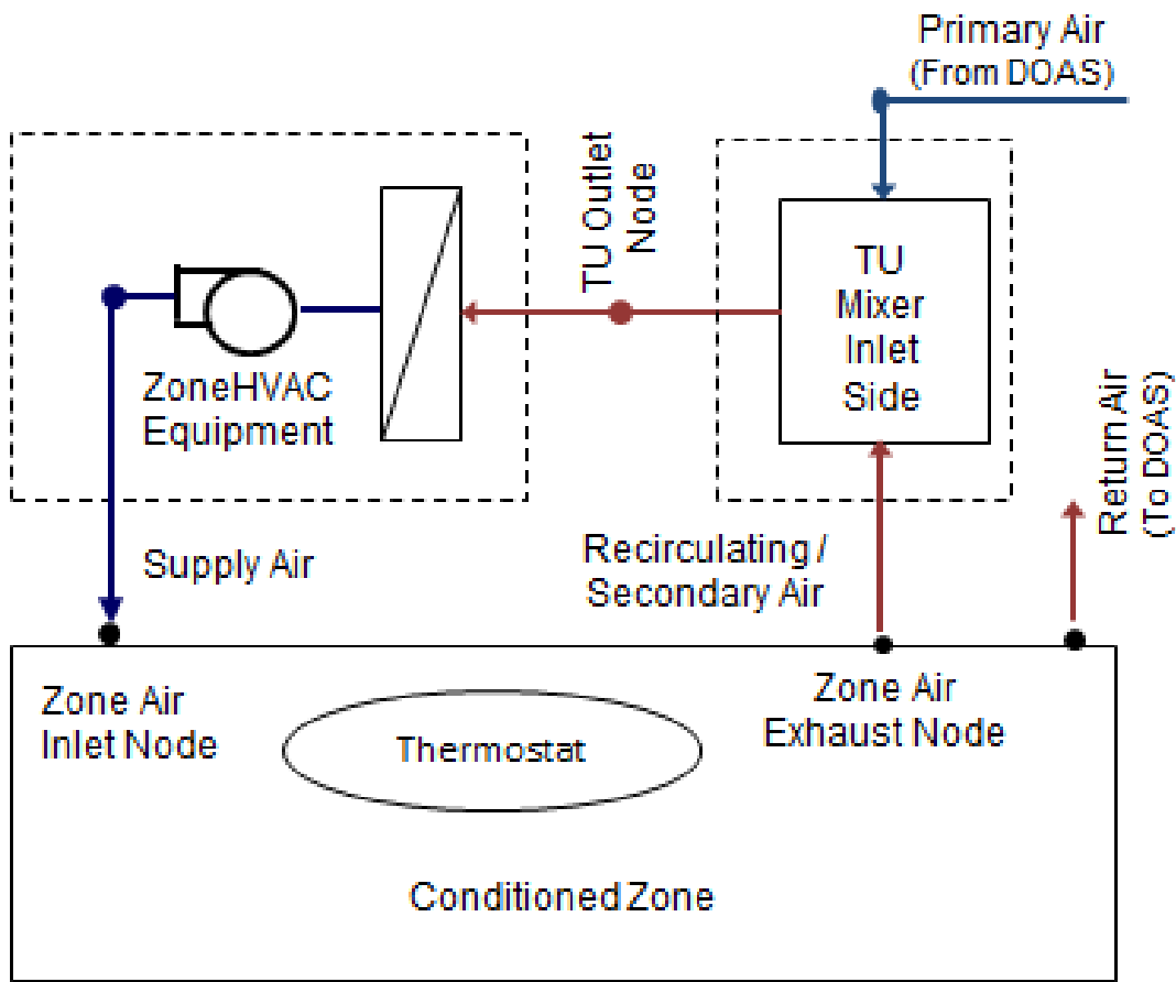
Figure 1.141: Inlet Side Mixer Air Terminal Unit with ZoneHVAC Equipment
