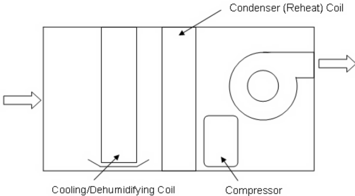
Figure 1.150: Schematic of a mechanical dehumidifier
