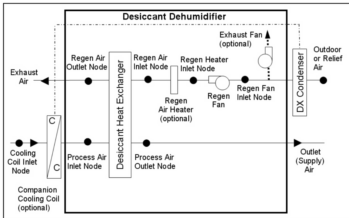
Figure 1.198: Schematic of Dehumidifier:Desiccant:System with Blow Through Regeneration Fan Placement
