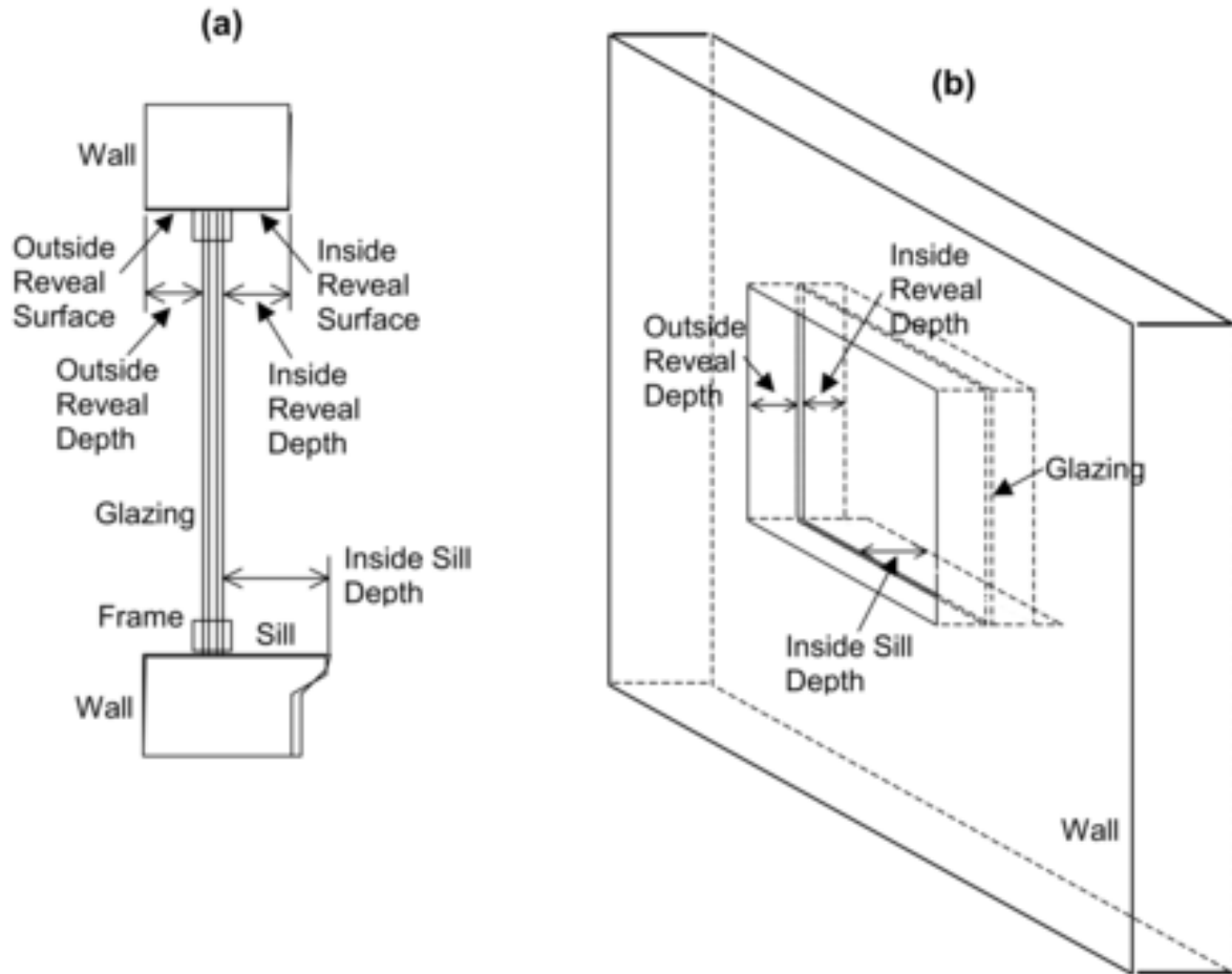
Figure 1.42: (a) Vertical section through a window (with frame) showing outside and inside reveal surfaces and inside sill. (b) Perspective view looking from the outside of a window (without frame) showing reveal surfaces. Note that “Outside Reveal Depth” is not a user input; it is calculated by the program from the window and wall vertices.
