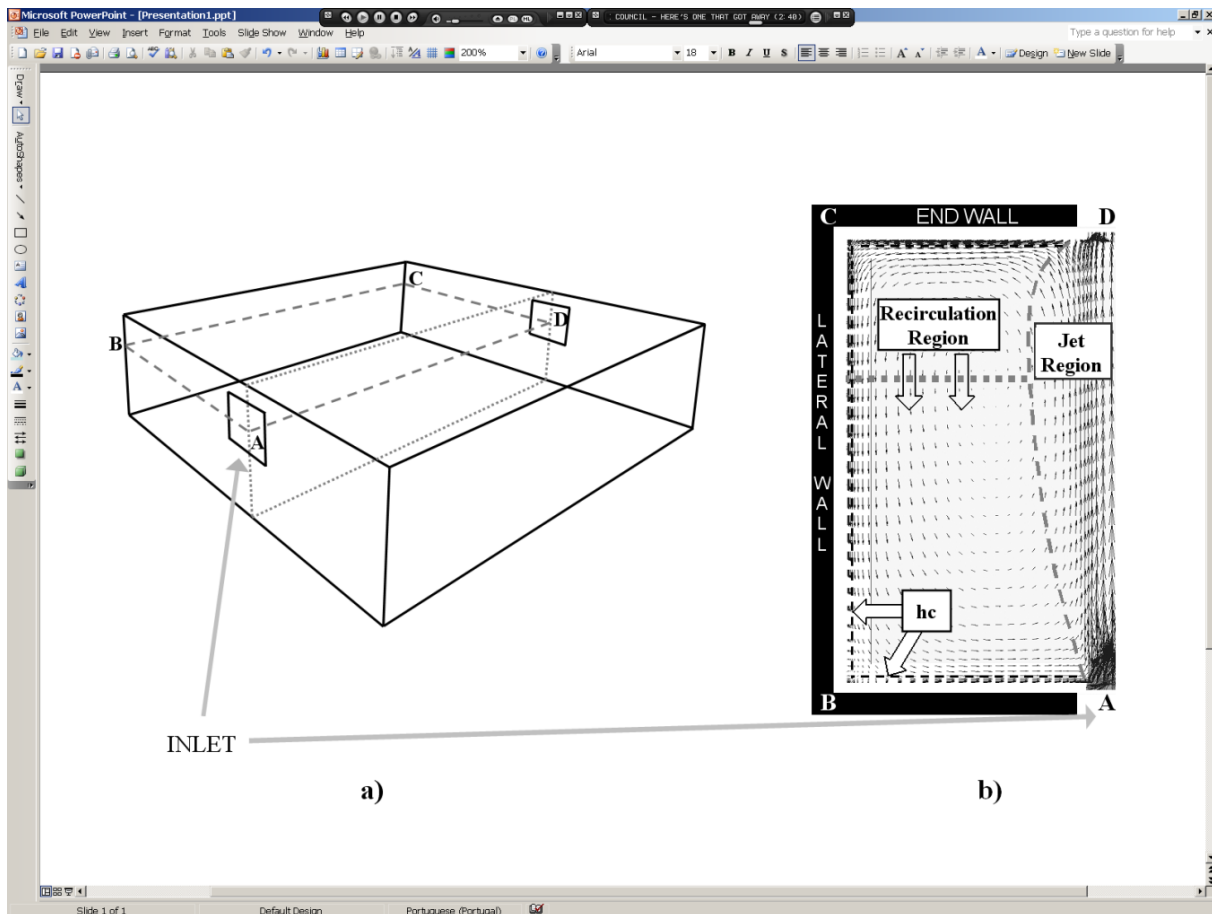
Figure 1.69: Schematic representation of room air geometry a) schematic representation of a room geometry that generates cross ventilation airflow. b) the proposed model distinguishes two regions in the flow: jet and recirculation (shown here in a CFD simulation of one half of a symmetrical room).
