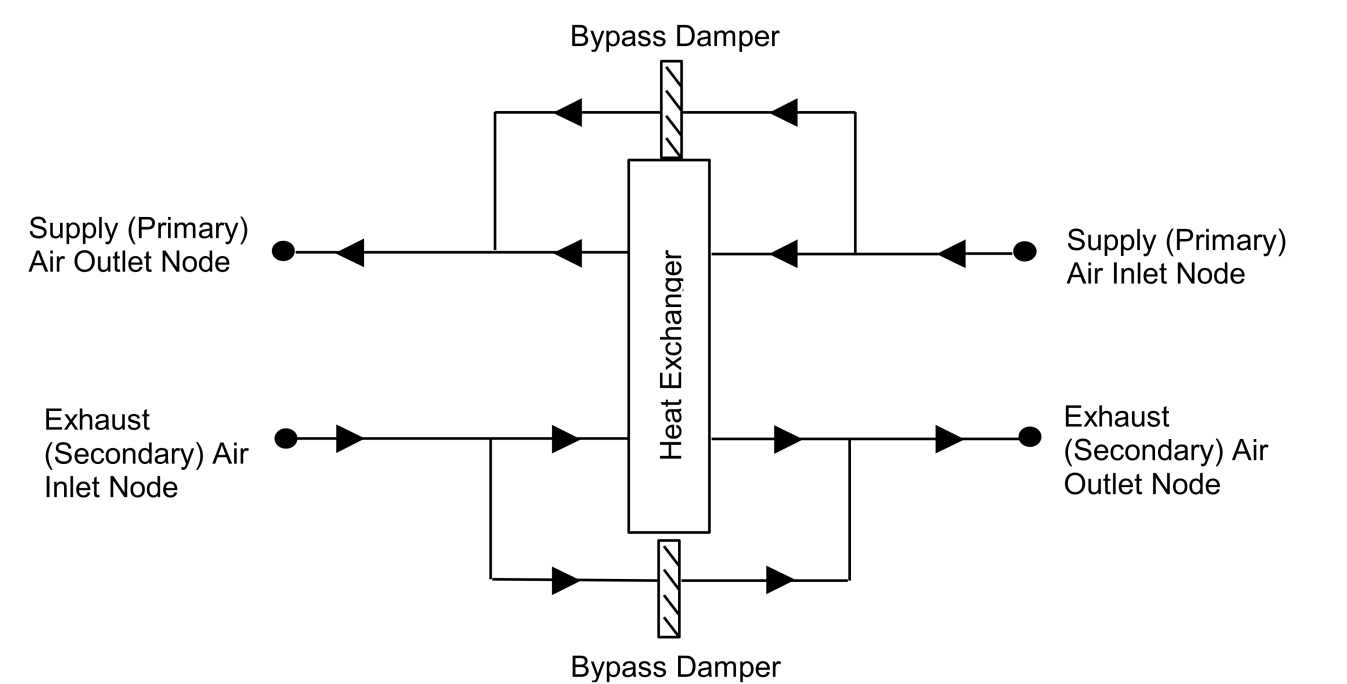
Figure 1.206: Schematic of the Sensible and Latent Air-to-Air Heat Exchanger
