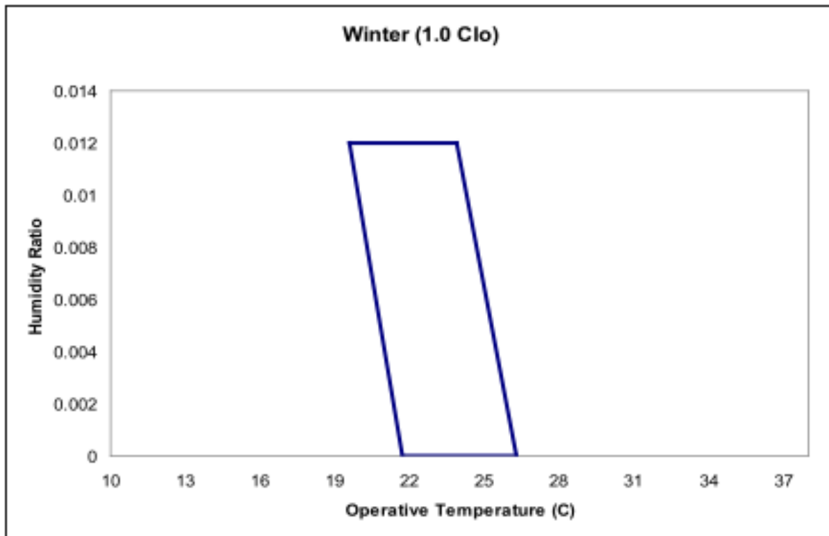
Figure 1.72: Winter Comfort Range
