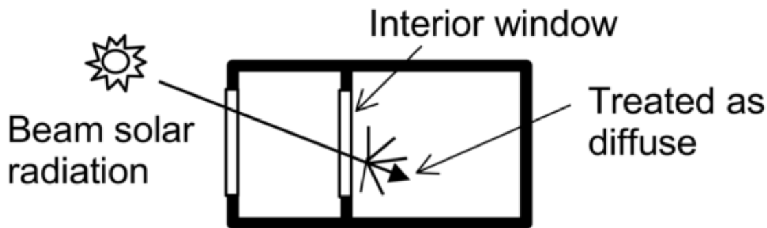
Figure 1.35: Beam solar radiation entering a zone through an interior window is distributed inside the zone as though it were diffuse radiation.
