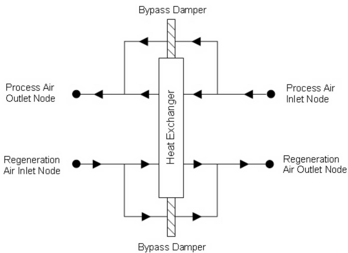
Figure 1.207: Schematic of the Balanced Flow Desiccant Heat Exchanger
