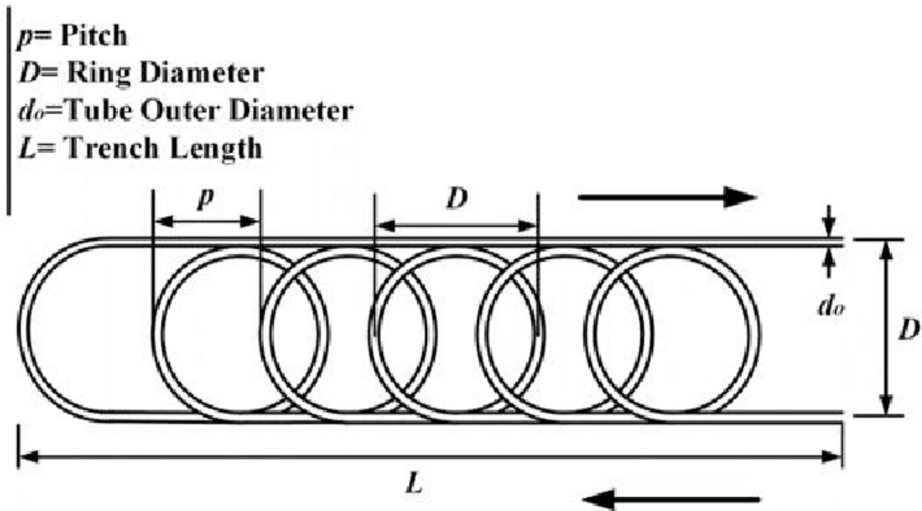
Figure 1.108: Schematic of Slinky HX
