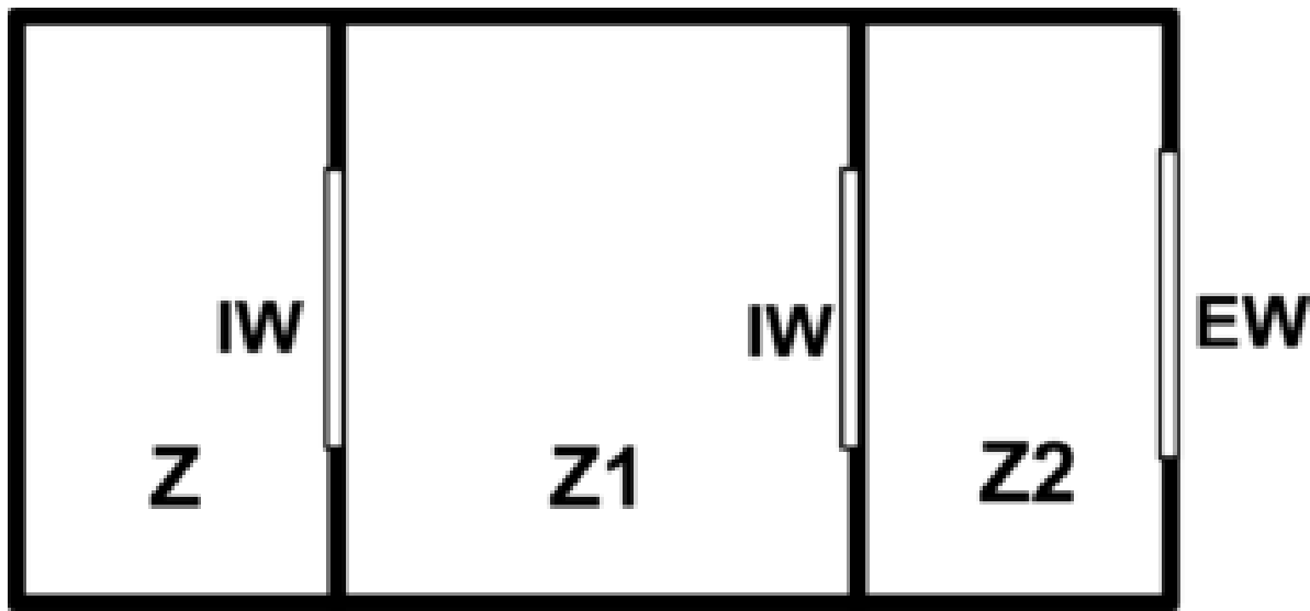
Figure 1.84: Configuration in which daylighting of zone Z through its interior window cannot be calculated with EnergyPlus. IW = interior window, EW = exterior window.
