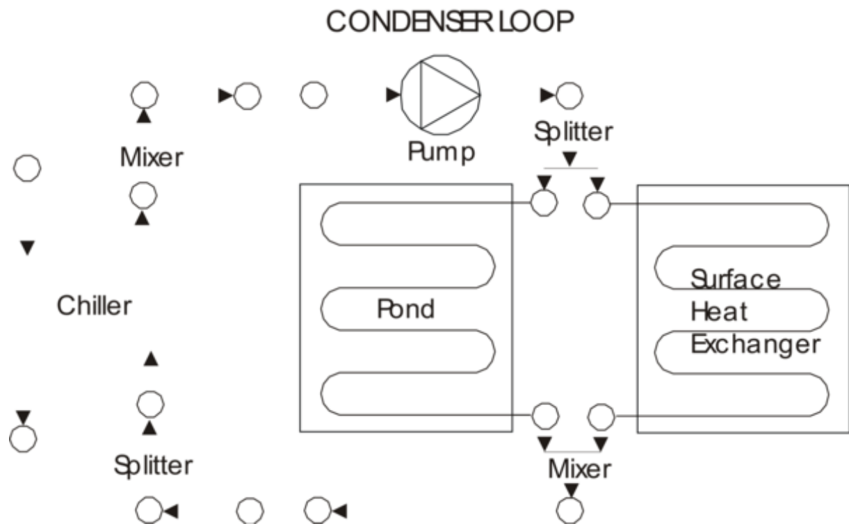
Figure 1.110: Pond Ground Heat Exchanger with other heat exchangers on condenser loop
