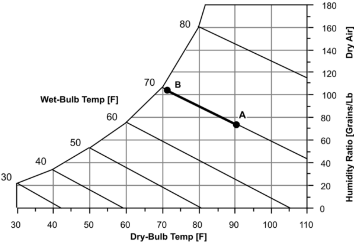
Figure 1.201: Psychrometric Chart – Constant Wet-Bulb Temperature
