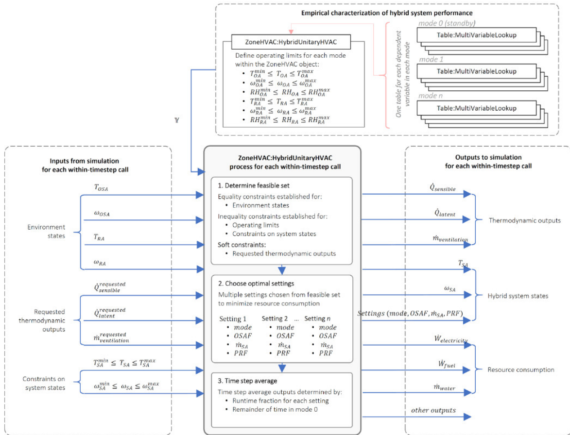
Figure 1.153: Schematic explanation of the architecture and function of ZoneHVAC:HybridUnitaryHVAC
