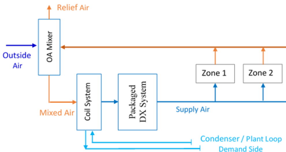
Figure 1.181: Water Side Economizer Coil System Upstream of Packaged DX System
