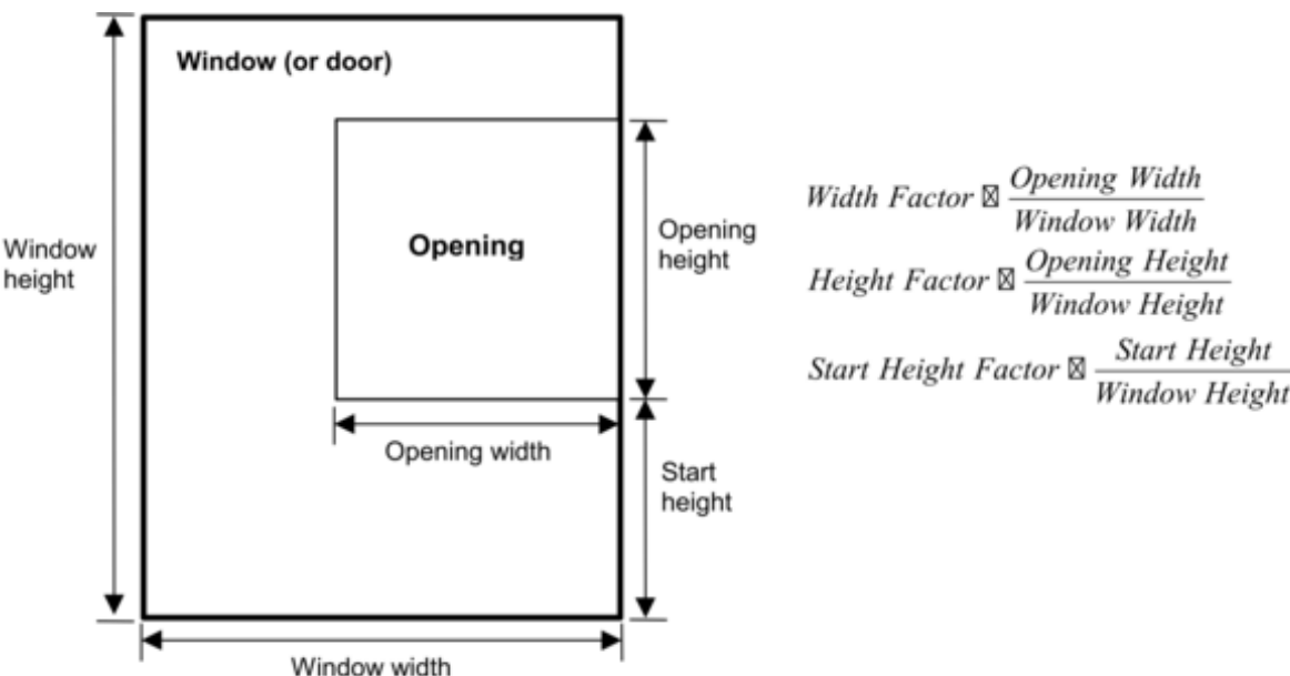
Figure 1.125: Window (or door) showing geometrical factors associated with an opening through which air flows.
