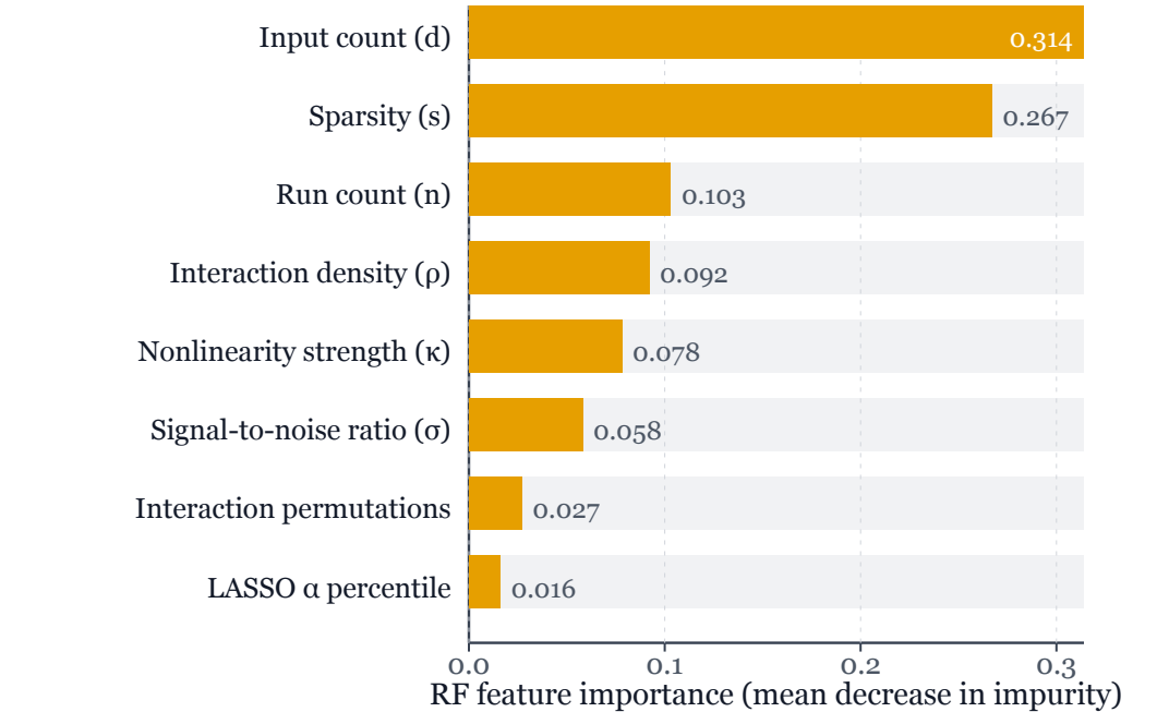
Runtime model: RF feature importance
