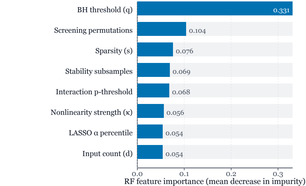
Quality model: RF feature importance
