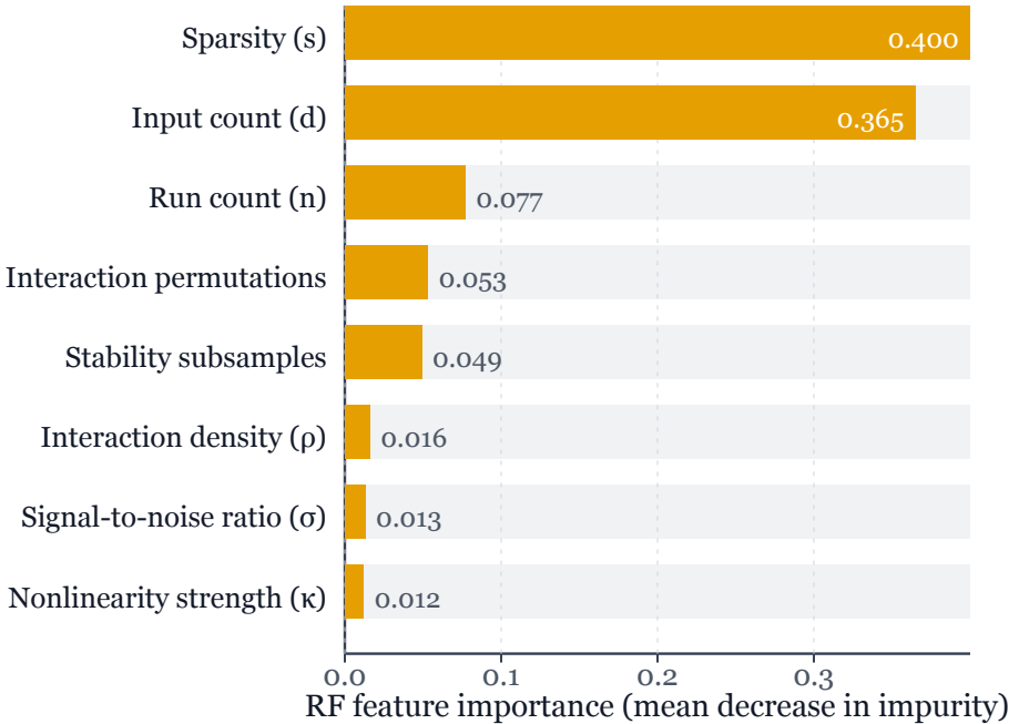
Runtime model: RF feature importance
