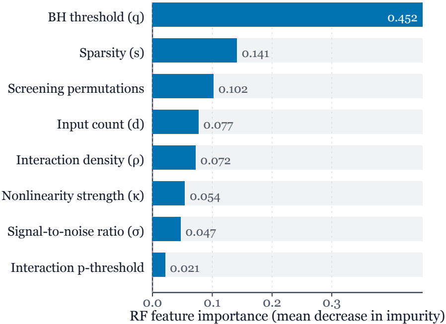
Quality model: RF feature importance
