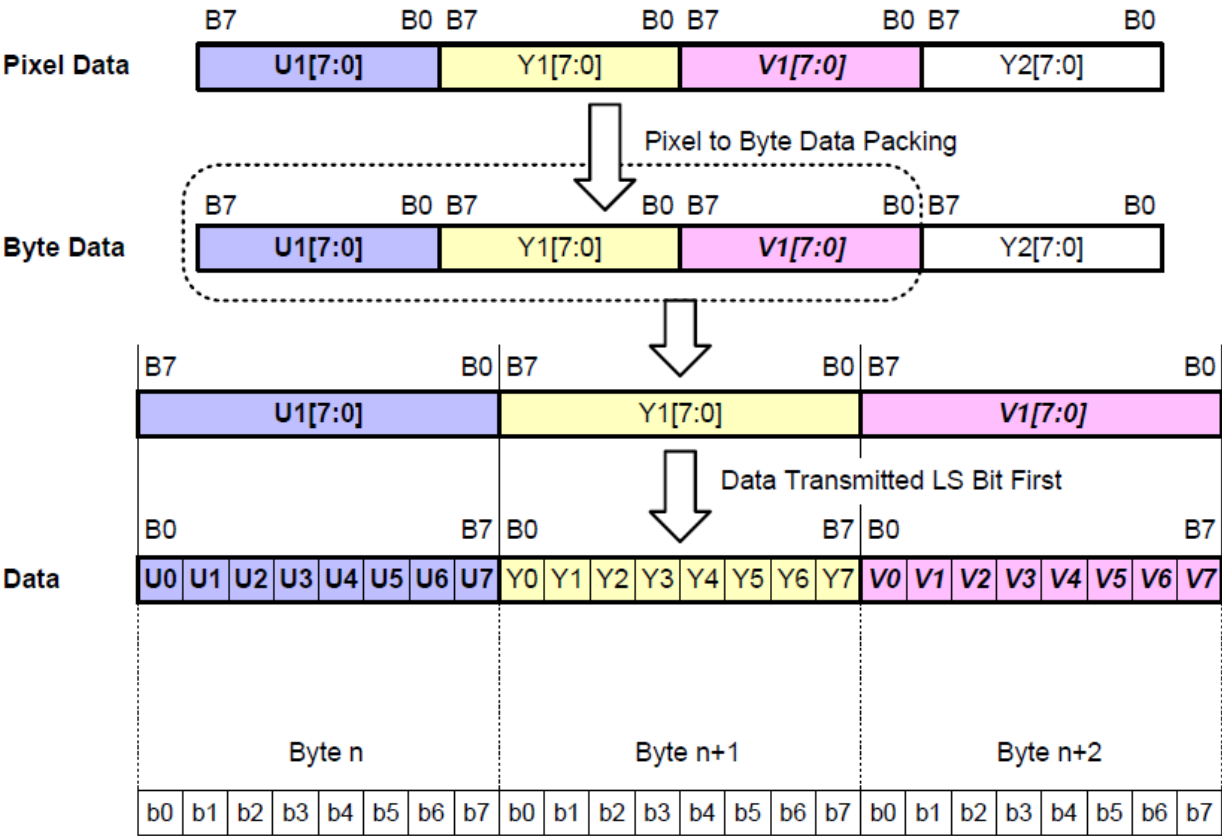
Diagram 19.24: YUV422-8bit data packet transmission mapping
