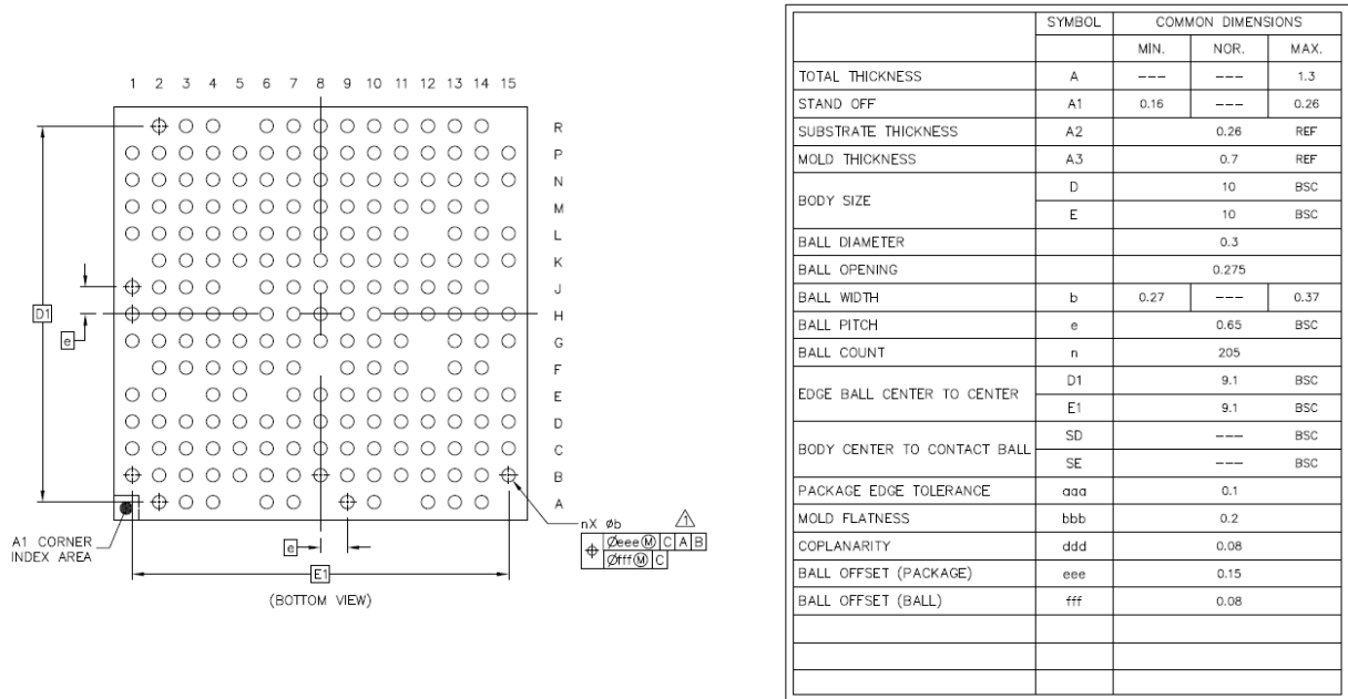
Diagram 3.2: Package appearance dimensions, bottom view
