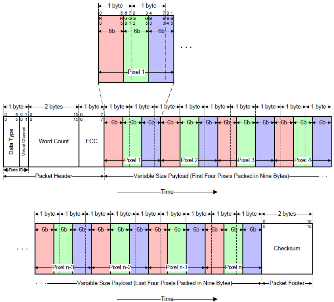
Diagram 19.53: RGB 18-bit format (Data type = 0x1E)
