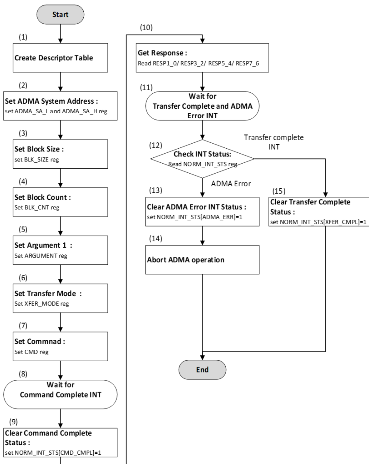
Diagram 21.41: ADMA data transfer mode program
