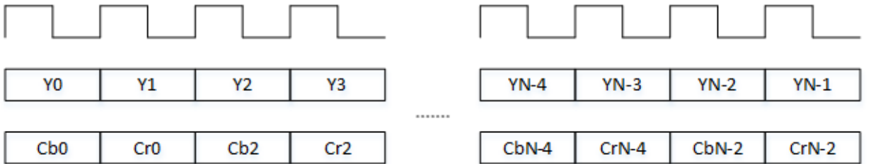
Diagram 19.8: BT.601 Y/C separated 16bit mode
