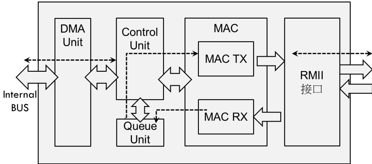
Diagram 18.1: eMAC overall data flow
