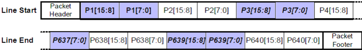
Diagram 19.35: RAW16 data transfer sequence
