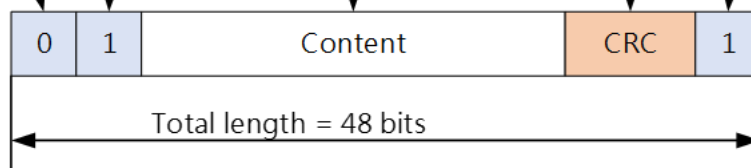
Diagram 21.22: eMMC/SD/SDIO command format
