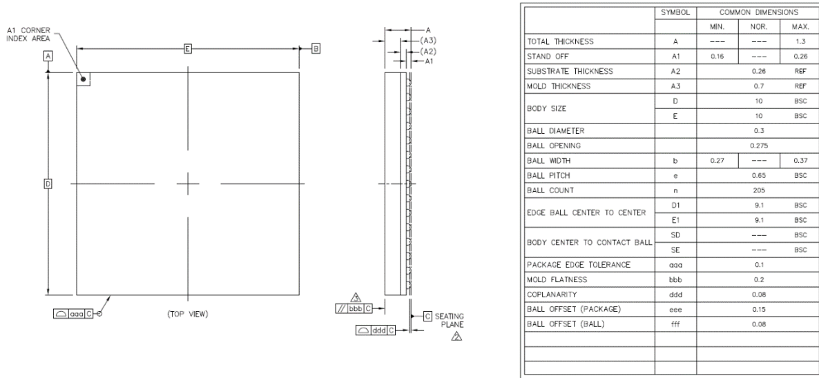
Diagram 3.1: Package appearance dimensions, top view
