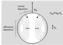
"Fig. 1. Internal circulation (Hill's vortex) inside a rising gas bubble."
