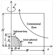
"Fig. 3. Schematic of the computational domain for transient drop deformation after abrupt inception of a uniaxial extensional flow. The flow is axisymmetric with respect to the y axis and the domain lies in the meridional plane. The drop size is exaggerated; the actual domain size has H = W = 10R_0 ."
