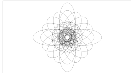
Figure 3: View from top (Z-axis) of hopf-fibration
