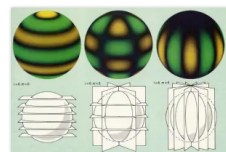
"3 Surface Harmonics at l=6 m=0, l=6 m=3 and l=6 m=6."
