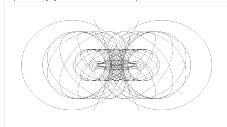
Figure 1: Profile of hopf-fibration from sides (X-axis/Y-axis)
