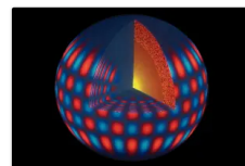
"Cut-away view of the Sun showing p and g modes with an accompanying l vs. v power spectrum"
