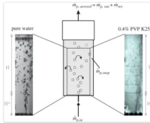
"Fig. 3. Mass balance of the bubble column (middle) and pictures taken with a high-speed camera for pure water (left) and for a PVP-water solution (right)."
